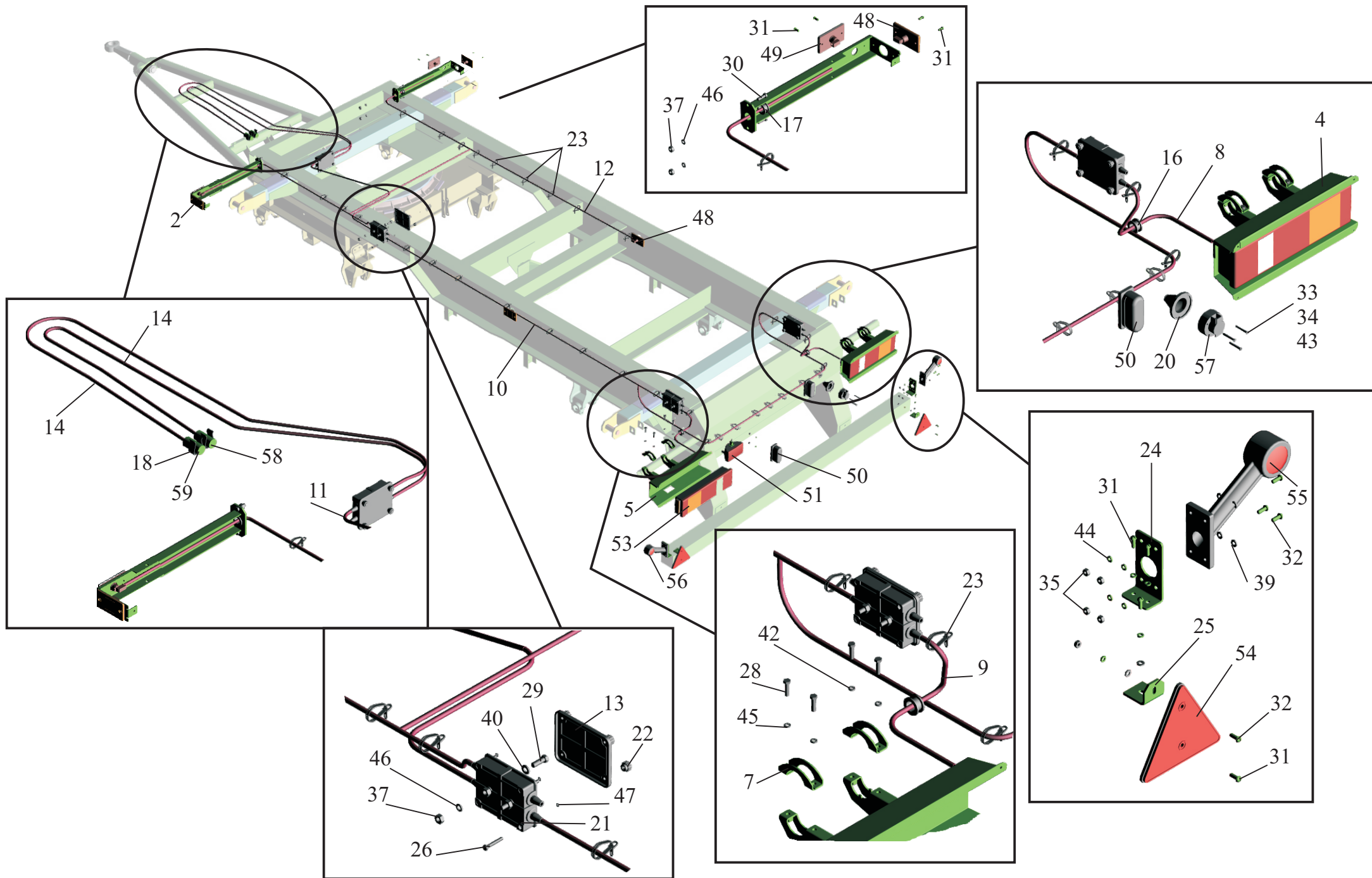
Fig. 42 Installation of an electric equipment 8571-3700002, 8571-3700002-700
