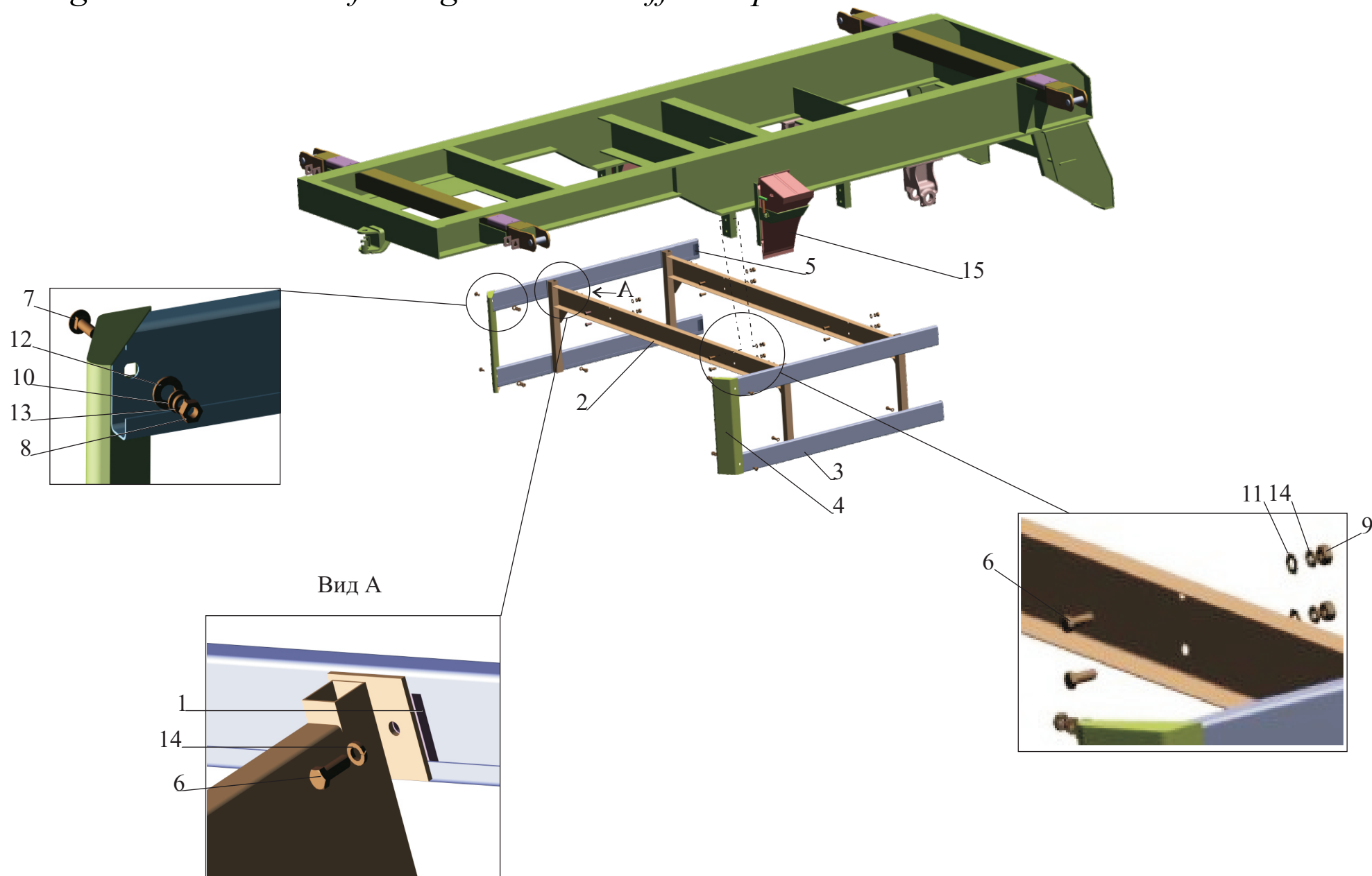
Fig. 7 Installation of side guard and buffer stop .
