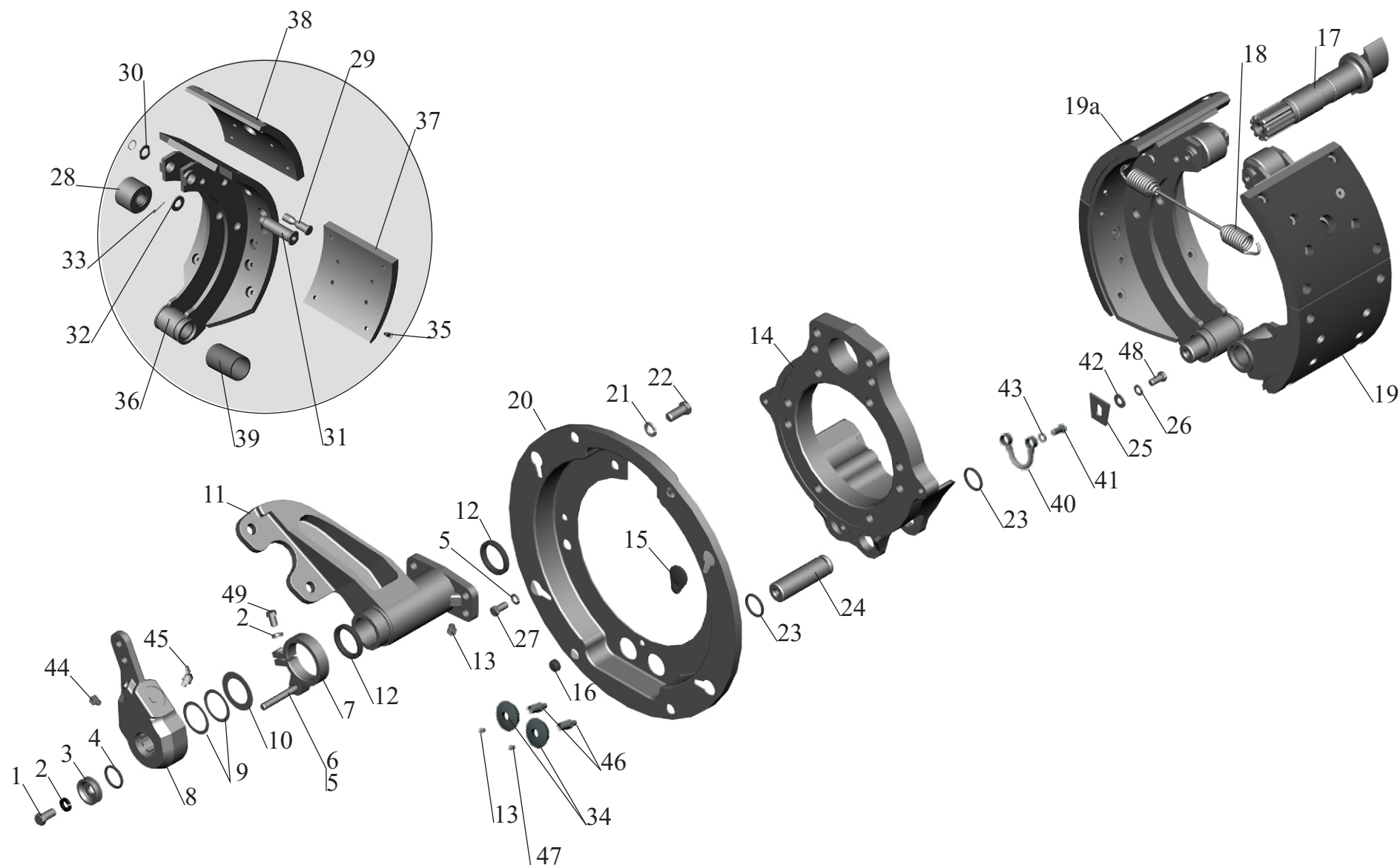
Fig. 21 Brake mechanism front wheels 152-3501004 (152-3501005)
