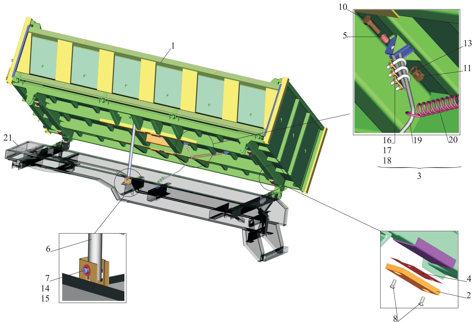
Fig. 43 Installation platform 8561-8500002-020, 8561-8500002-030 Frame 8561-2801010.
