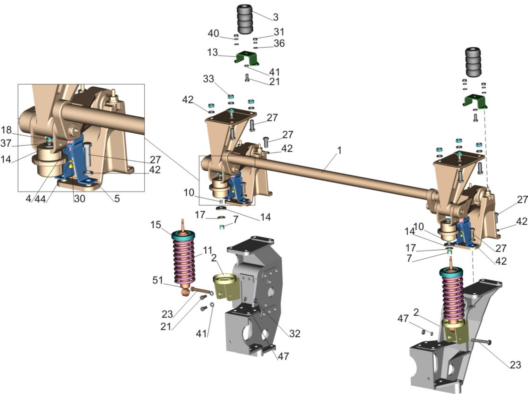
Fig. 214 Front springing 6430-5001700-10
