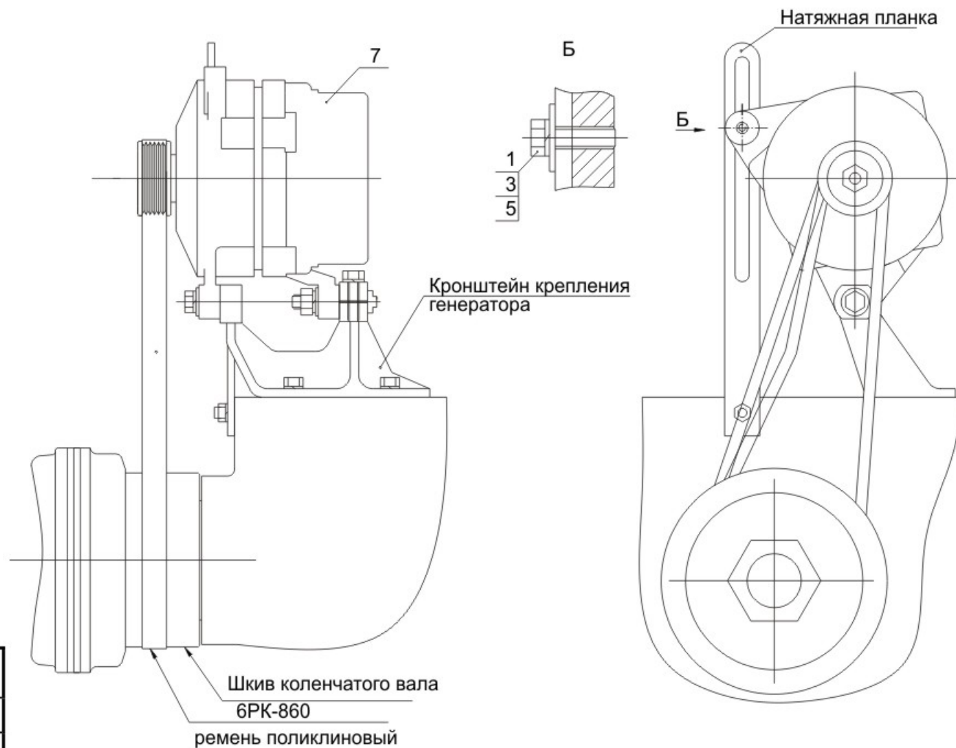
Fig. 190 Installation generator 642208-3700011
