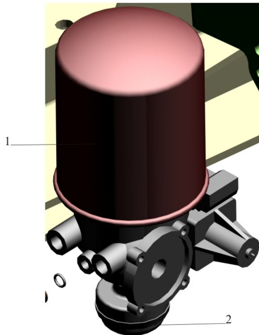
Fig. 168 Air dehumidifier with muffler 630300-3512004
