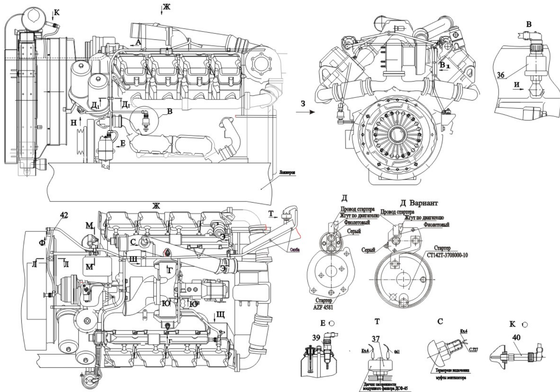
Fig.189 Electric equipment installation on the engine (page 1)
