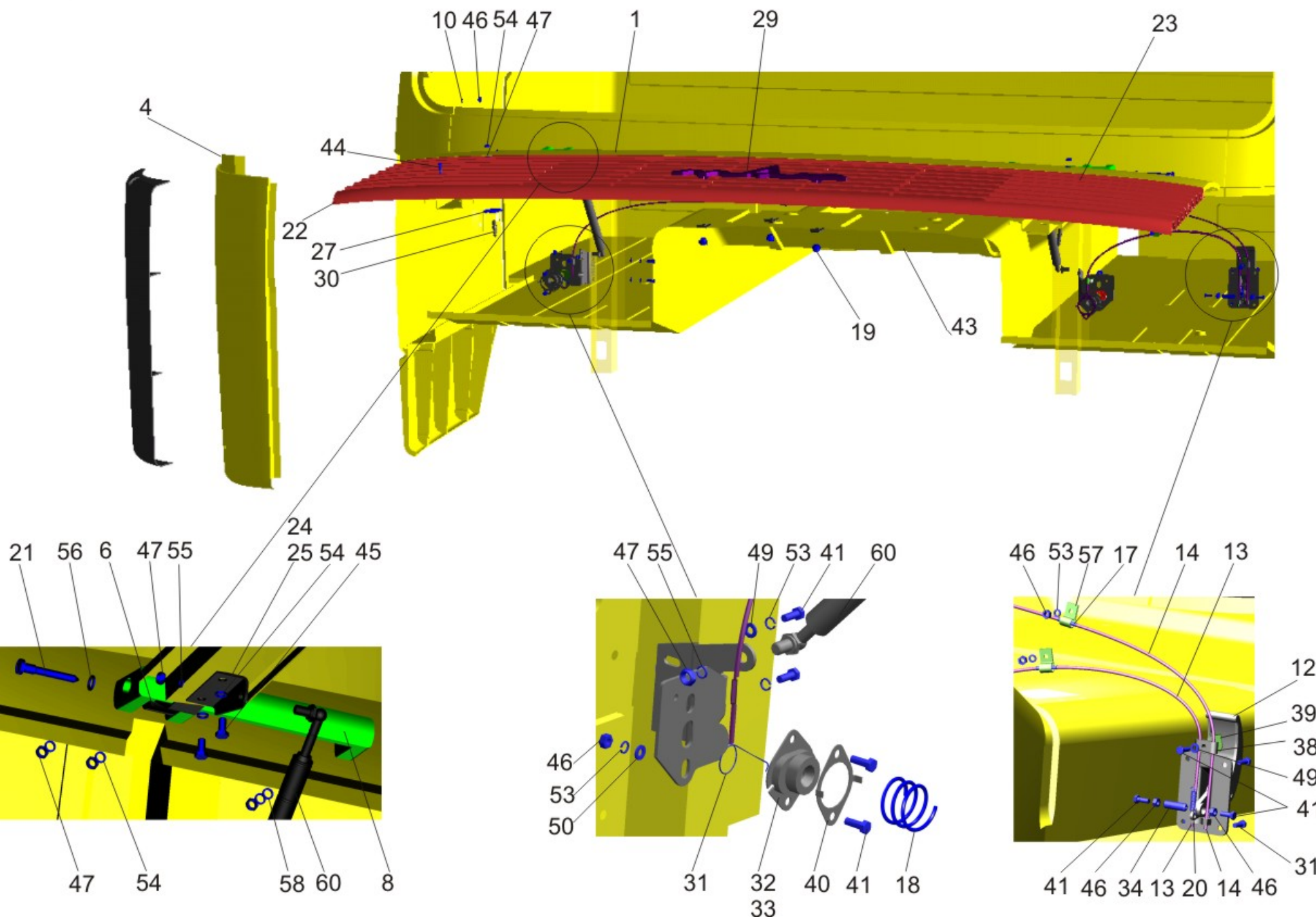
Fig. 232 Installation of facing 6430-8400018
