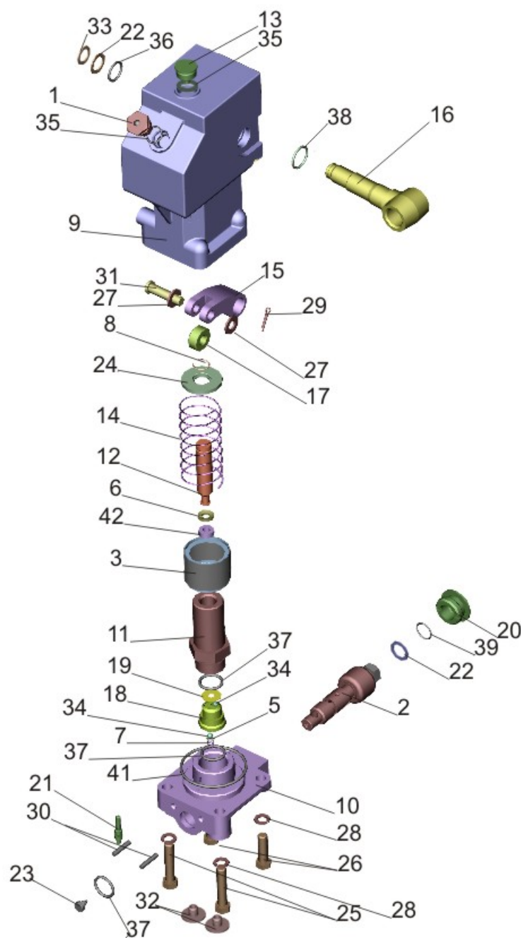
Fig. 240 Pump cab tilting mechanism 6430-5004010
