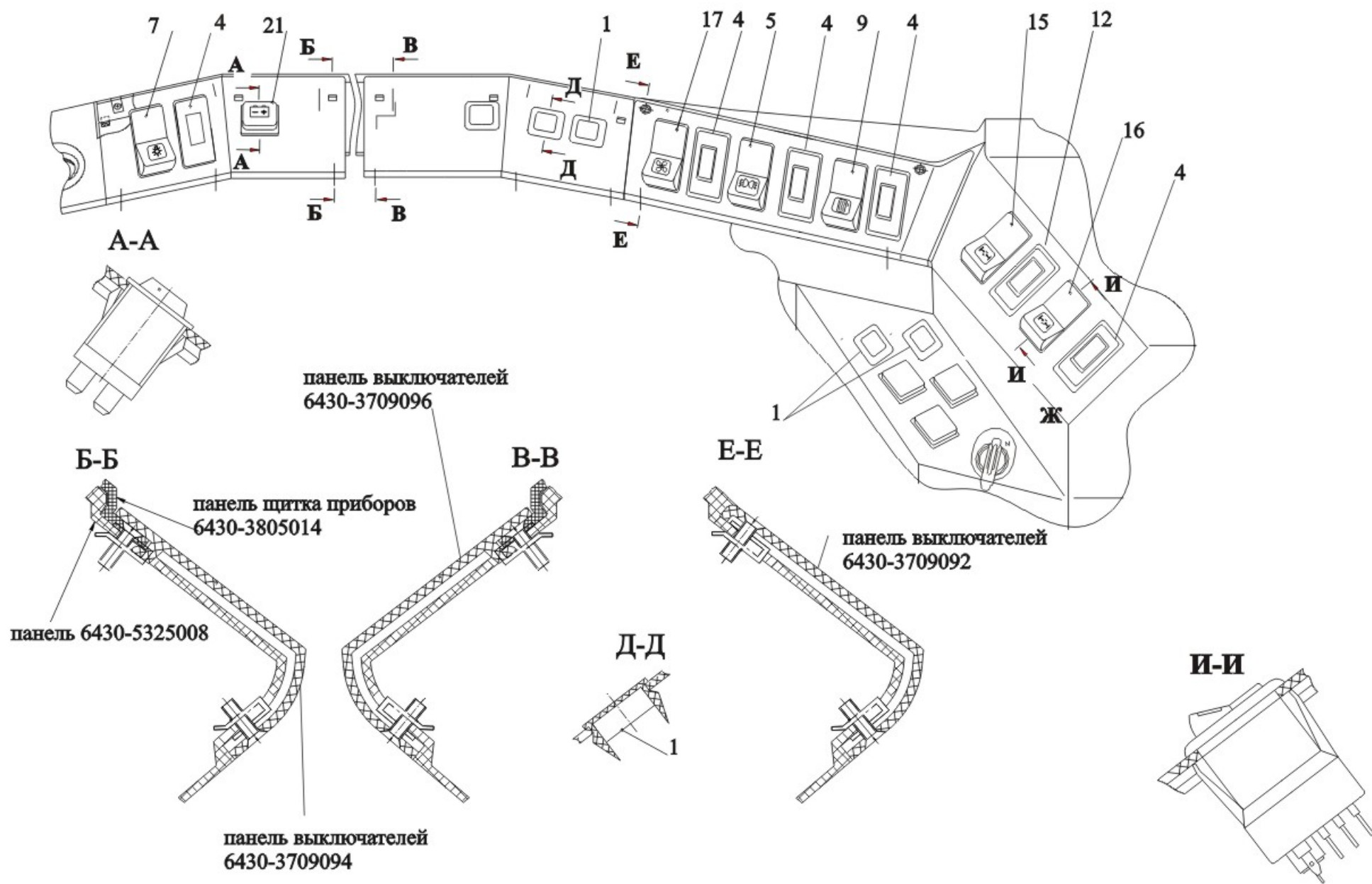
Fig. 180 Installation of switches 650105-3700018
