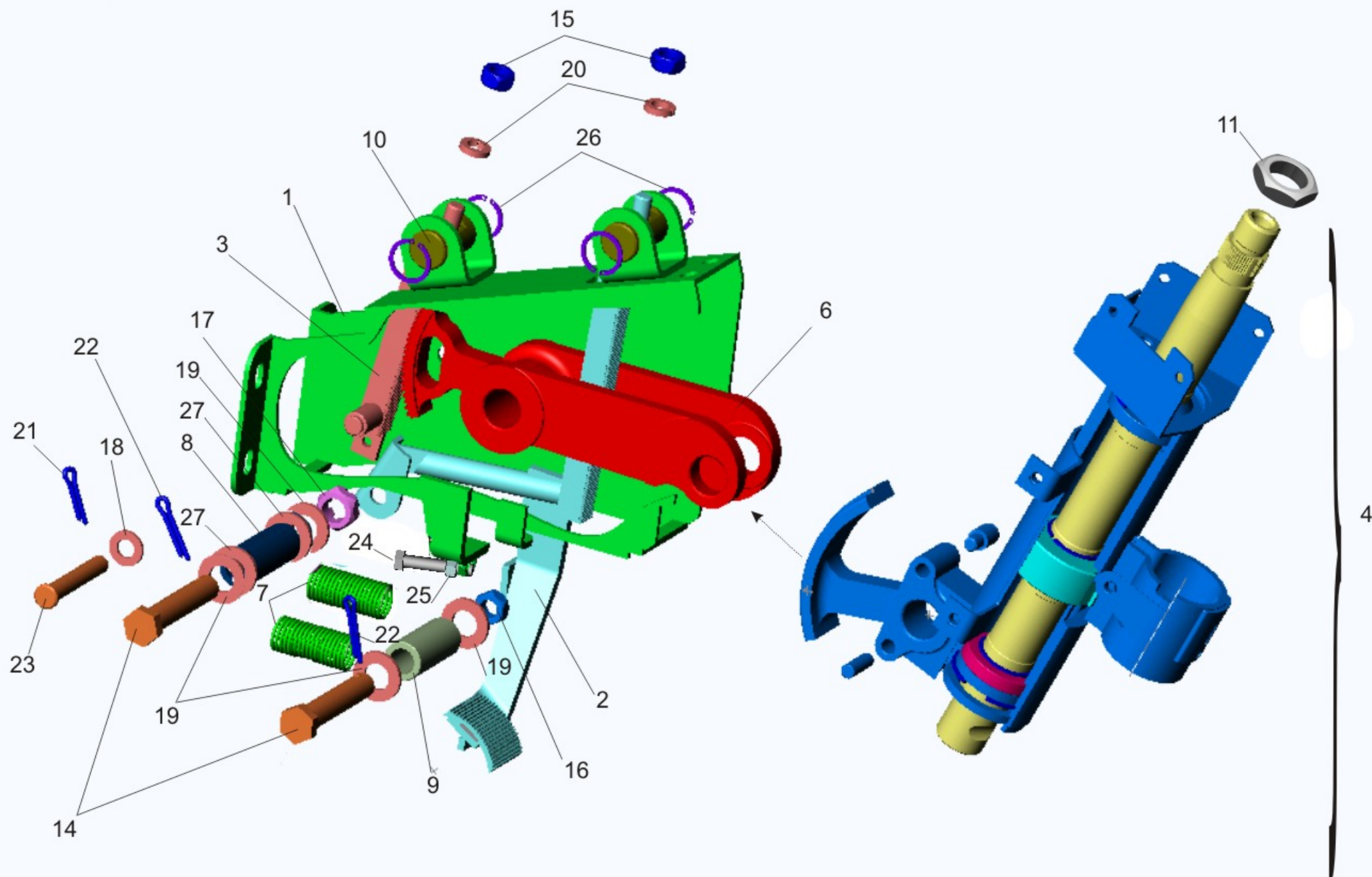
Fig. 144 Arm with a column 5440-3403008
