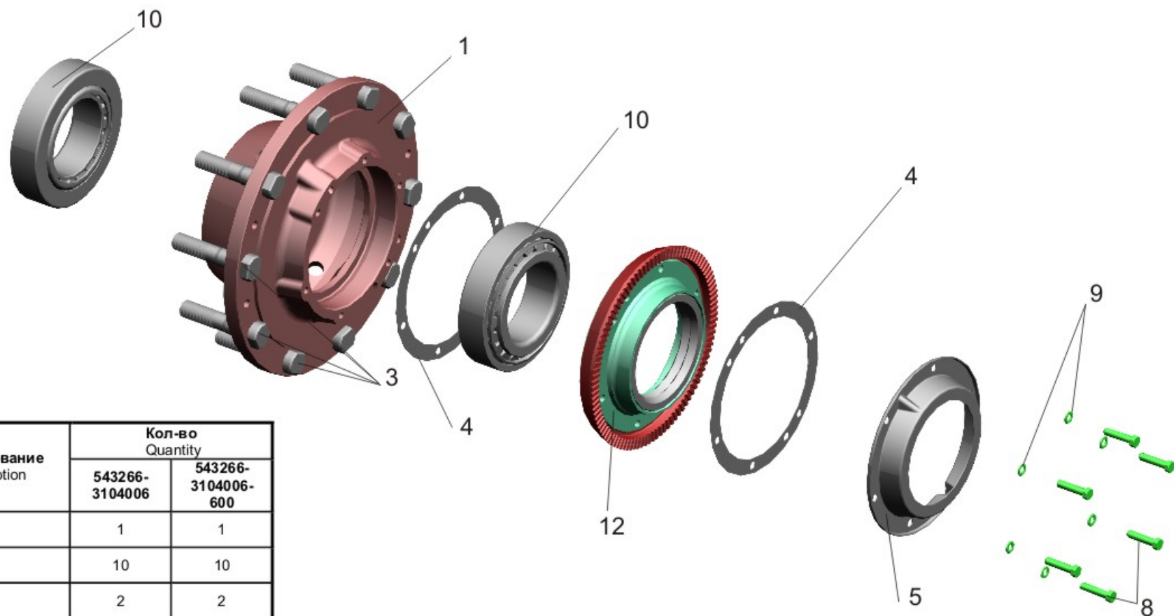
Fig. 58 Rear axle hub 543266-3104006, 543266-3104006-600
