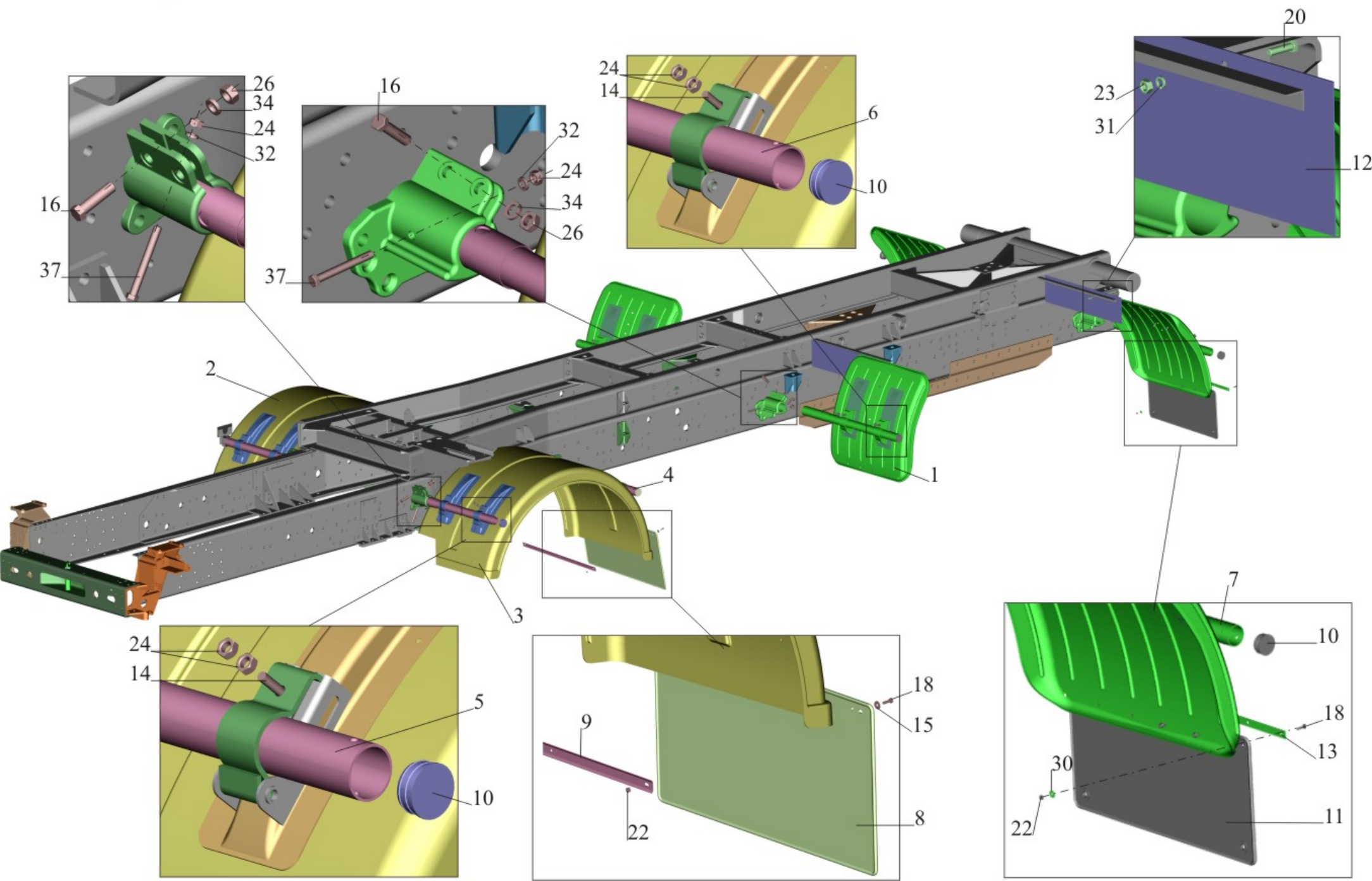
Fig. 282 Installation fenders 651608-8500048-020
