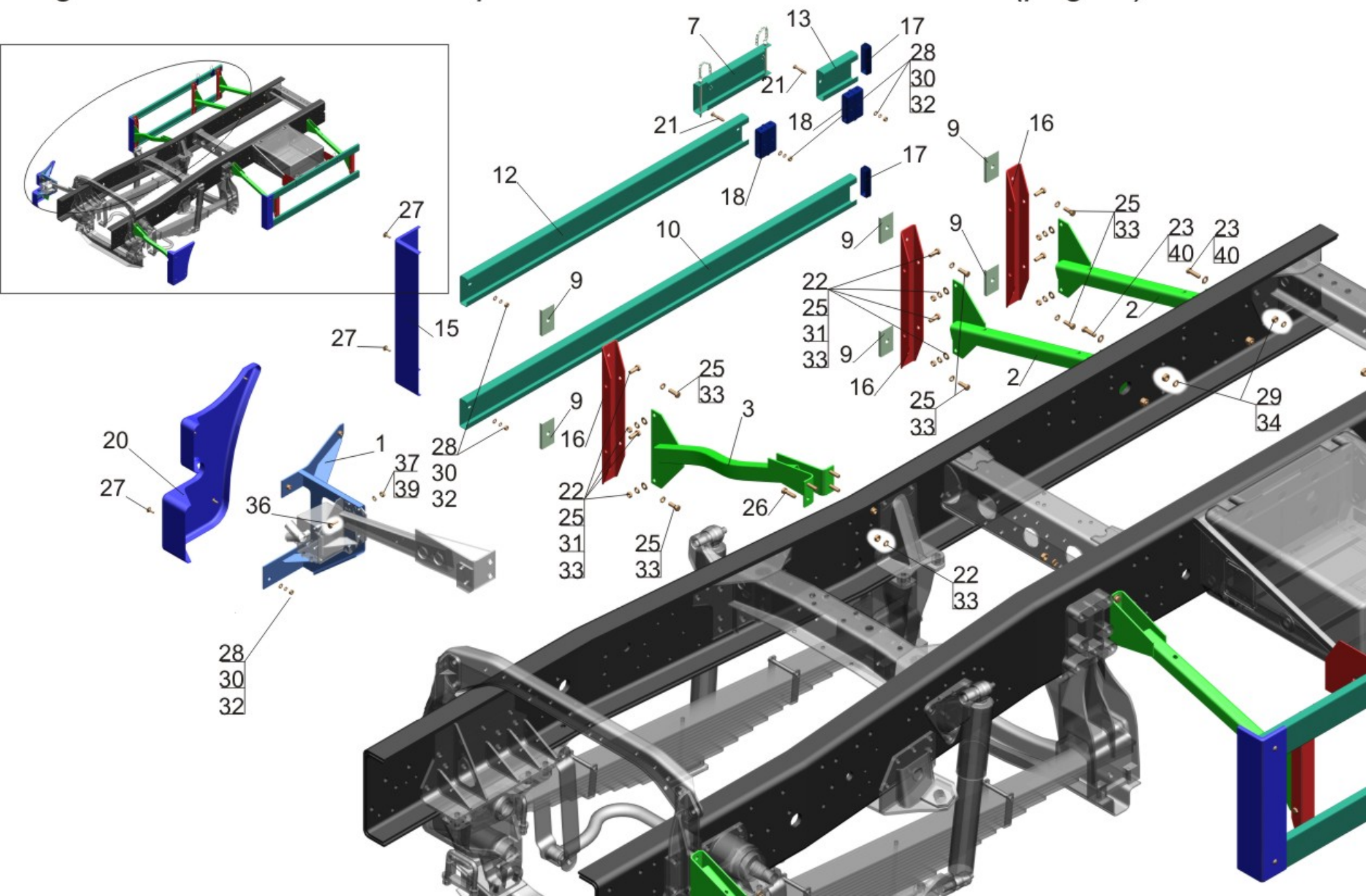
Fig.91 Installation of lateral protection 651608-2800040-010 (page 1)
