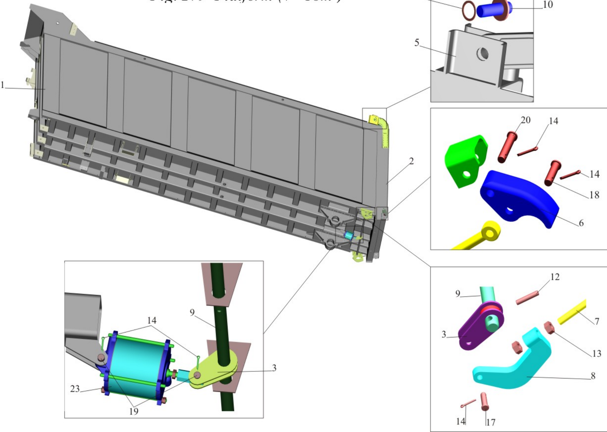
Fig. 279 Platform ( V=18m^3 )
