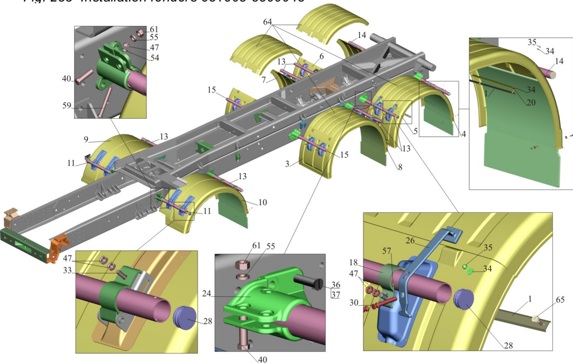
Fig. 283 Installation fenders 651608-8500048
