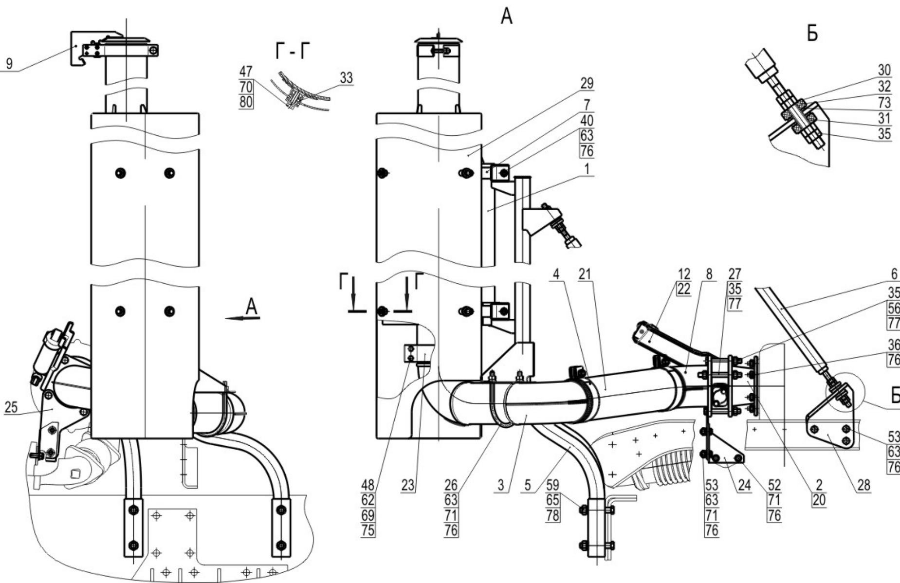
Fig. 26 Installing of gases exhaust system 651608-1200001
