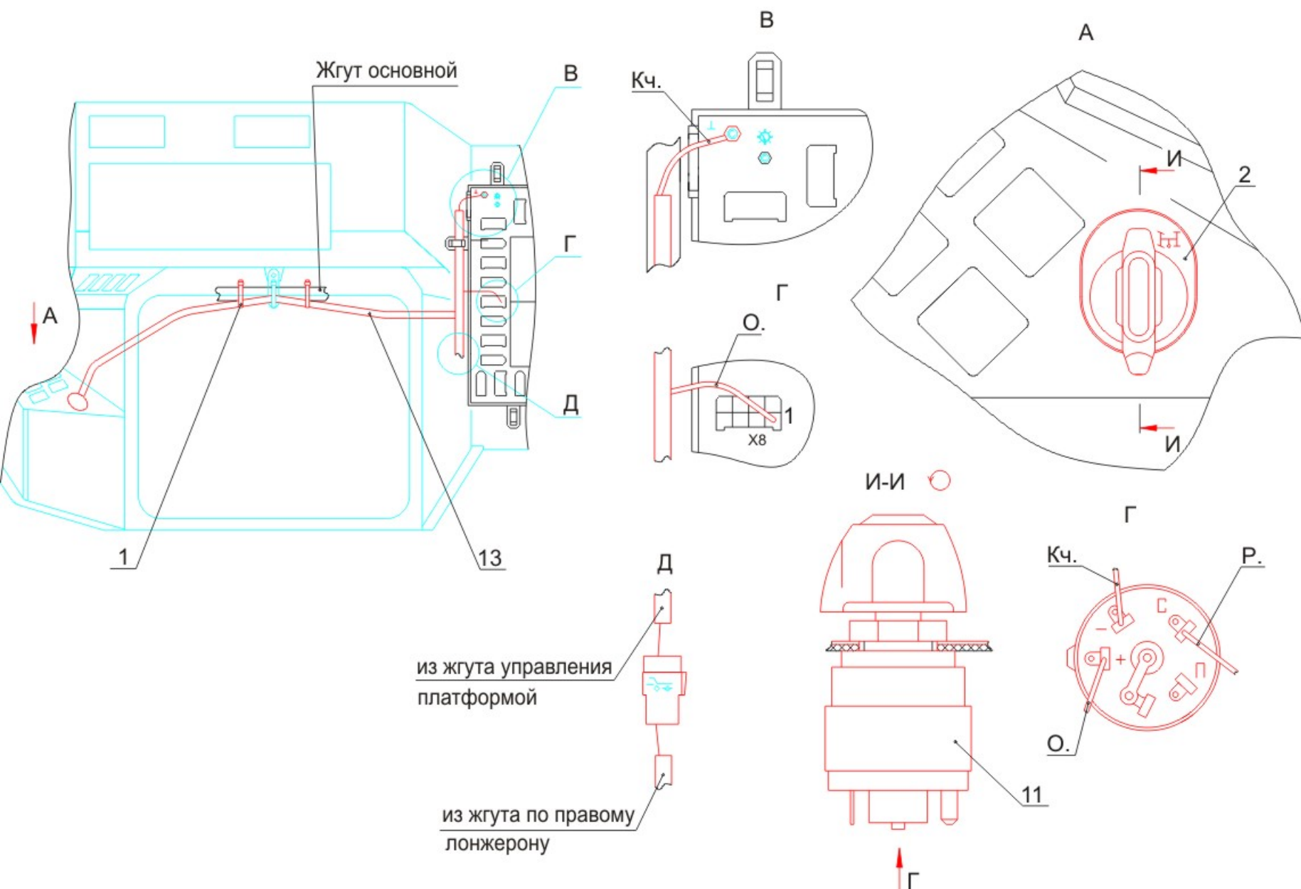
Fig.195 Installation of an electric equipment for inclusion of selection of capacity
