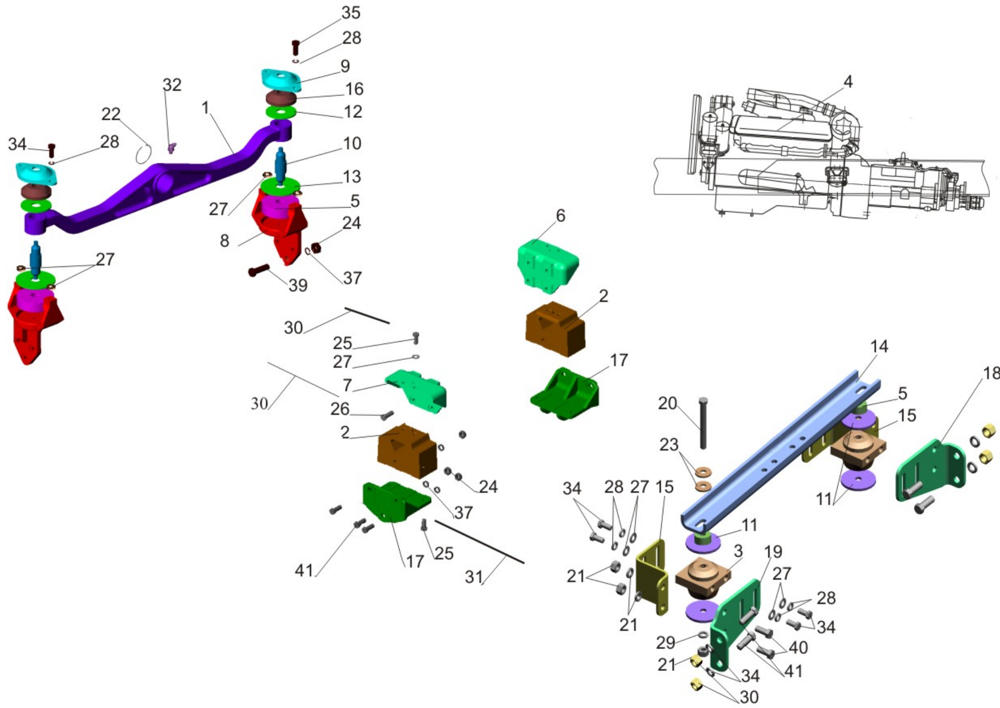
Fig. 4 Mounting of engine 651608-1001002, (-600), (-700)
