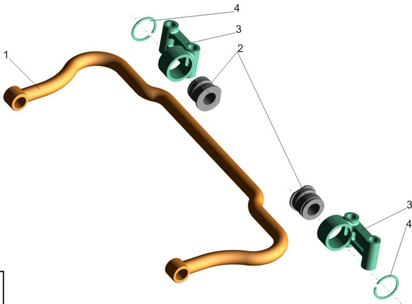
Fig. 94 Stabilizer shaft with brackets 631705-2906006
