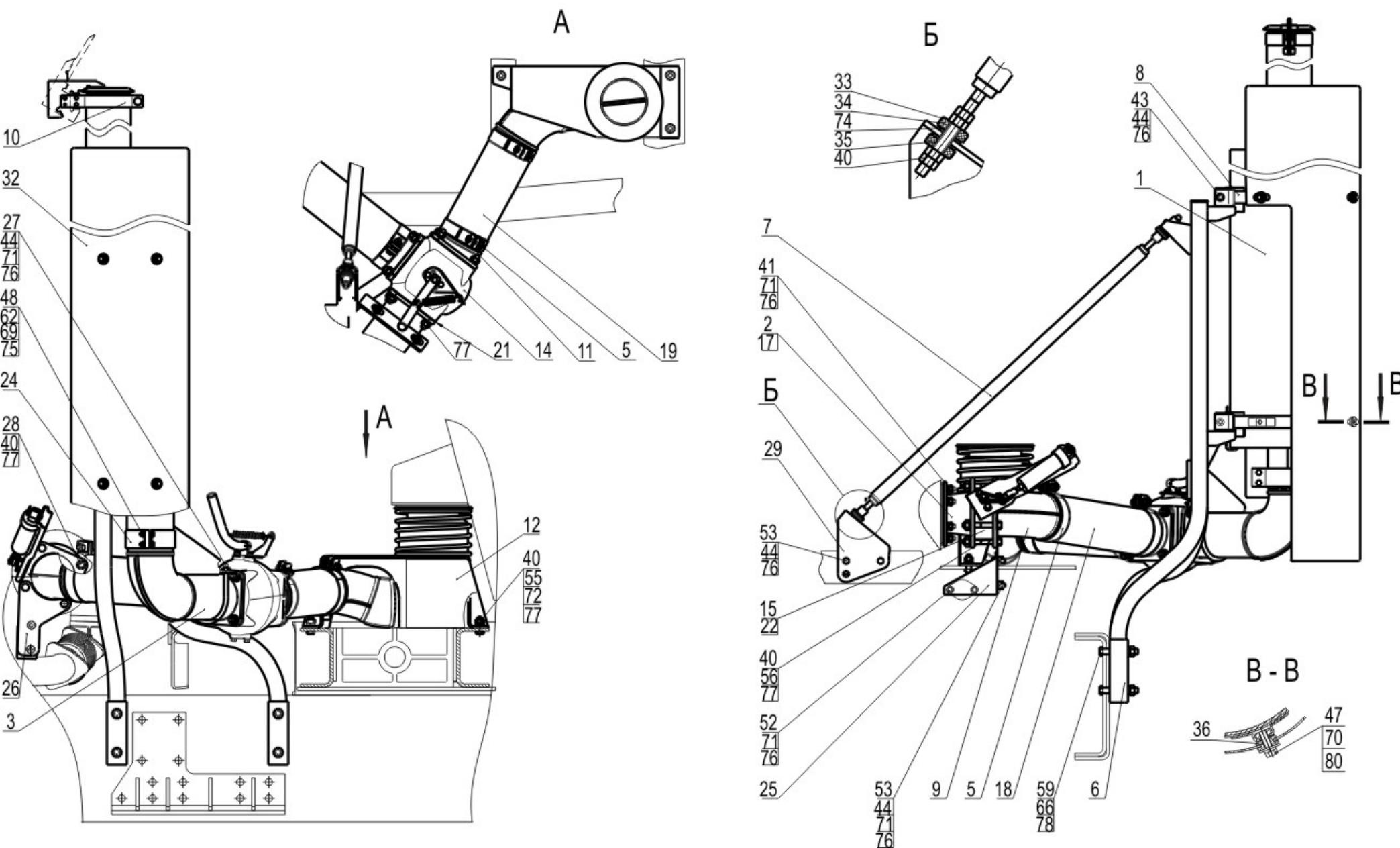
Fig. 27 Installing of gases exhaust system 651608-1200001-010
