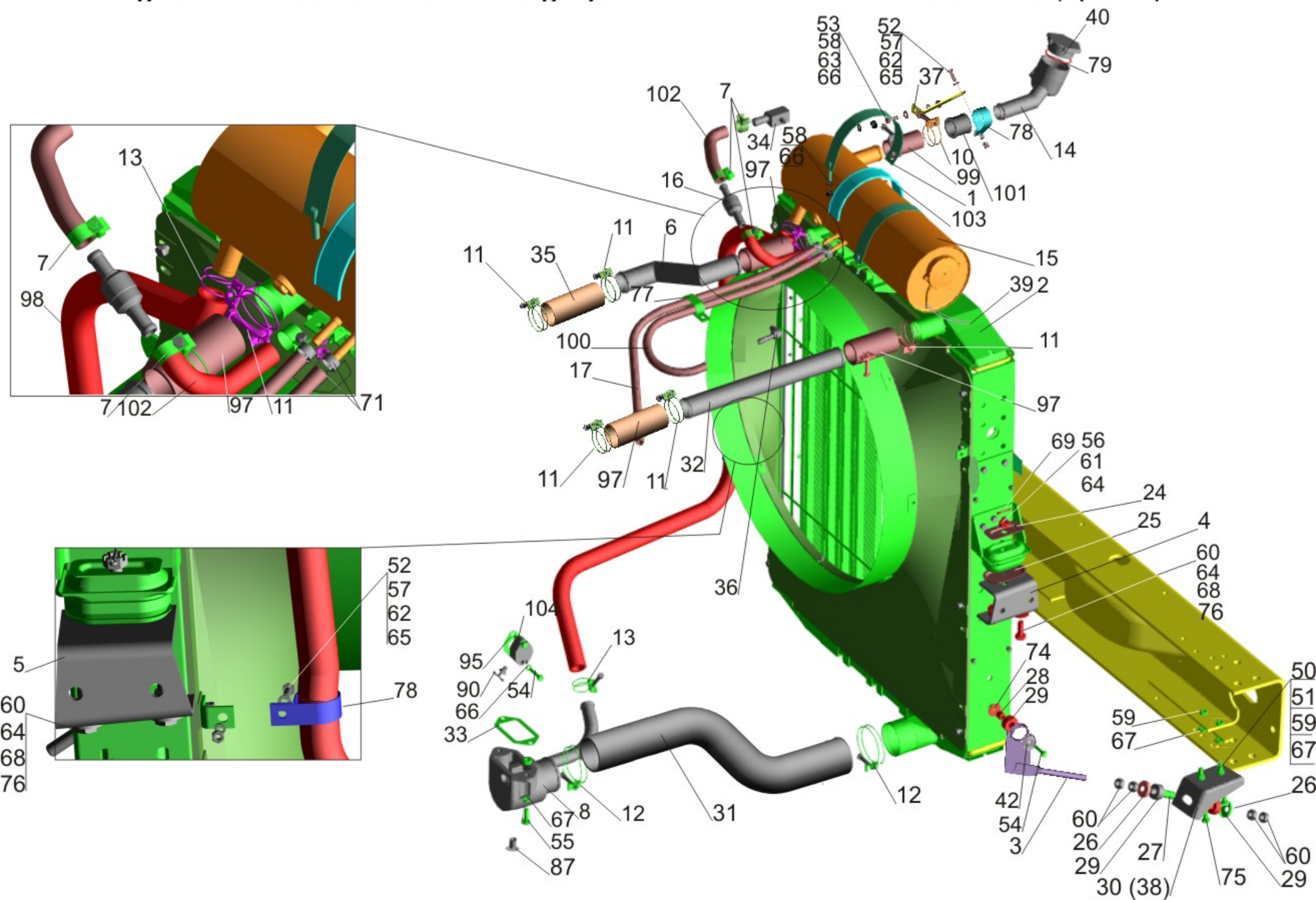
Fig.28 Installation of cooling system set 651608-1300005-000, (-010)
