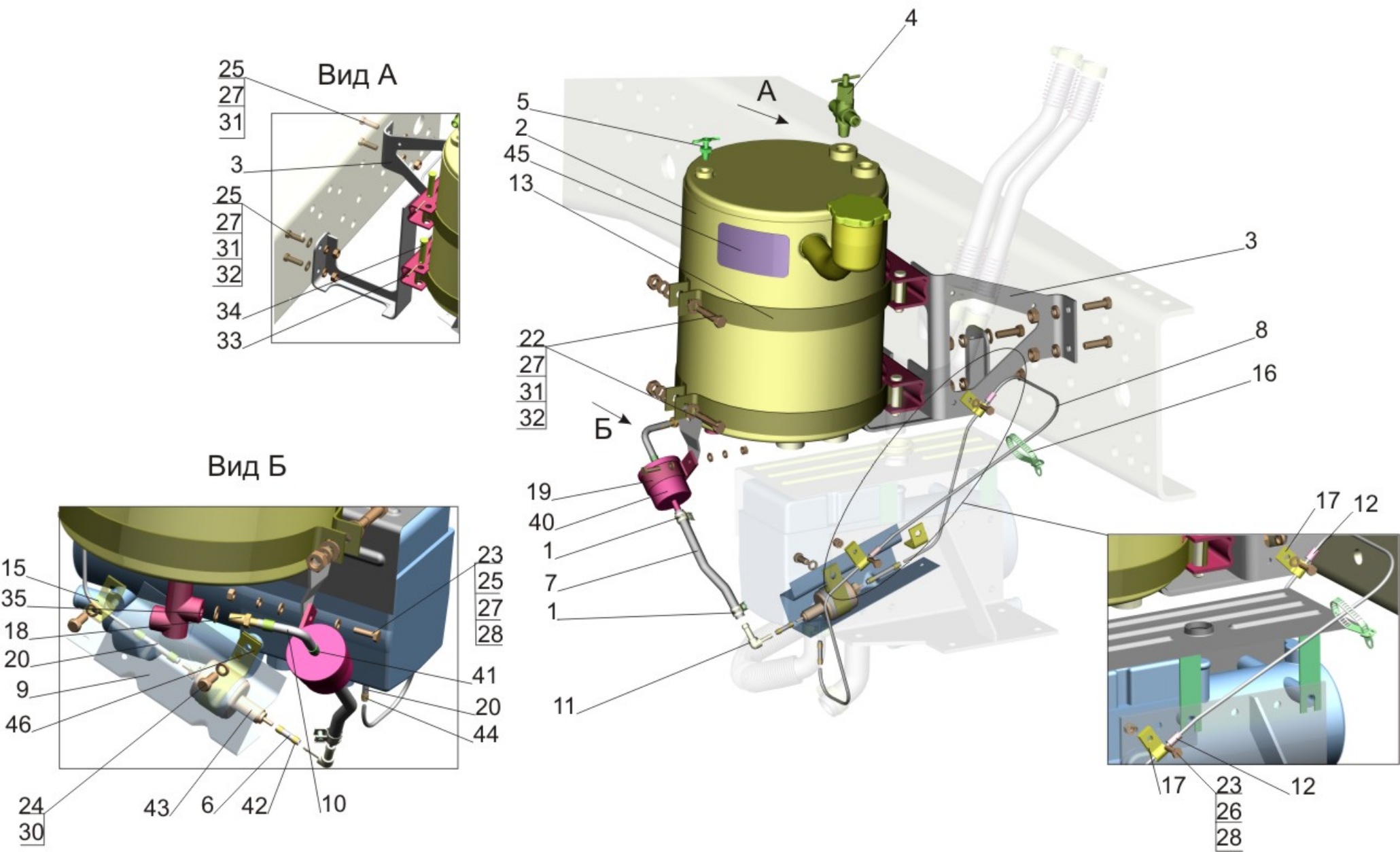
Fig.7 Mounting fuel lines of heater 651608-1015004
