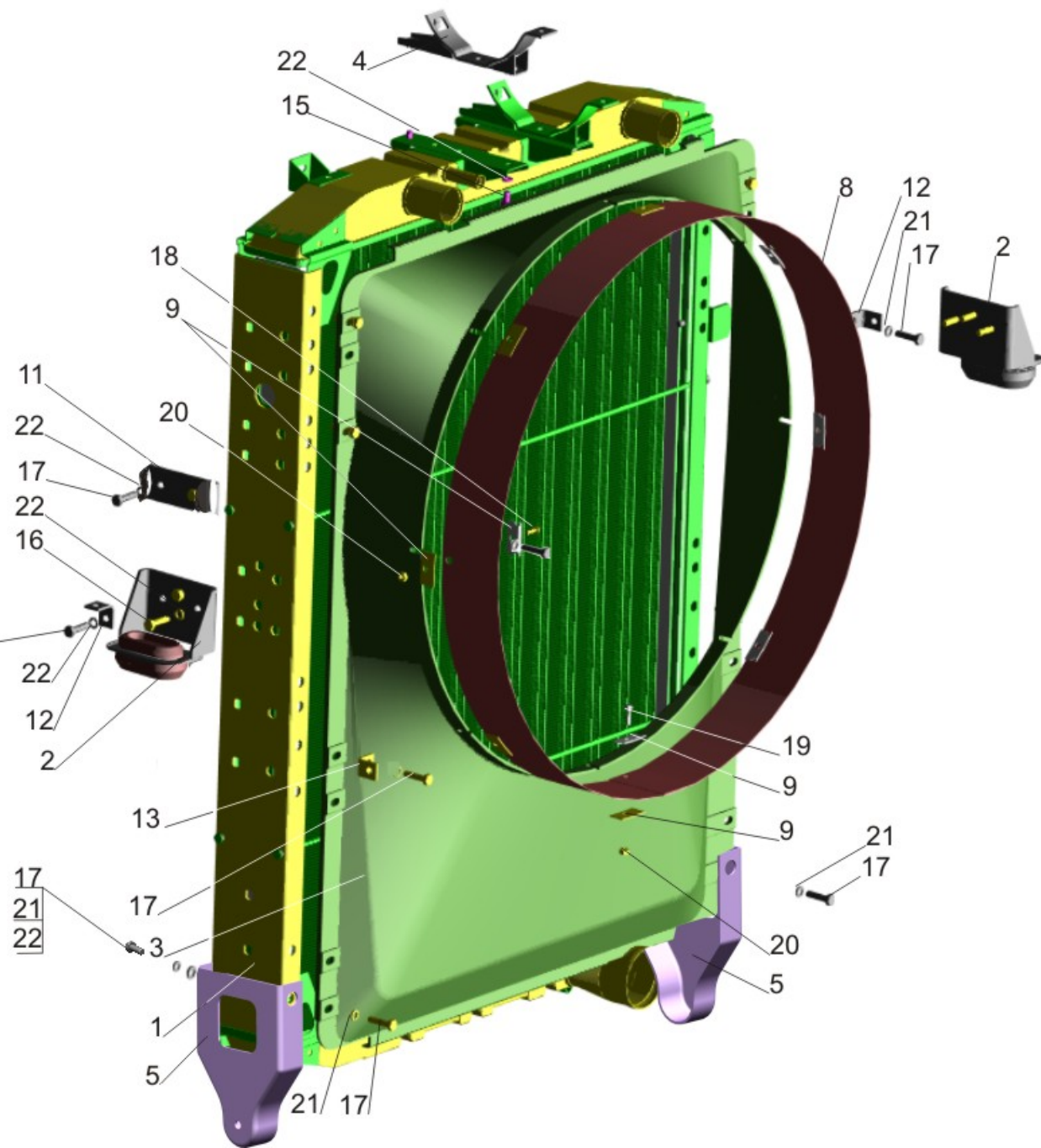
Fig.29 Cooler with housing 651608-1301009-000
