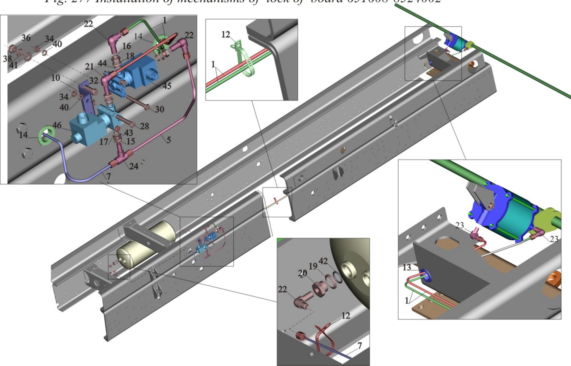
Fig. 277 Installation of mechanisms of lock of board 651608-8524002
