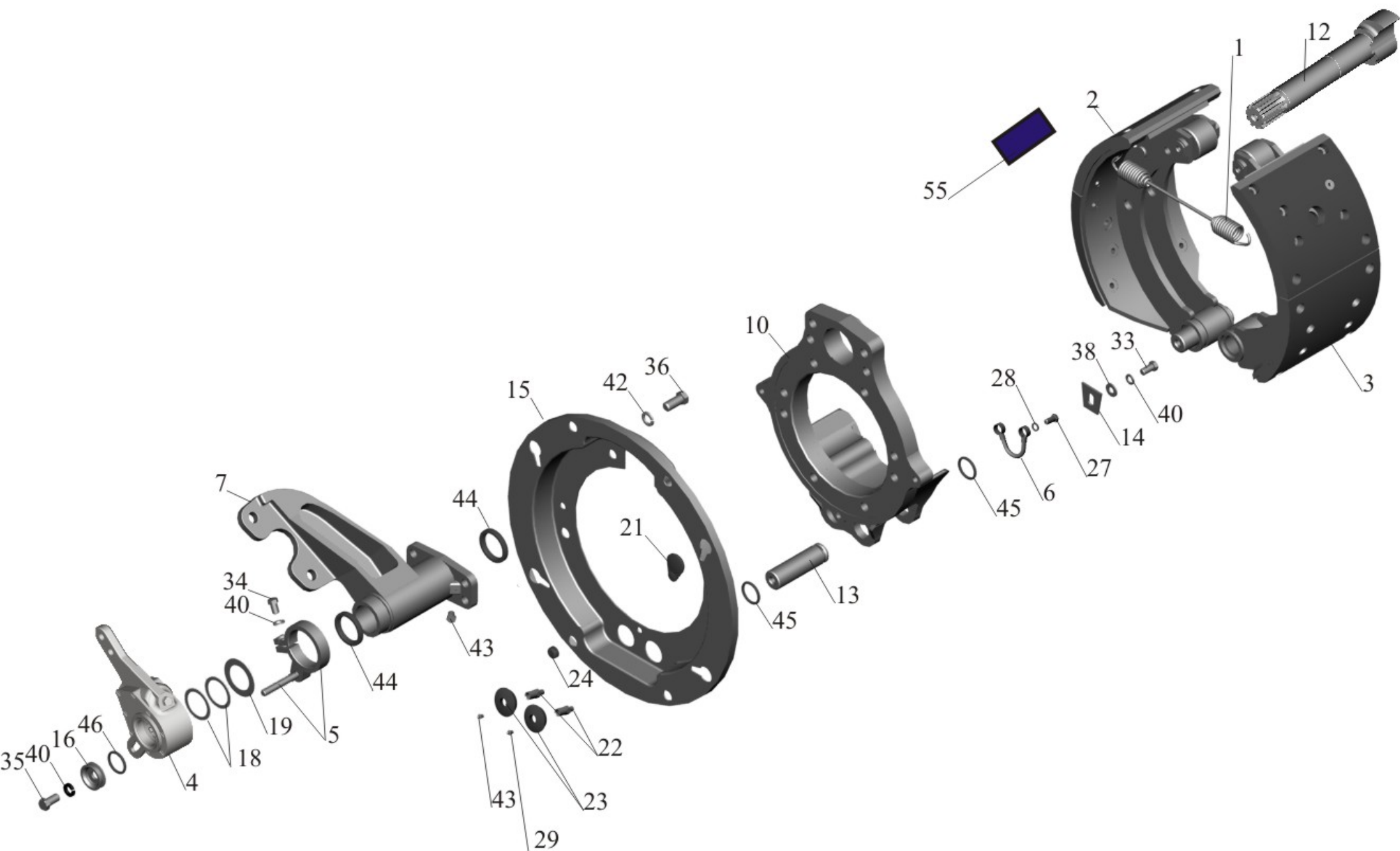
Fig. 111 Front brake 6516-3501004 (6516-3501005)
