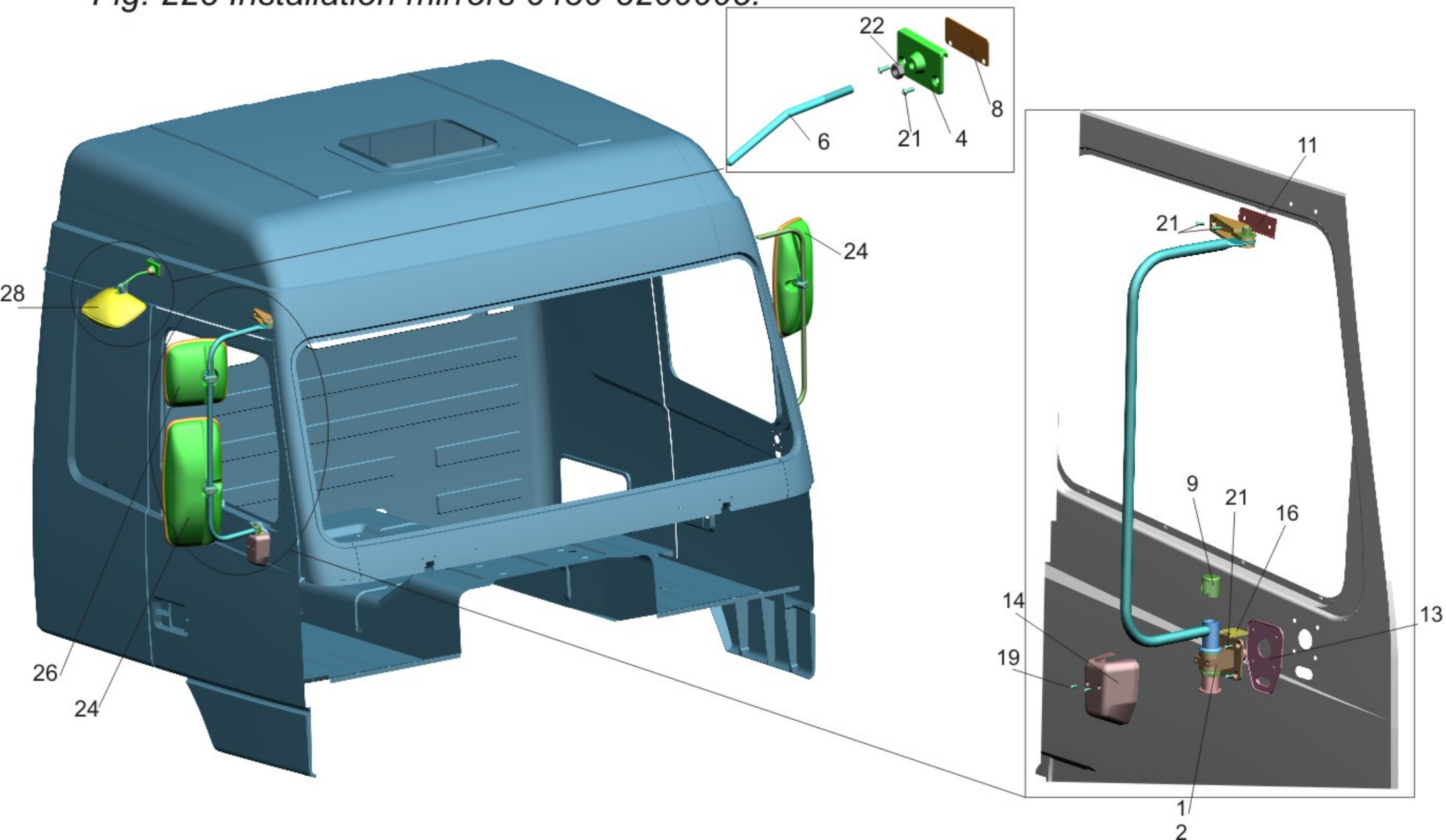
Fig. 228 Installation mirrors 6430-8200005.
