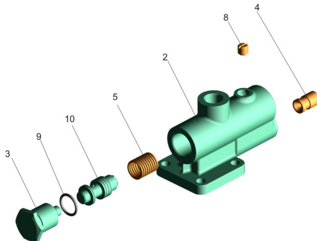
Fig. 150 Valve of the expense and pressure 6418-3407260
