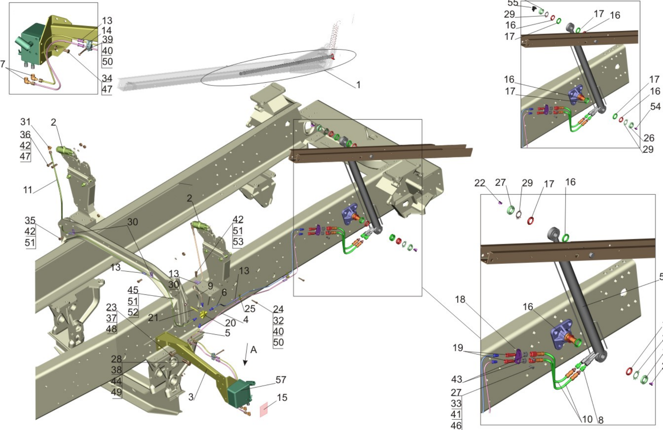
Fig. 237 Cab tilting mechanism 651608-5000040-010, (-011)
