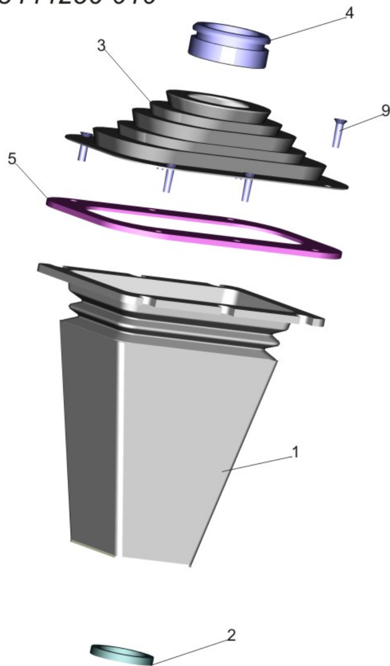
Fig. 151 Sealing hatch of cabin 5440-3444256-010
