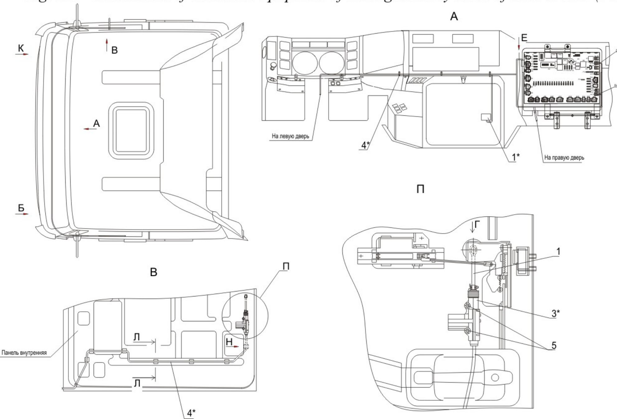
Fig. 183 Installation of electrical equipment of management by drive of central lock (Page1)
