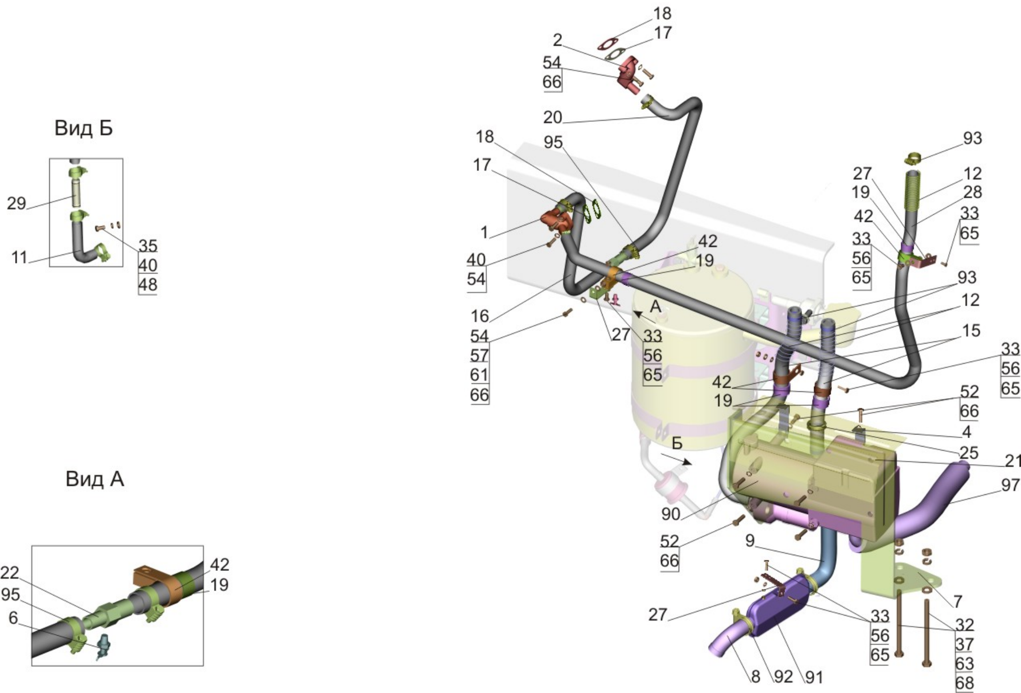
Fig. 6 Heater mounting 651608-1015001
