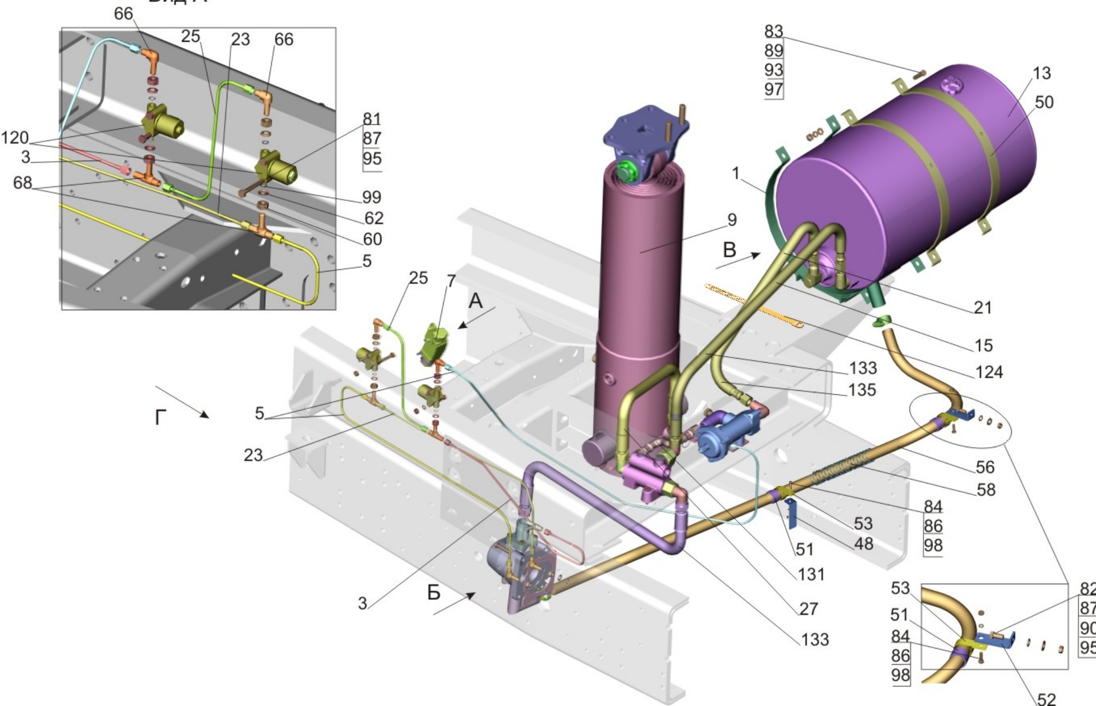
Fig. 285 Installation of hydroequipment 651608-8600005, 651608-8600005-700
