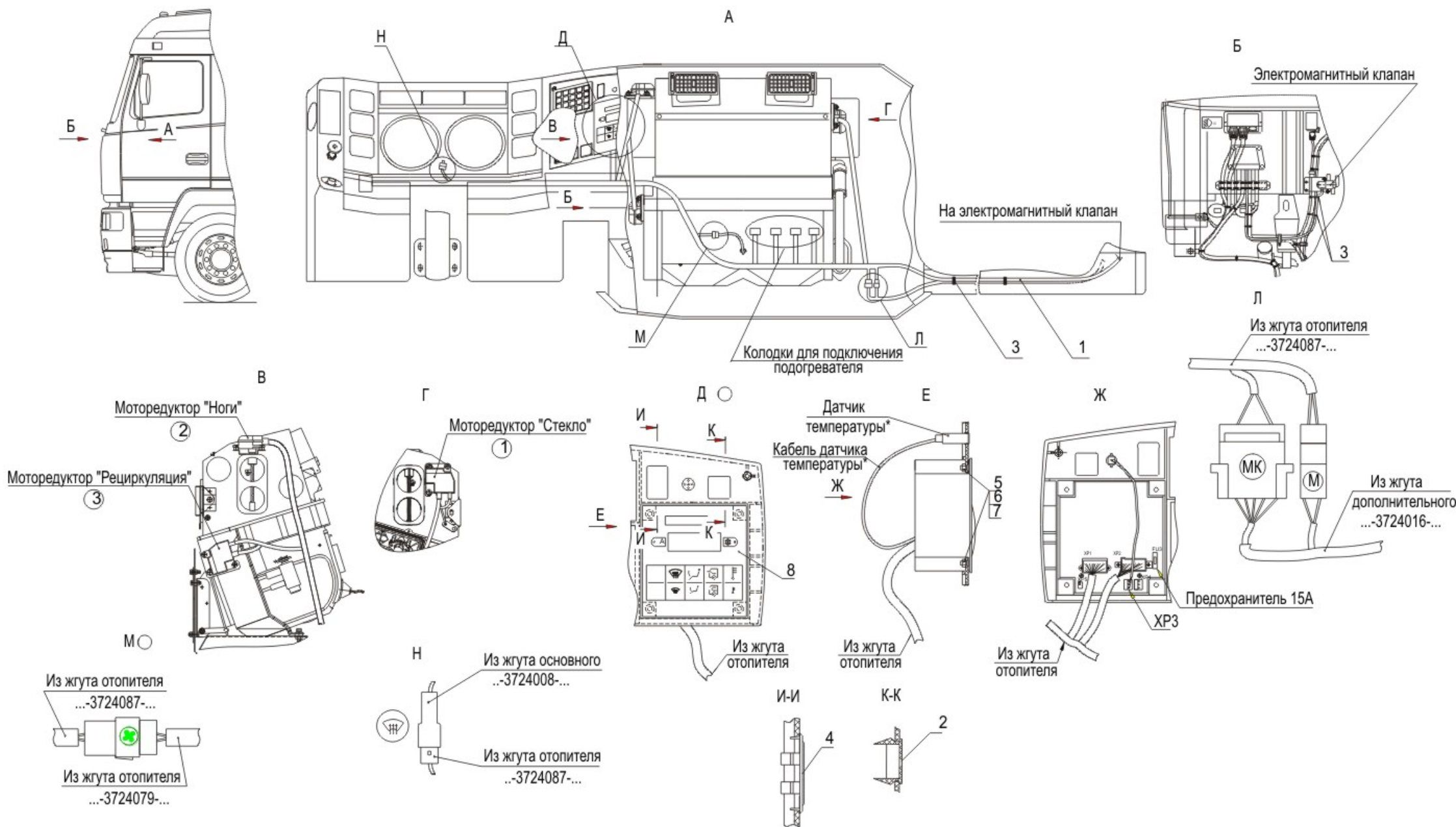
Fig. 193 Installation of an electric equipment of management microclimate 5440-3700103-010
