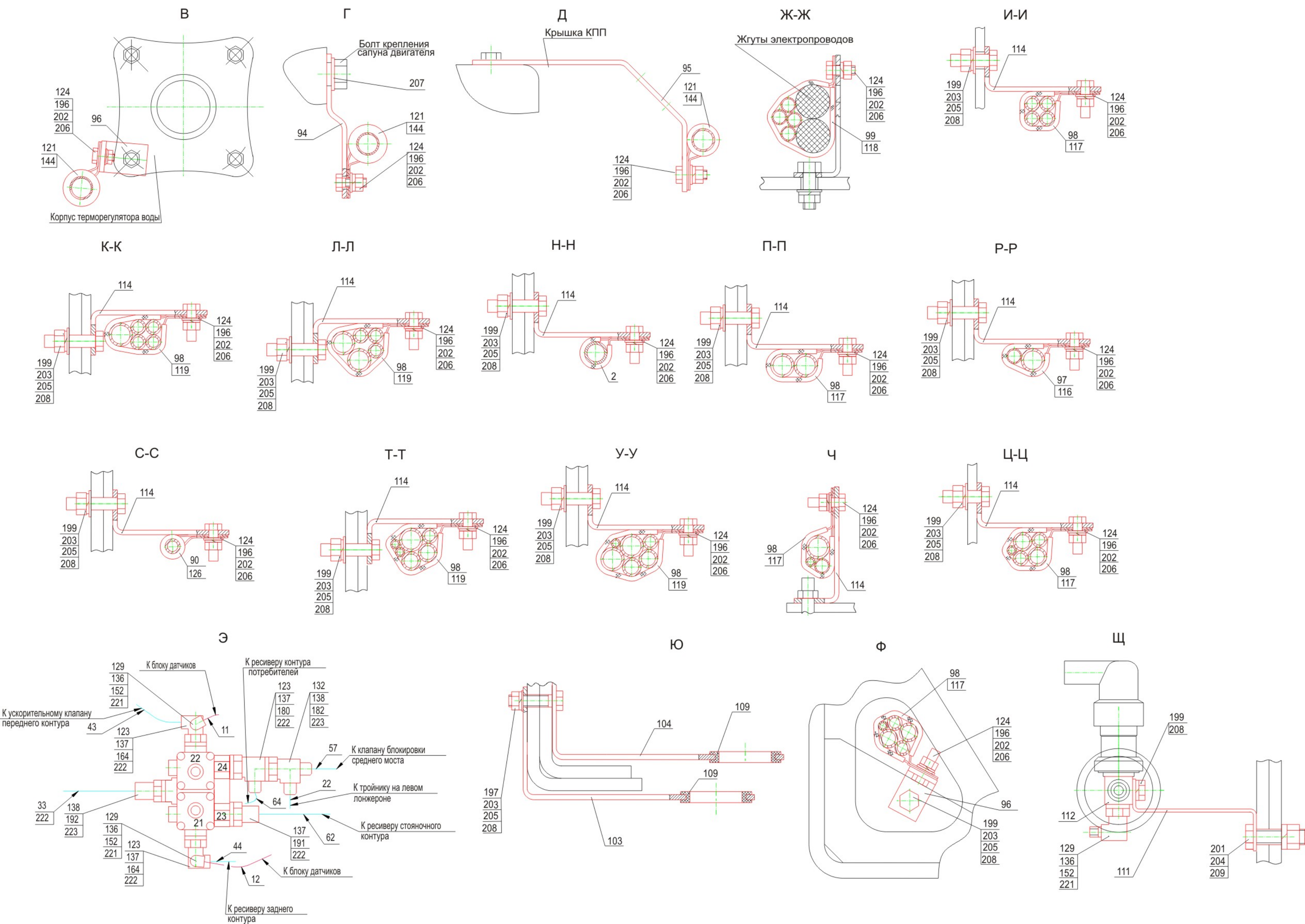
Fig. 154 Installation pneumobrakes
