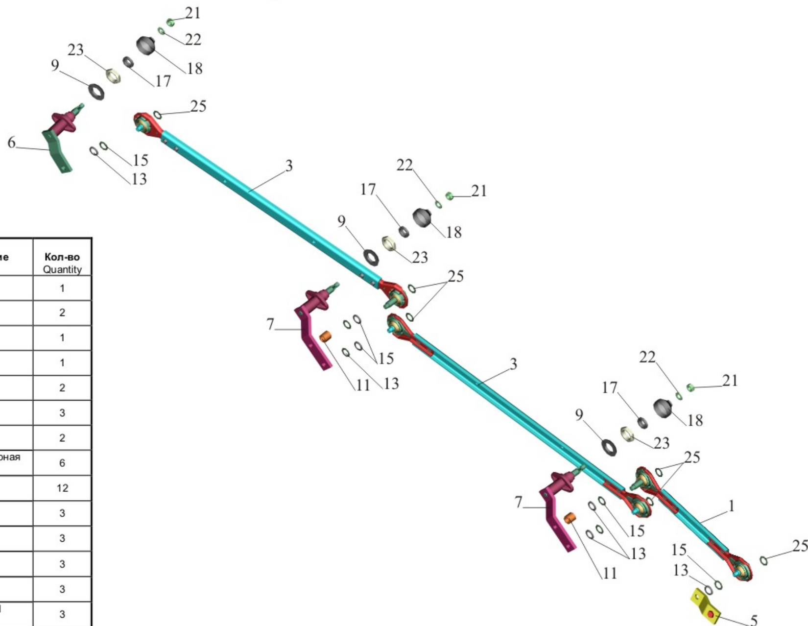
Fig. 235 Drive of cleaner of glasses 6430-5205500-010
