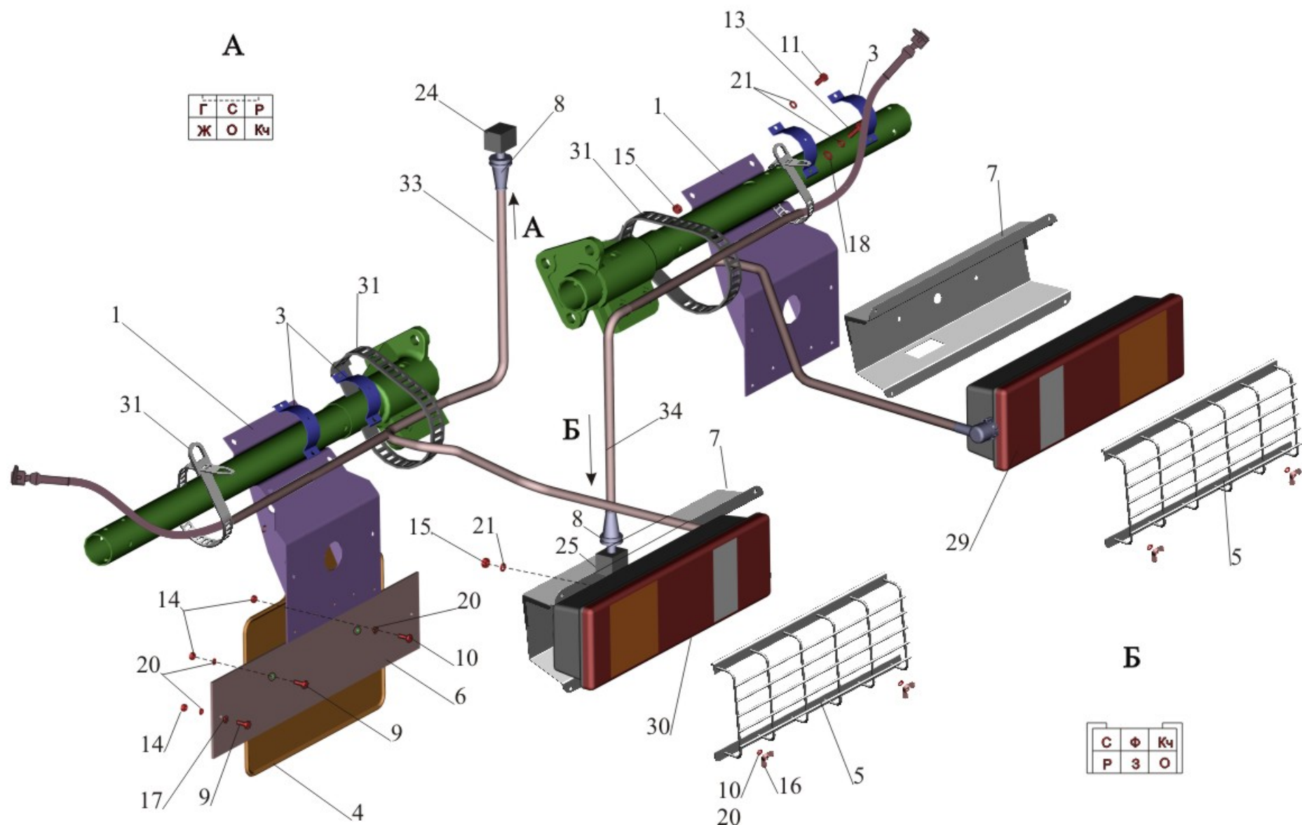
Fig. 177 Installation of tail lights 6516А8-3700009-010, 6516А8-3700009-710
