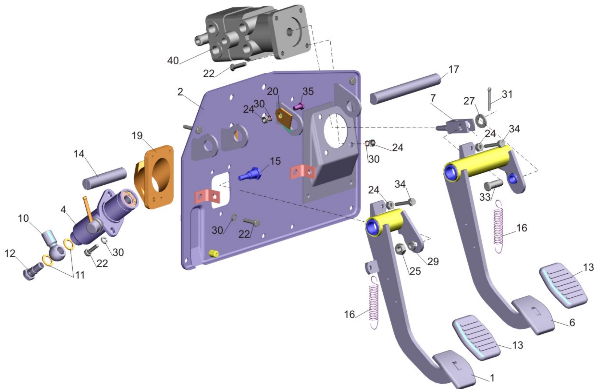
Fig. 32 Clutch and brake control unit 555035-1602004-010
