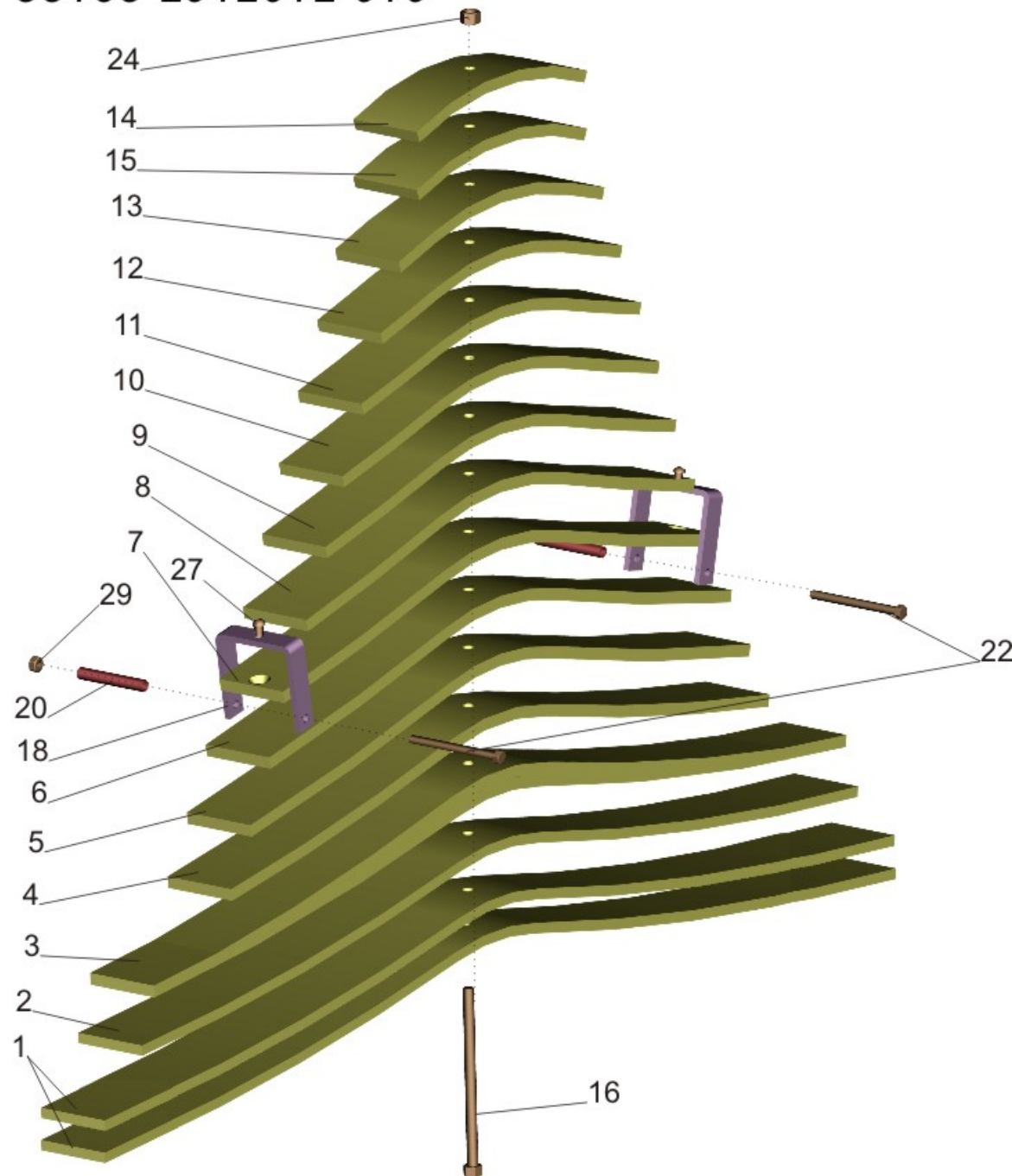
Fig. 98 Back leaf spring 55165-2912012-010
