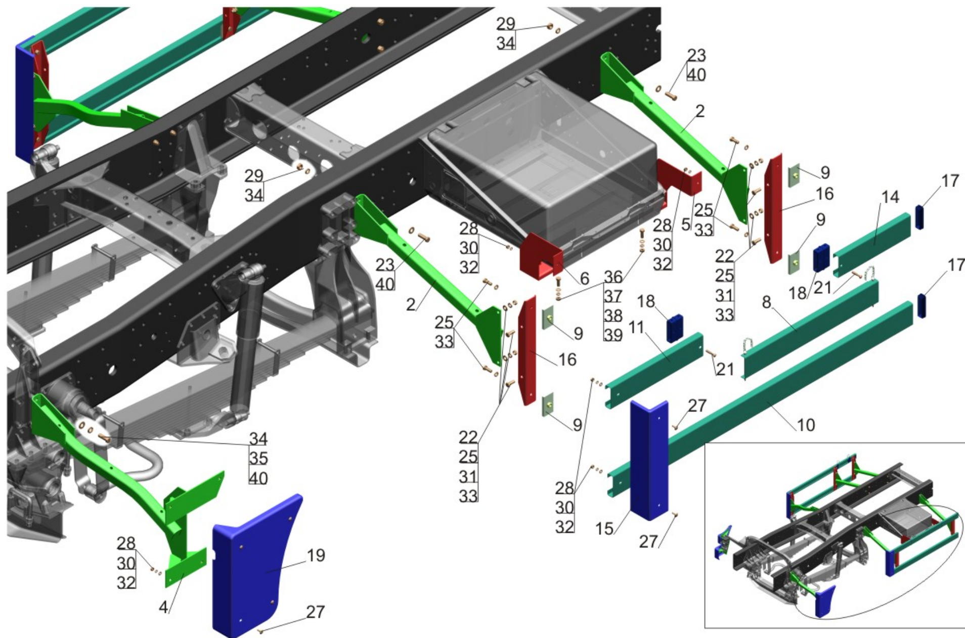
Fig.90 Installation of lateral protection 651608-2800040 (page 2)
