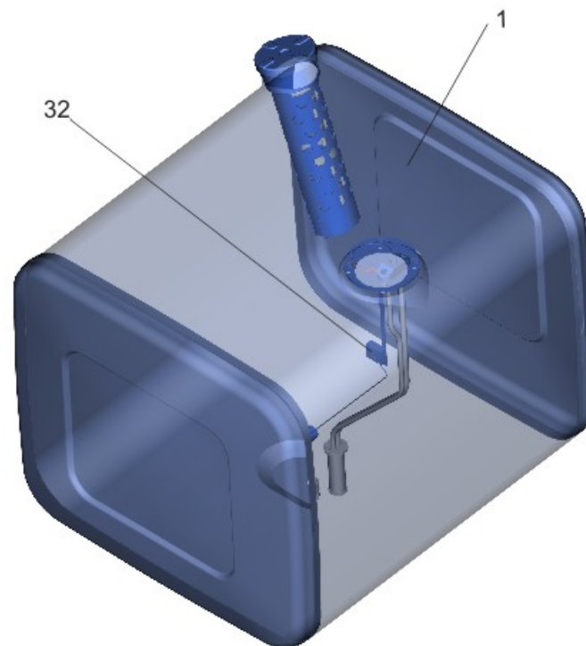
Fig. 11 Mounting of fuel tank 651608-1101002
