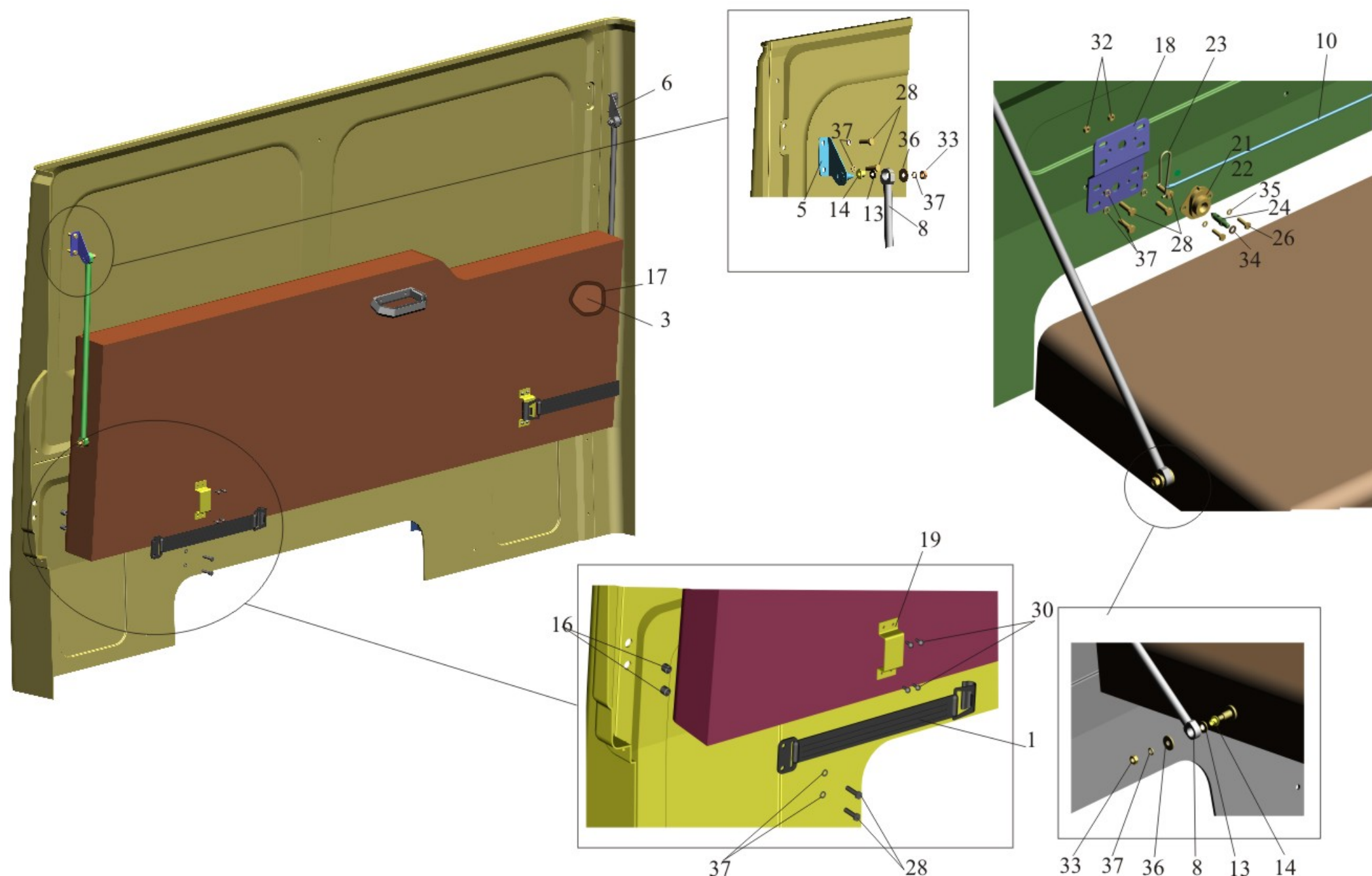
Fig. 269 Installation of a berth 6501-8200010
