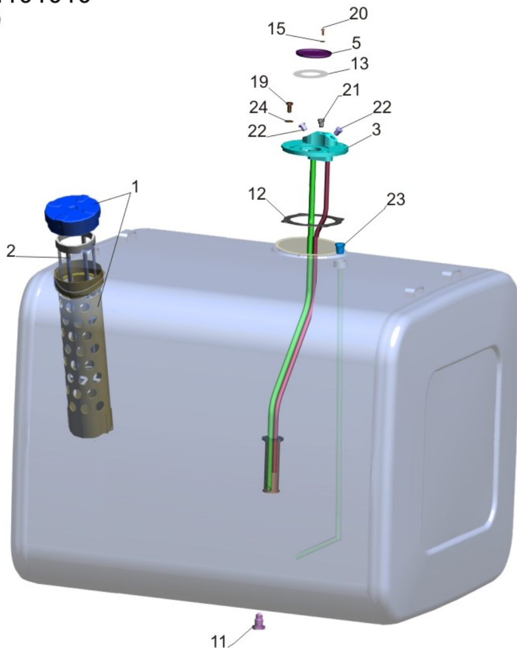
Fig. 12 Fuel tank 6501B5-1101010
