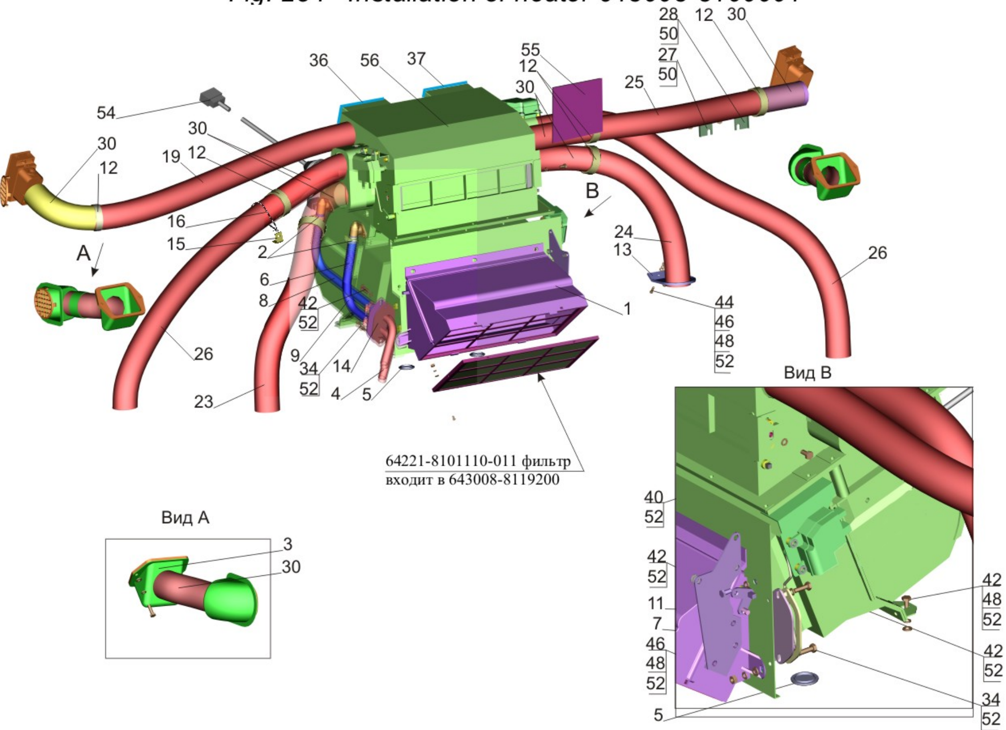
Fig. 254 Installation of heater 643008-8100001
