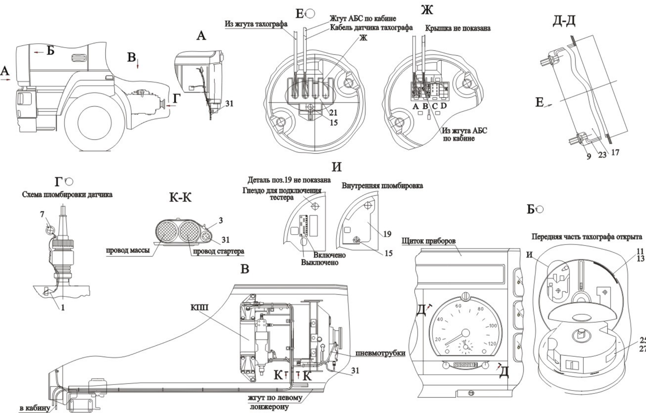
Fig. 201 Installation and identification seal of a tachograph 5440-3800005-040
