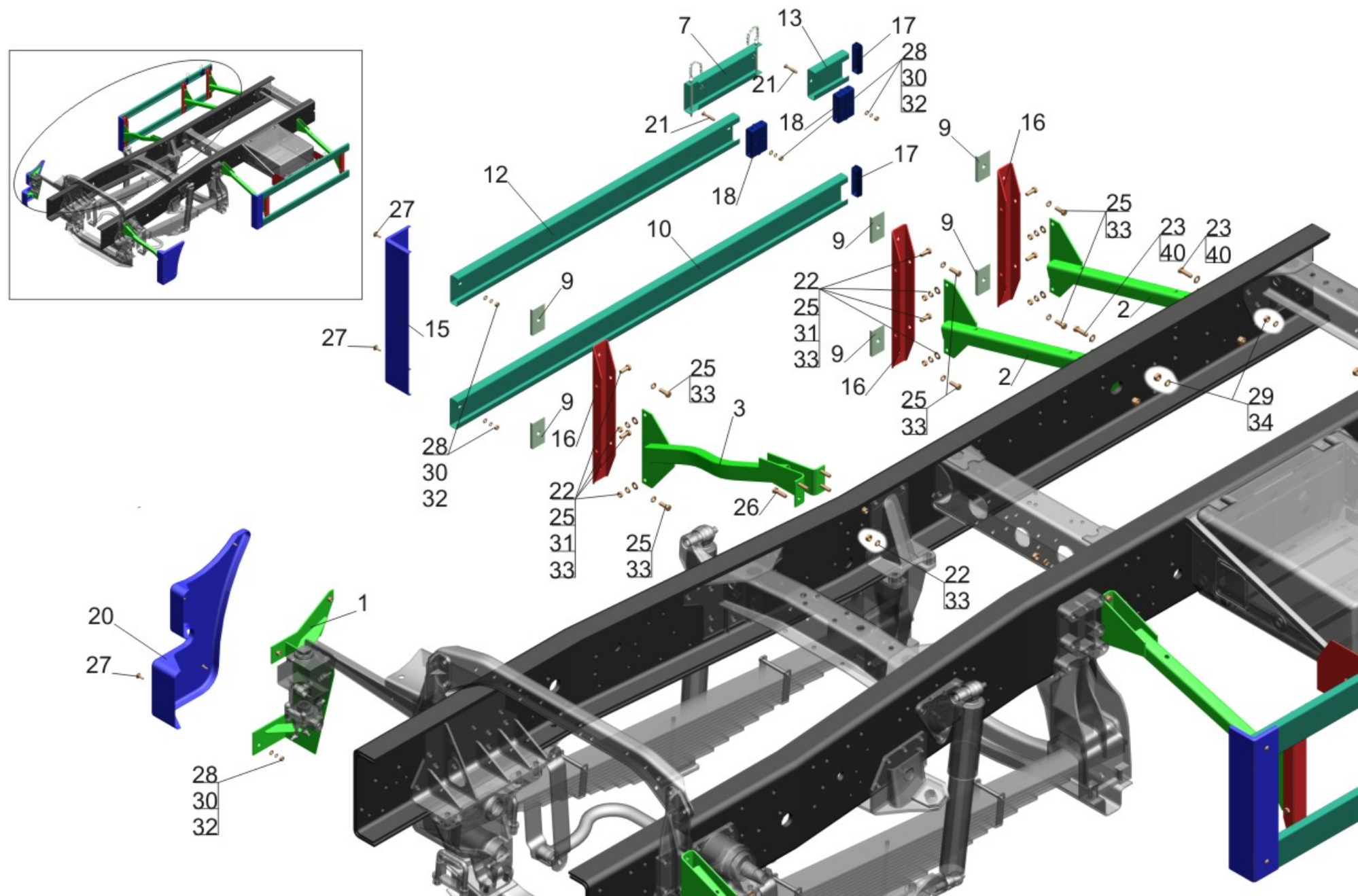
Fig.90 Installation of lateral protection 651608-2800040 (page 1)
