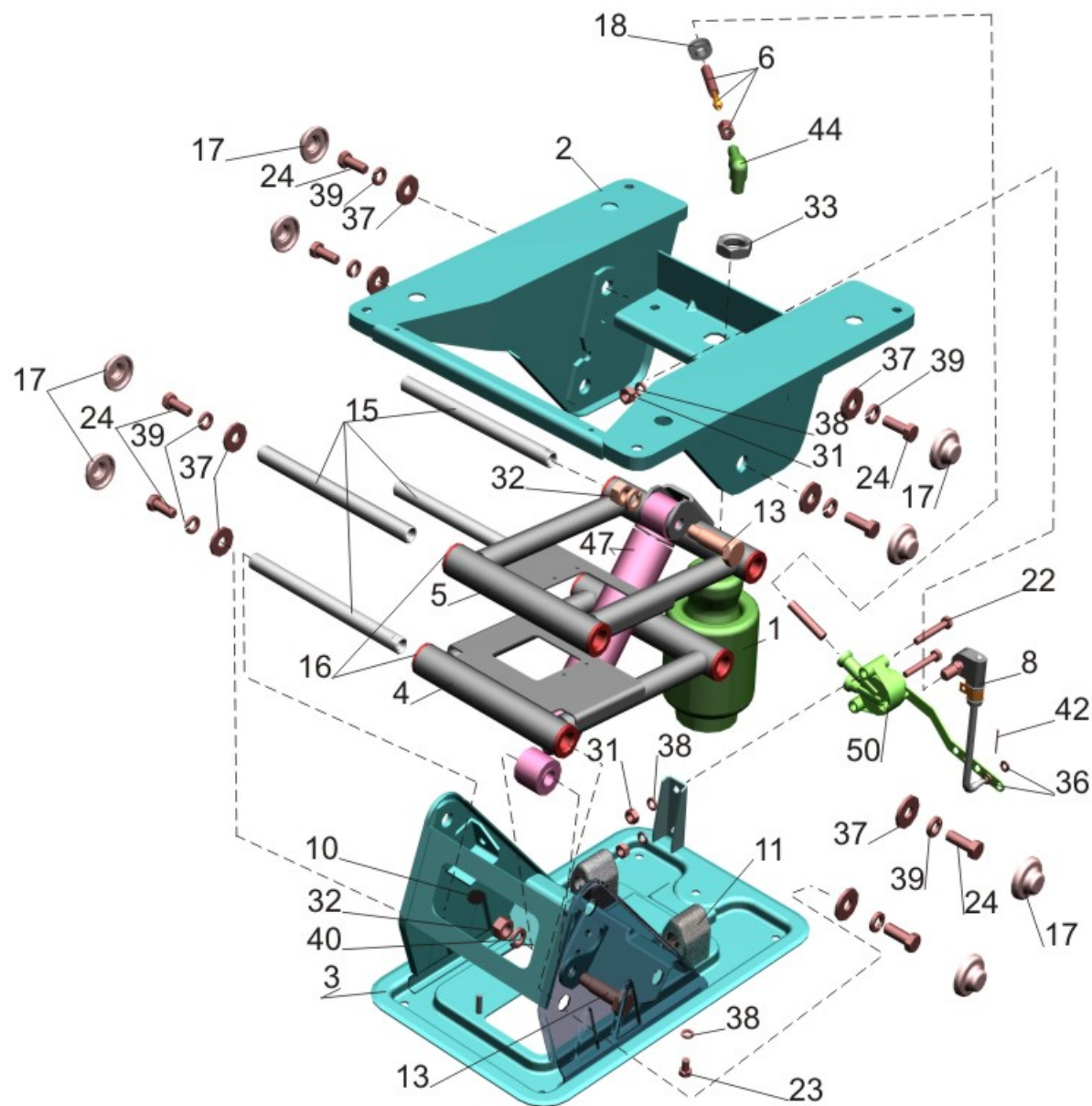
Fig. 248 Seat support with pneumatic equipment 6430-6807006-010
