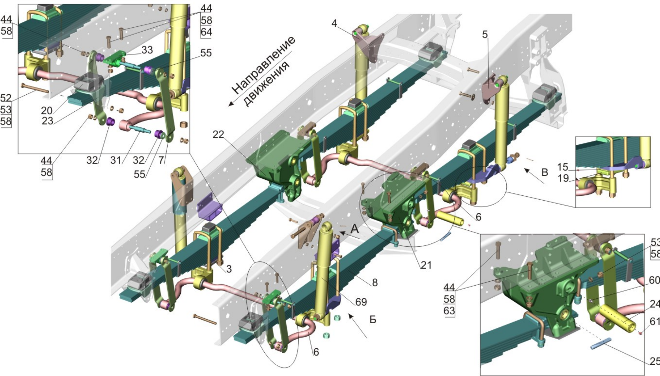
Fig. 93 Mounting front suspension 651608-2900001 (page 1)
