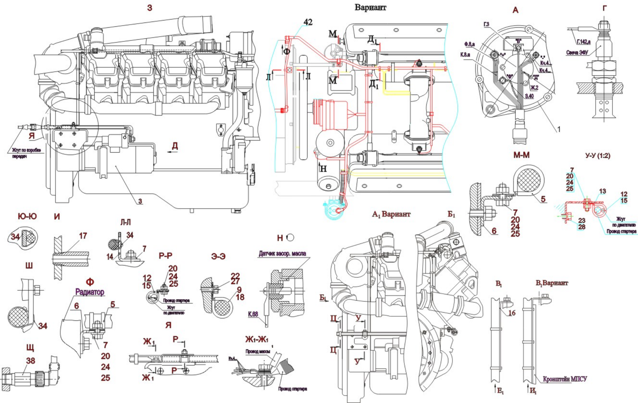
Fig.189 Electric equipment installation on the engine (page 2)
