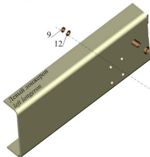
Fig. 157 Mounting of receivers 650108-3513005
