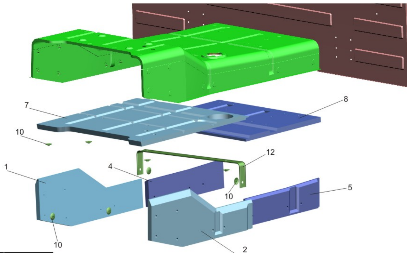
Fig. 220 Installation additional tehrho noise isolations 6501-5000122
