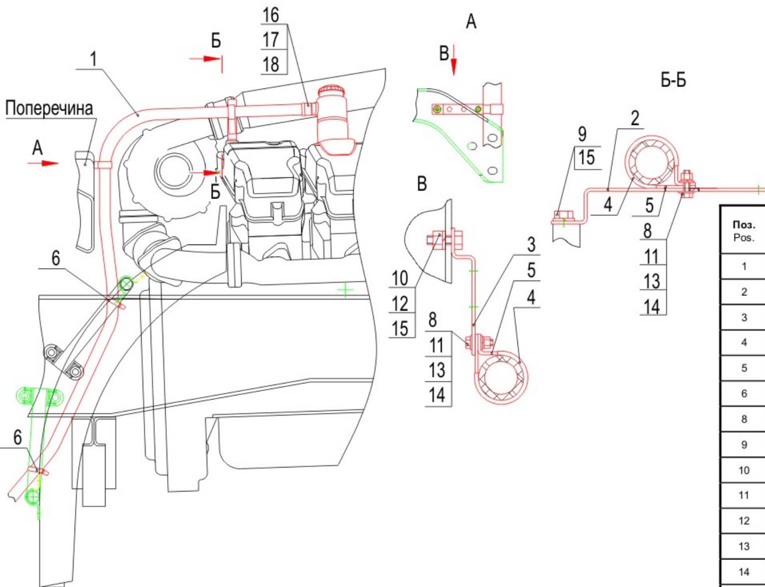
Fig. 2 Installation breathing of engine 641808-1014002
