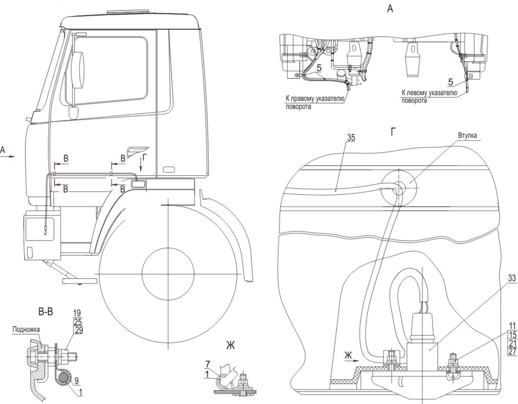
Fig. 273 Installing of turn indicator side 530905-3700150(-700)
