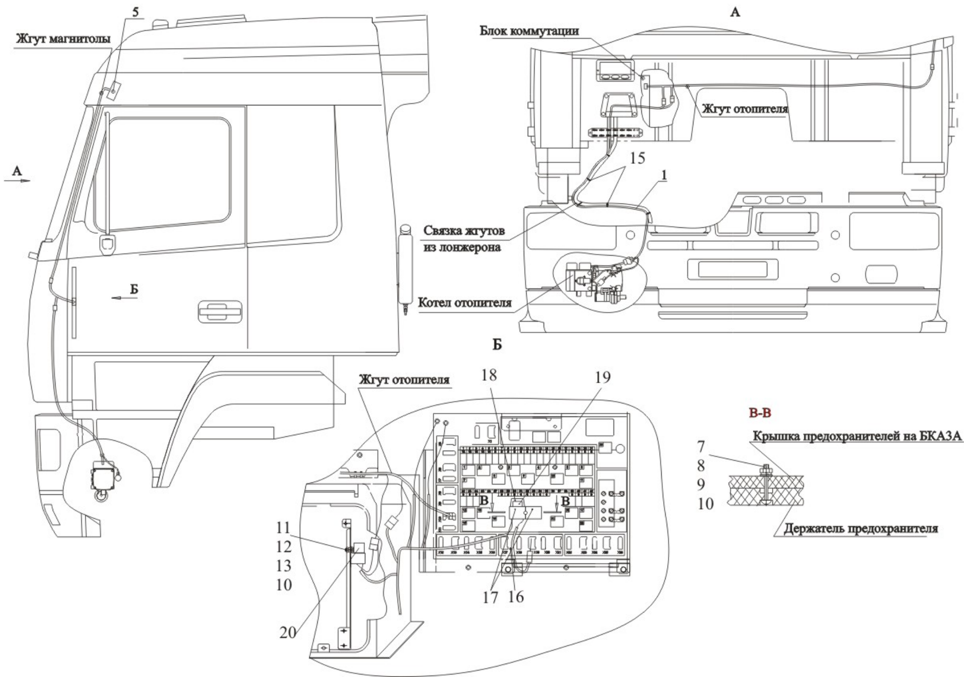
Fig. 203 Mounting of electrical equipment heater 544003-3700085
