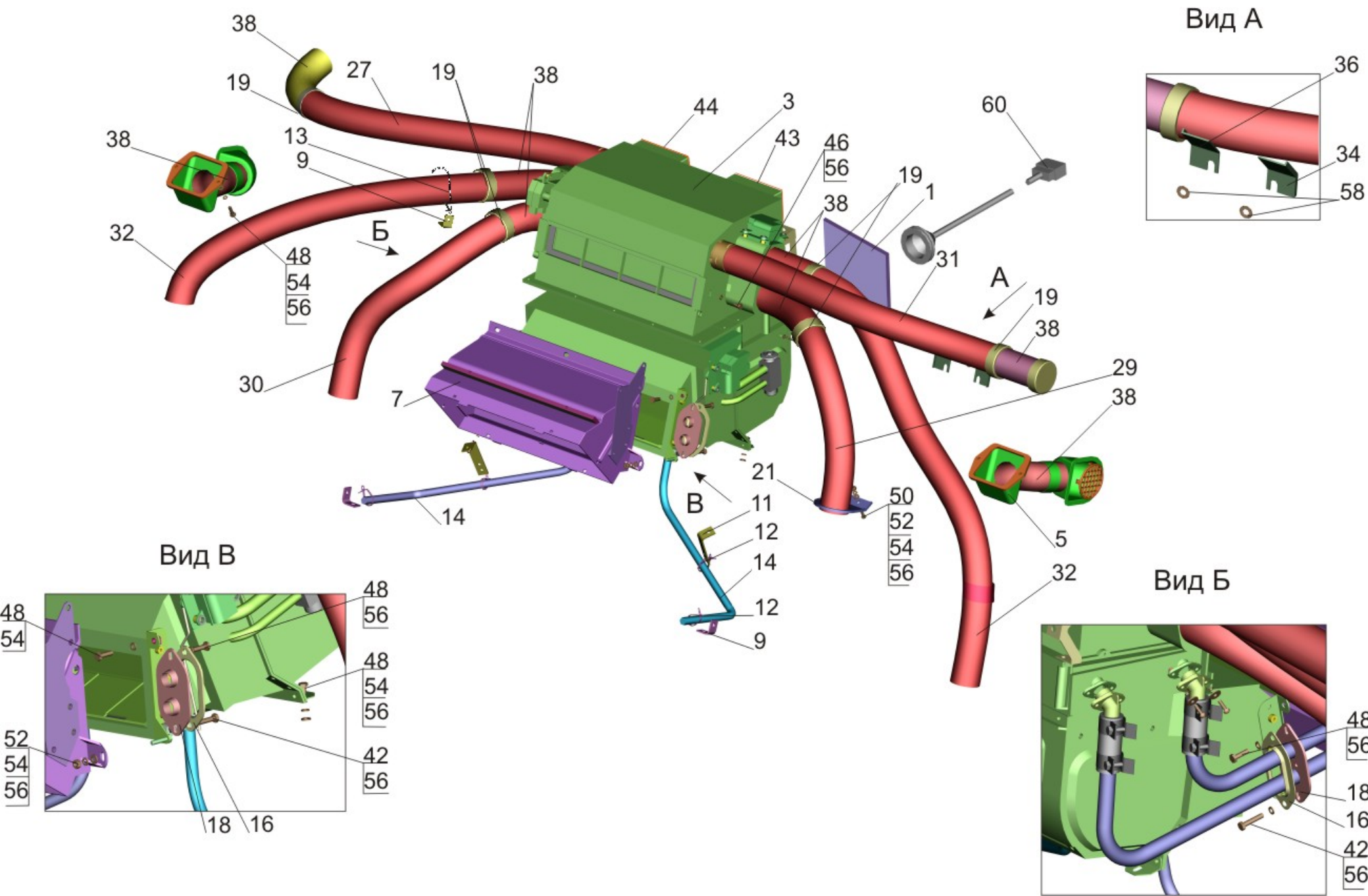
Fig. 253 Installation of heater 631019-8100001-010
