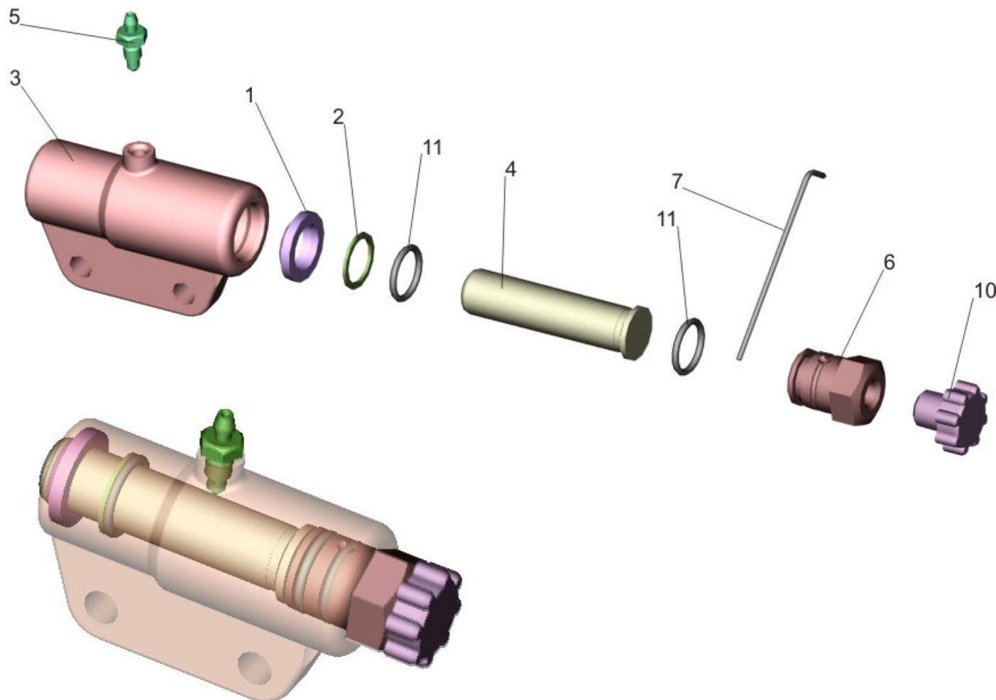
Fig. 239 Hydrocylinder 6430-5003100
