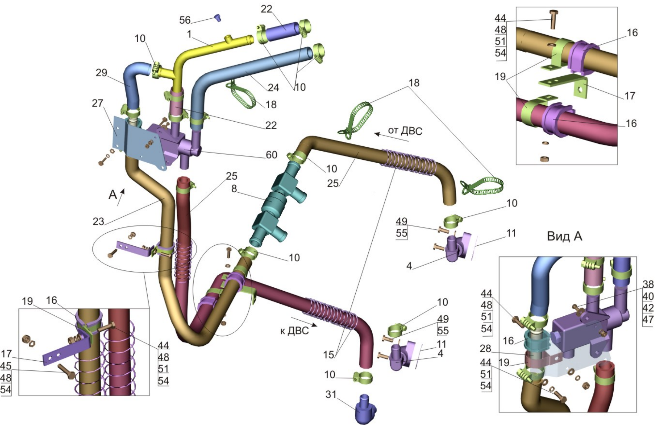
Fig. 263 Installation of hoses heater 544004-8100006-030
