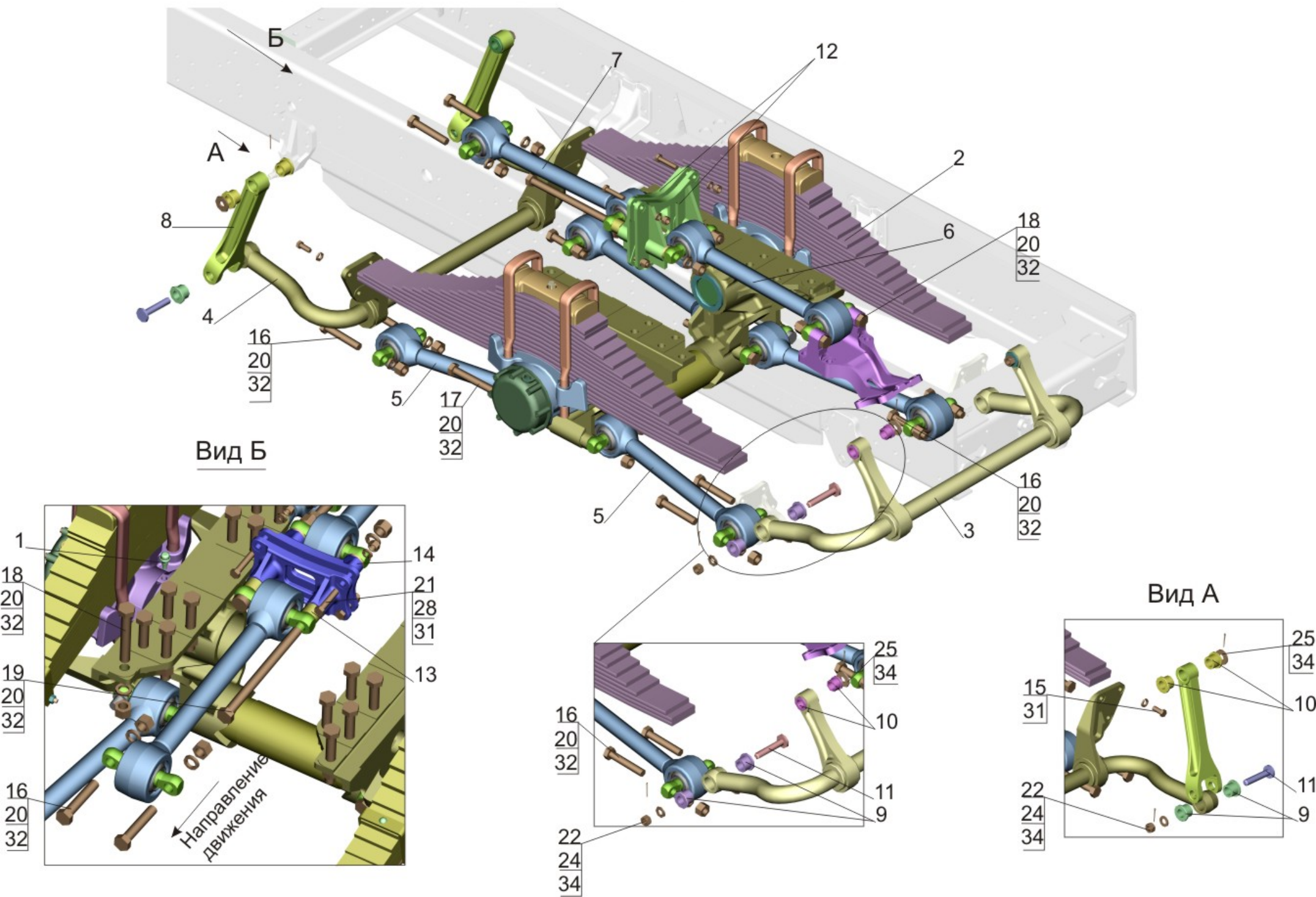
Fig.96 Installation beam suspension 651608-2900002
