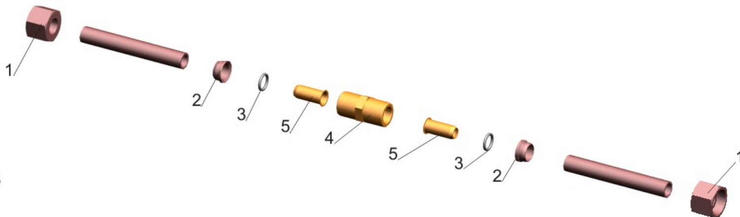
Fig.172 Connection for repair of the damaged pipelines
