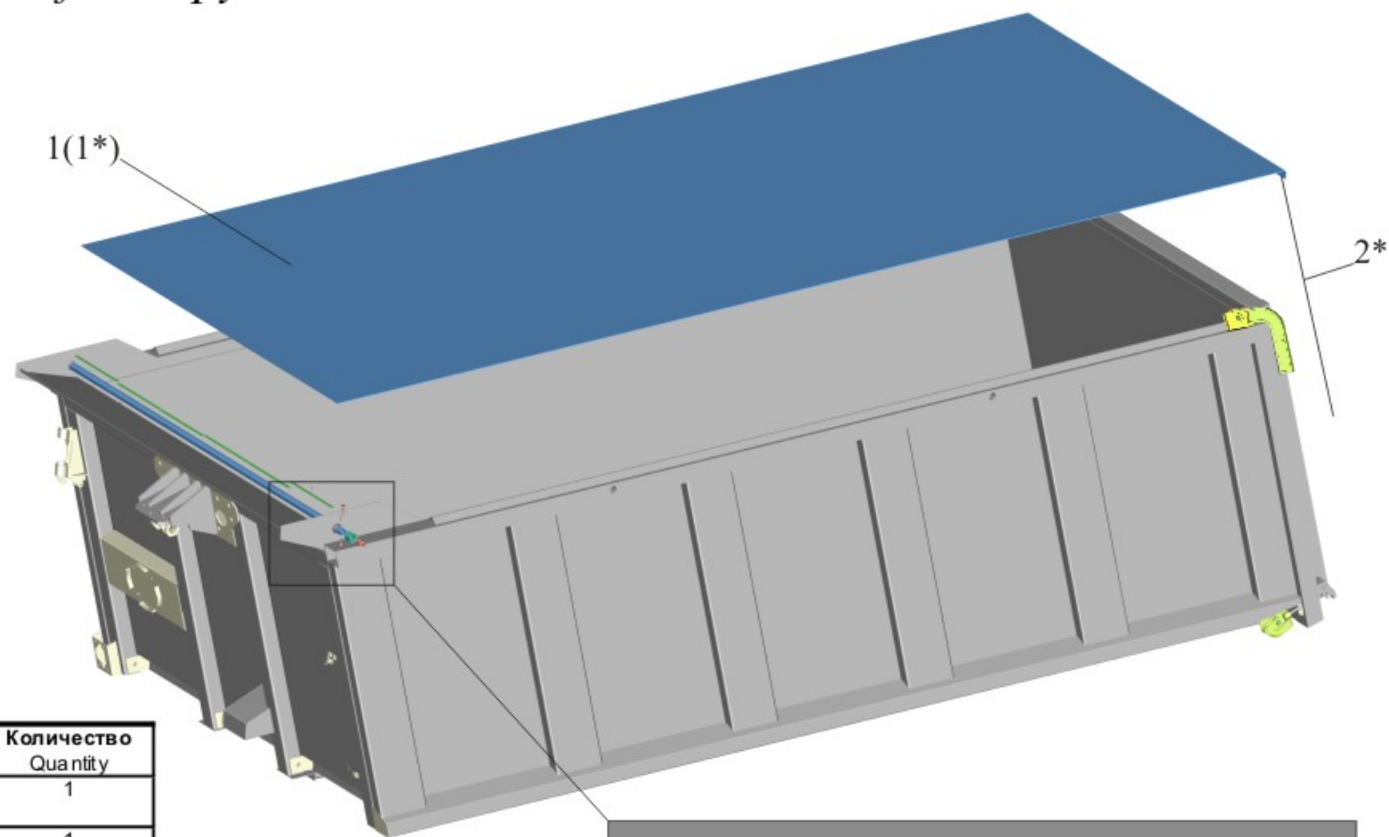
Fig. 280 Installation of canopy 651608-8500004
