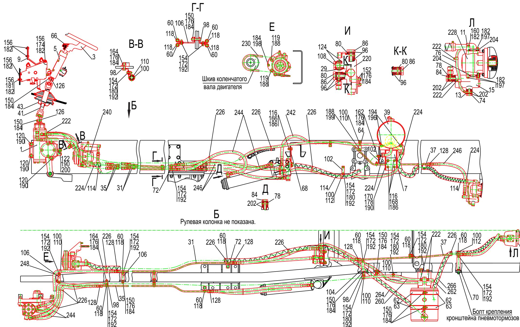
Fig. 134 Steering installation 651608-3400001
