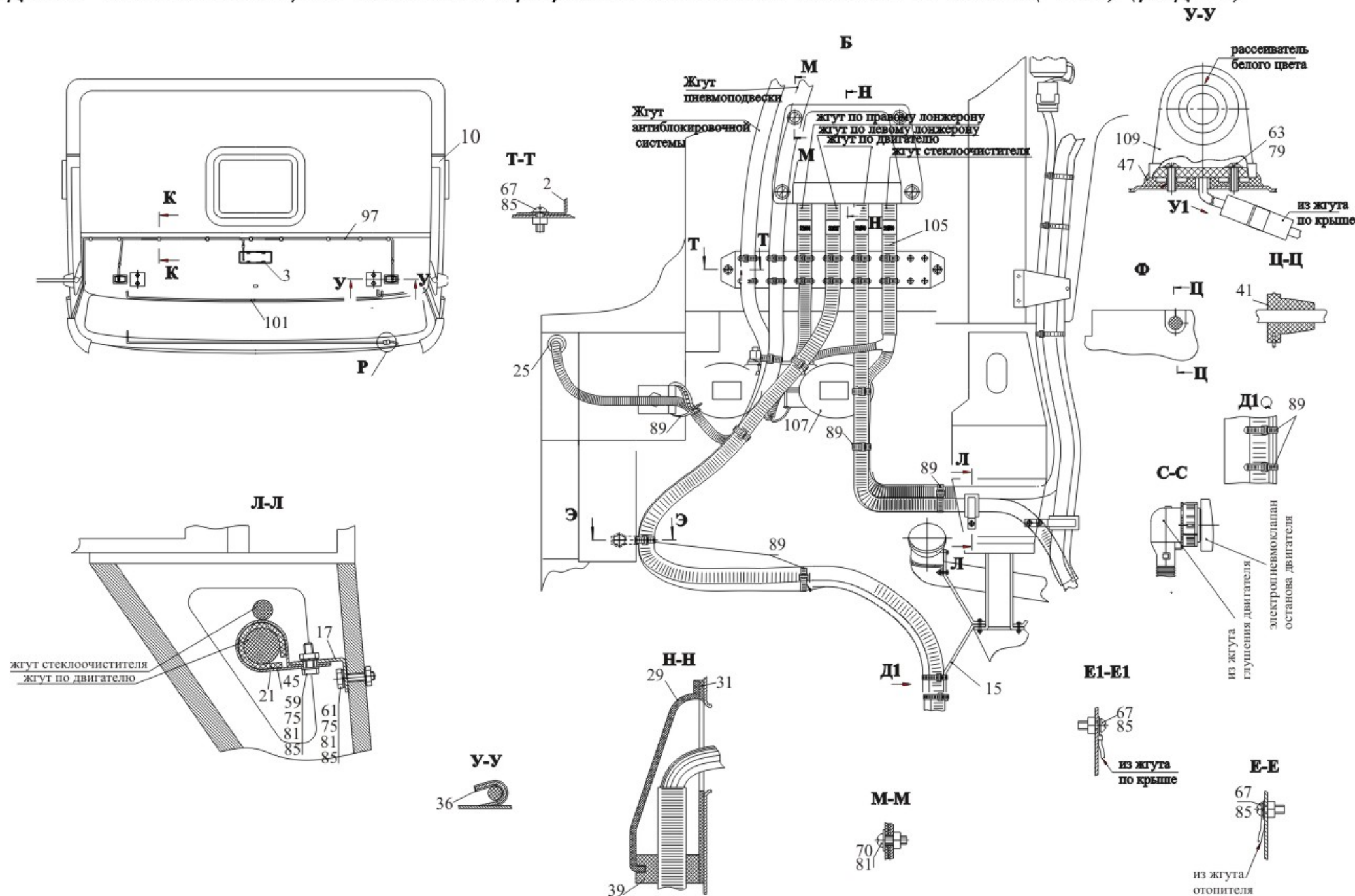
Fig.181 Installation of an electrical equipment in a cabin 555002-3700076(-700) (page 2)
