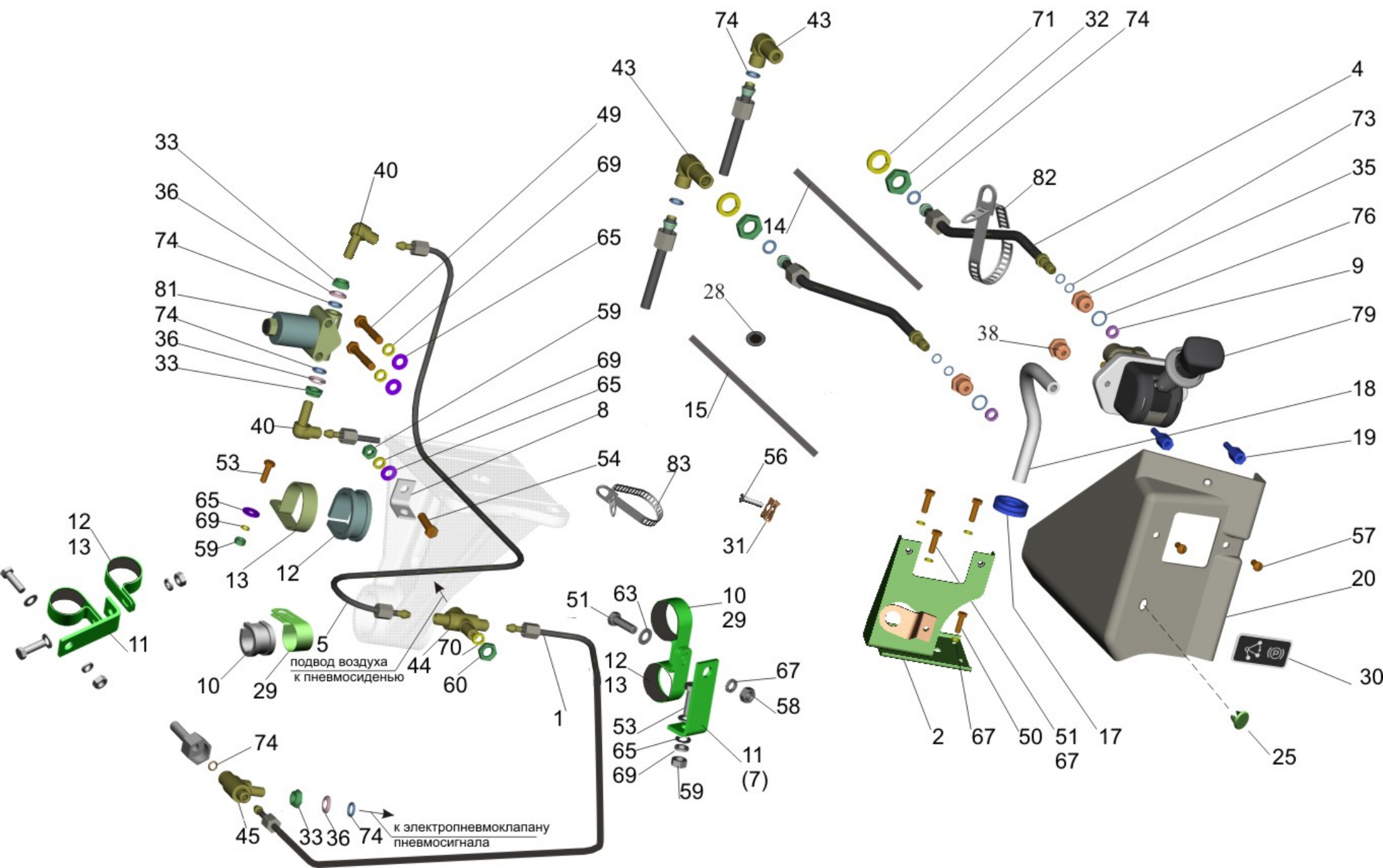
Fig. 169 Drive parking and motor brake.
