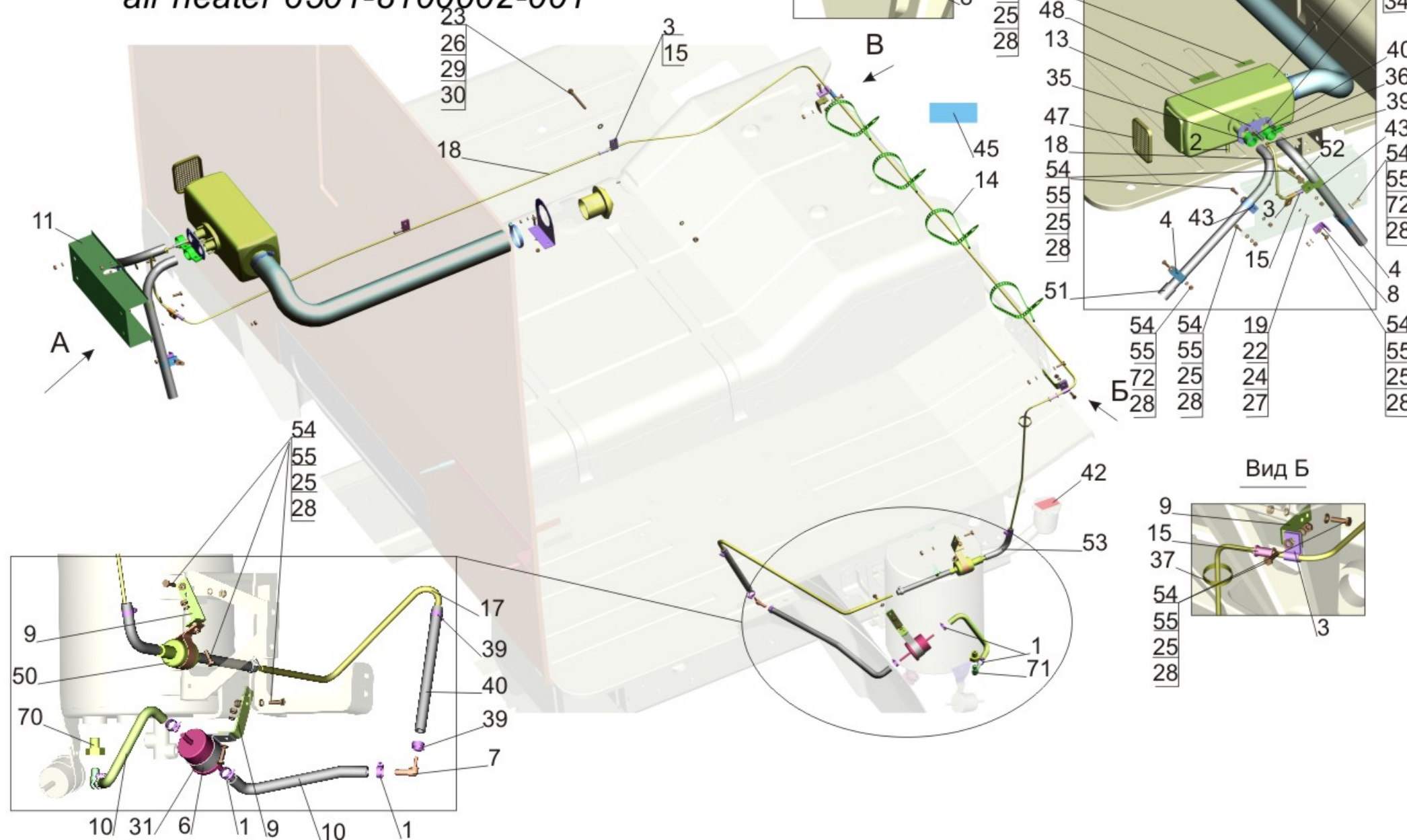
Fig. 264 Installation of the independent air heater 6501-8100002-001
