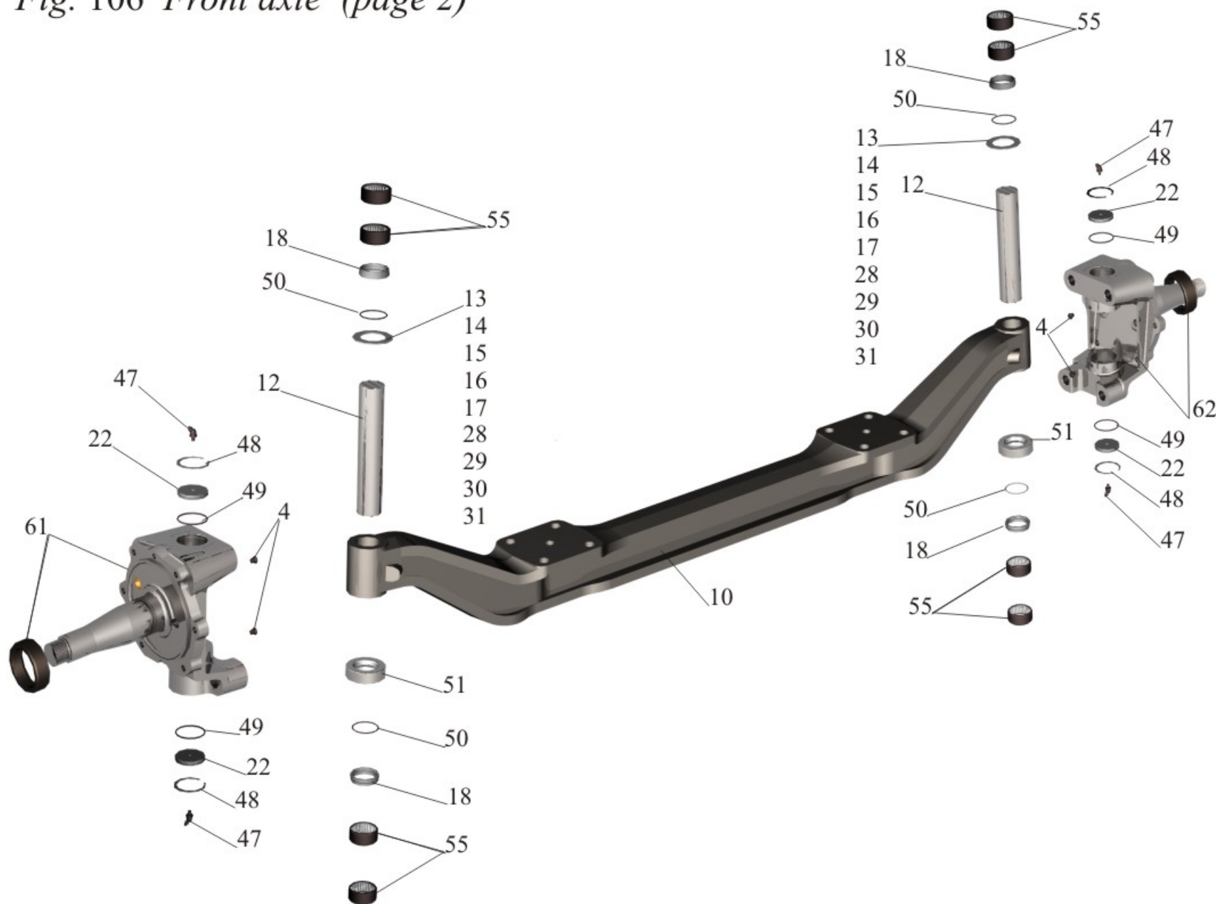
Fig. 106 Front axle (page 2)
