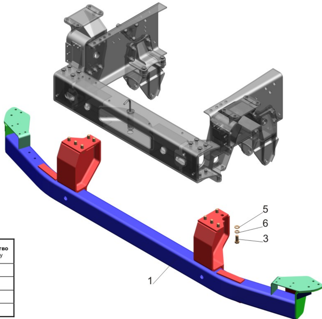
Fig. 89 Installation of front buffer stop 651608-2800030
