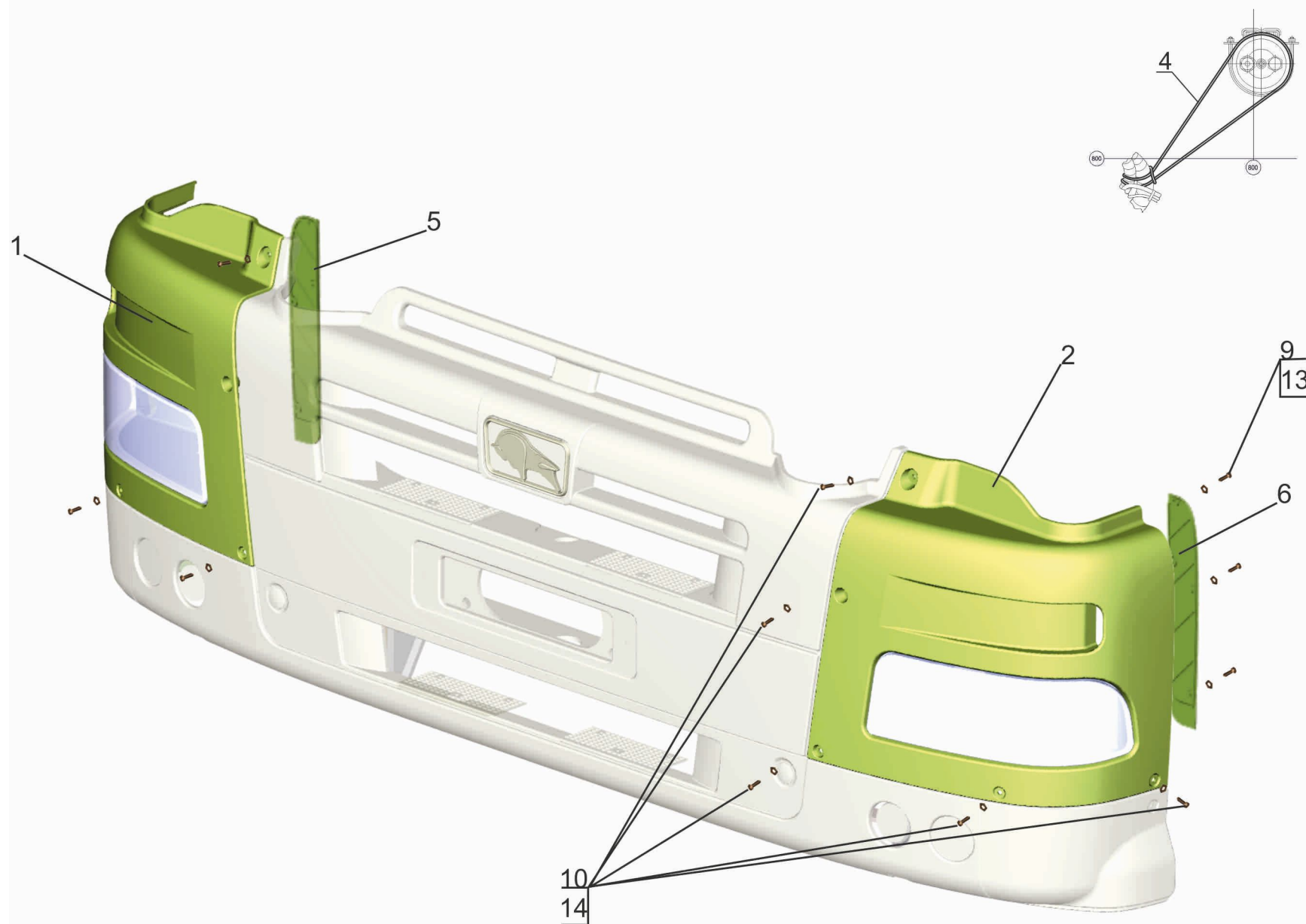
Fig. 85 Installation front bumper 643019-2800005
