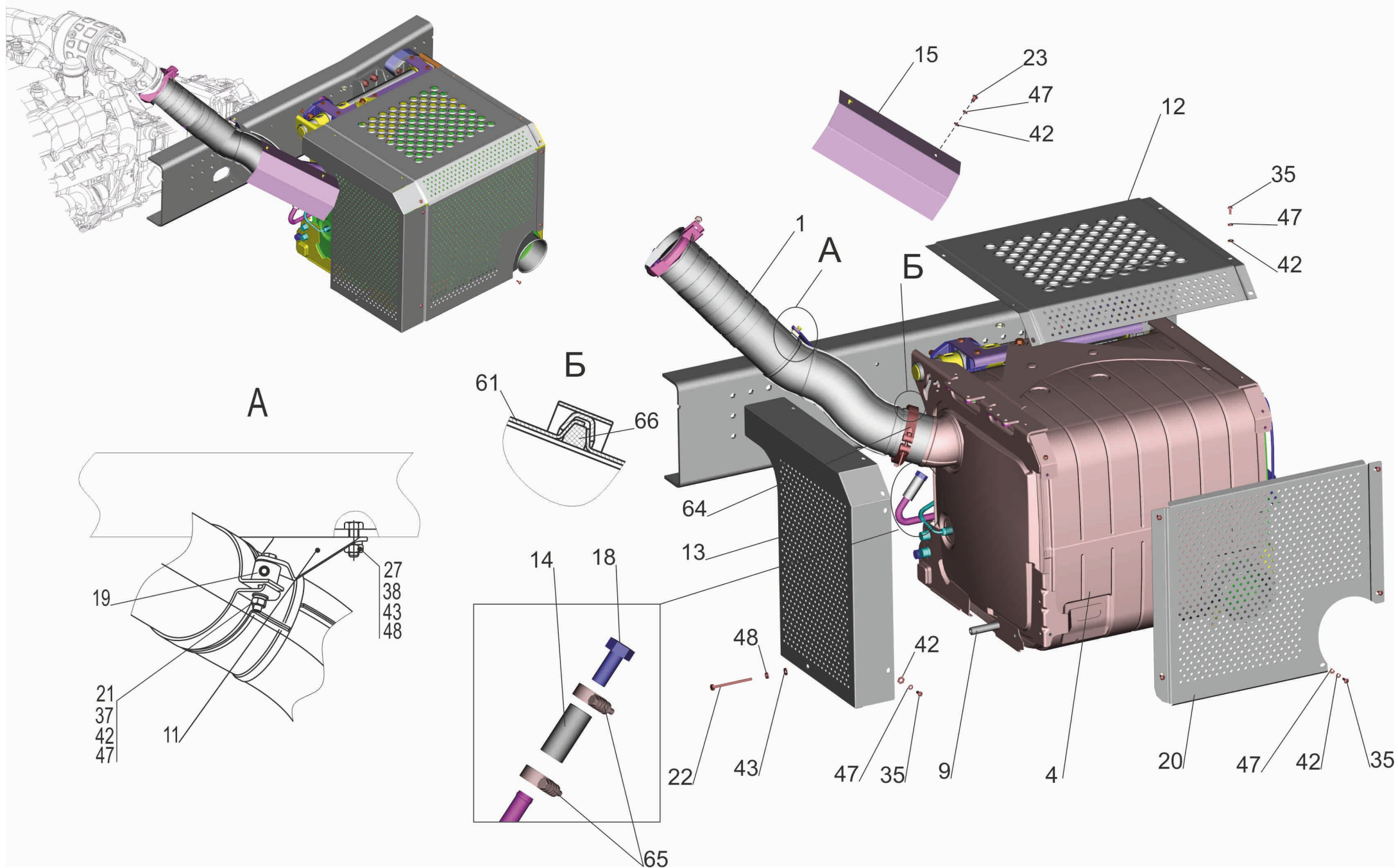
Fig. 24 Installing of gas release sistem 534019-1200001 (page 1)
