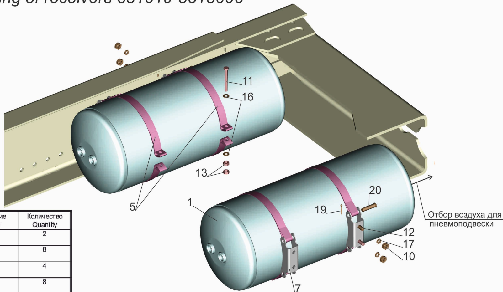
Fig. 165 Mounting of receivers 631019-3513006
