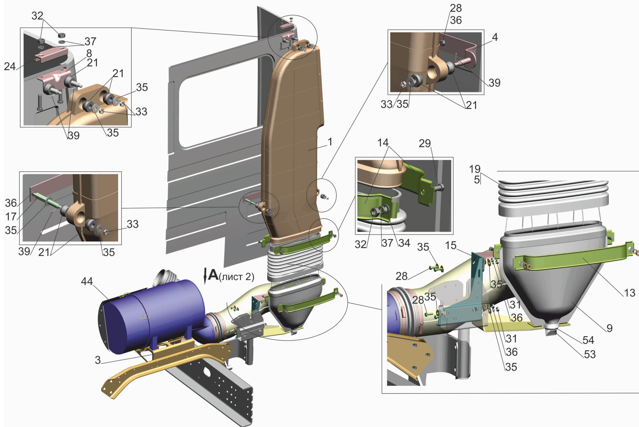
Fig. 22 Air filter mounting 544019-1109002-001 (page 1)
