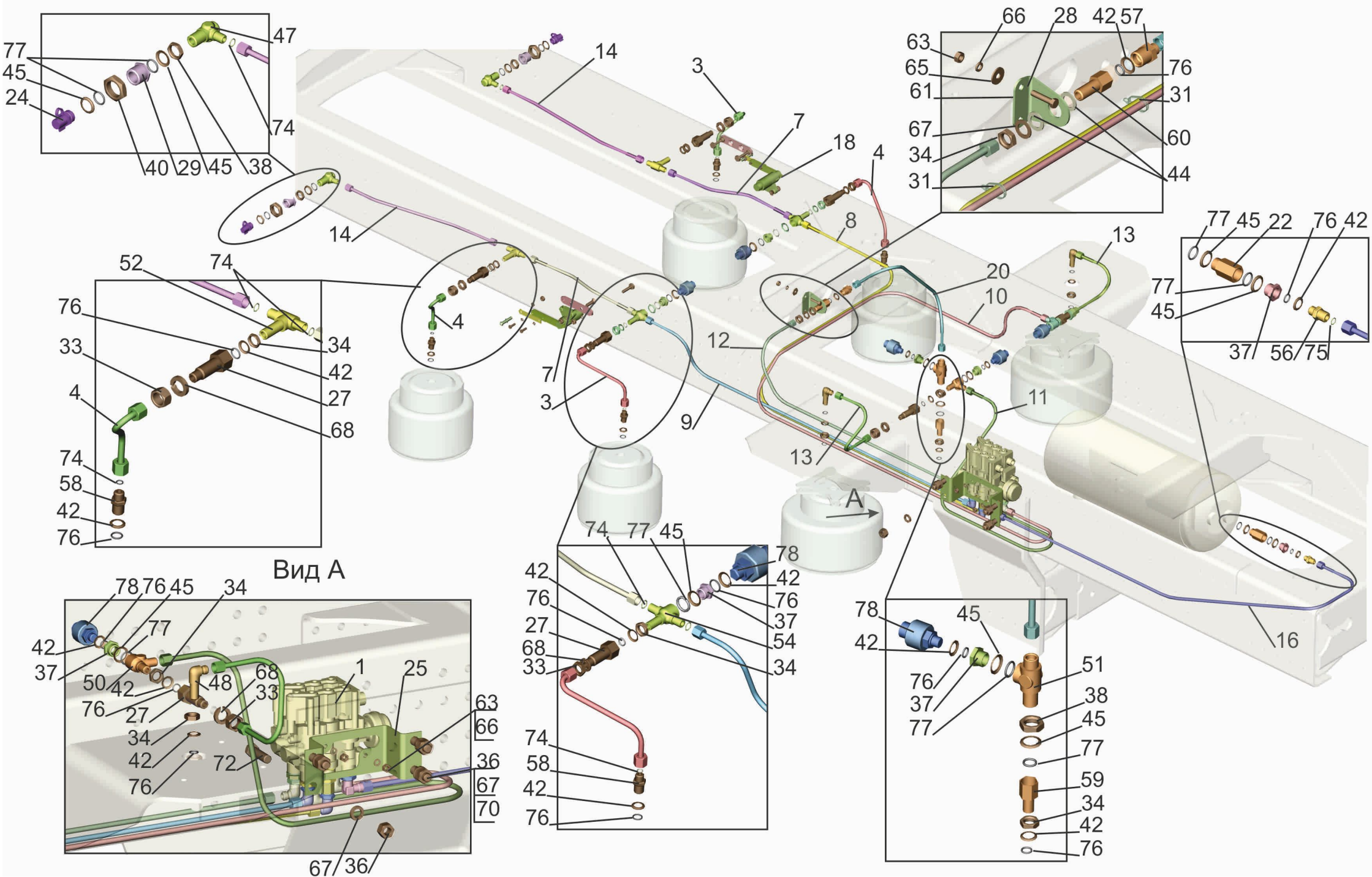
Fig. 109 Installation of pipelines ECAS 631019-2900018
