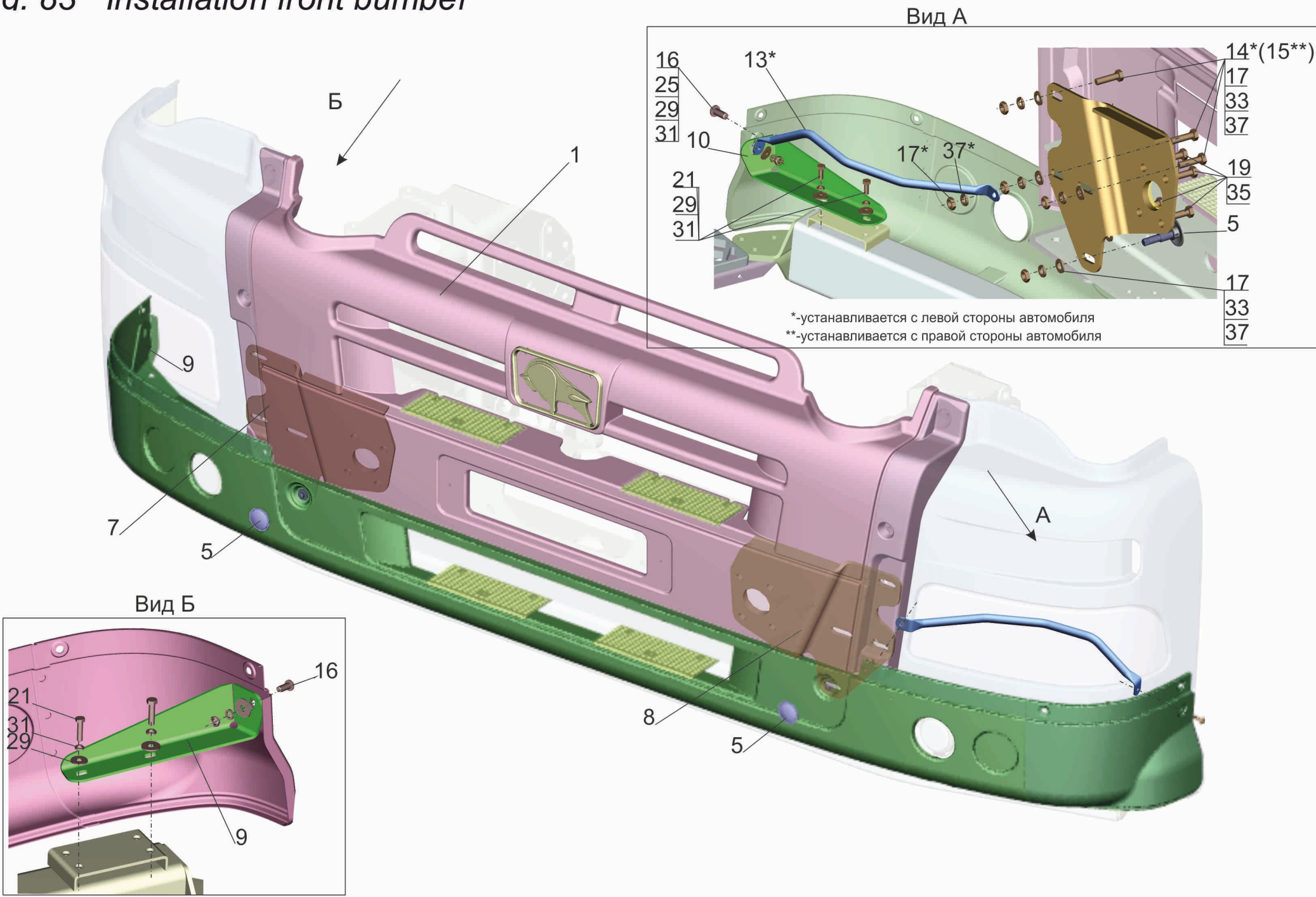
Fig. 83 Installation front bumper
