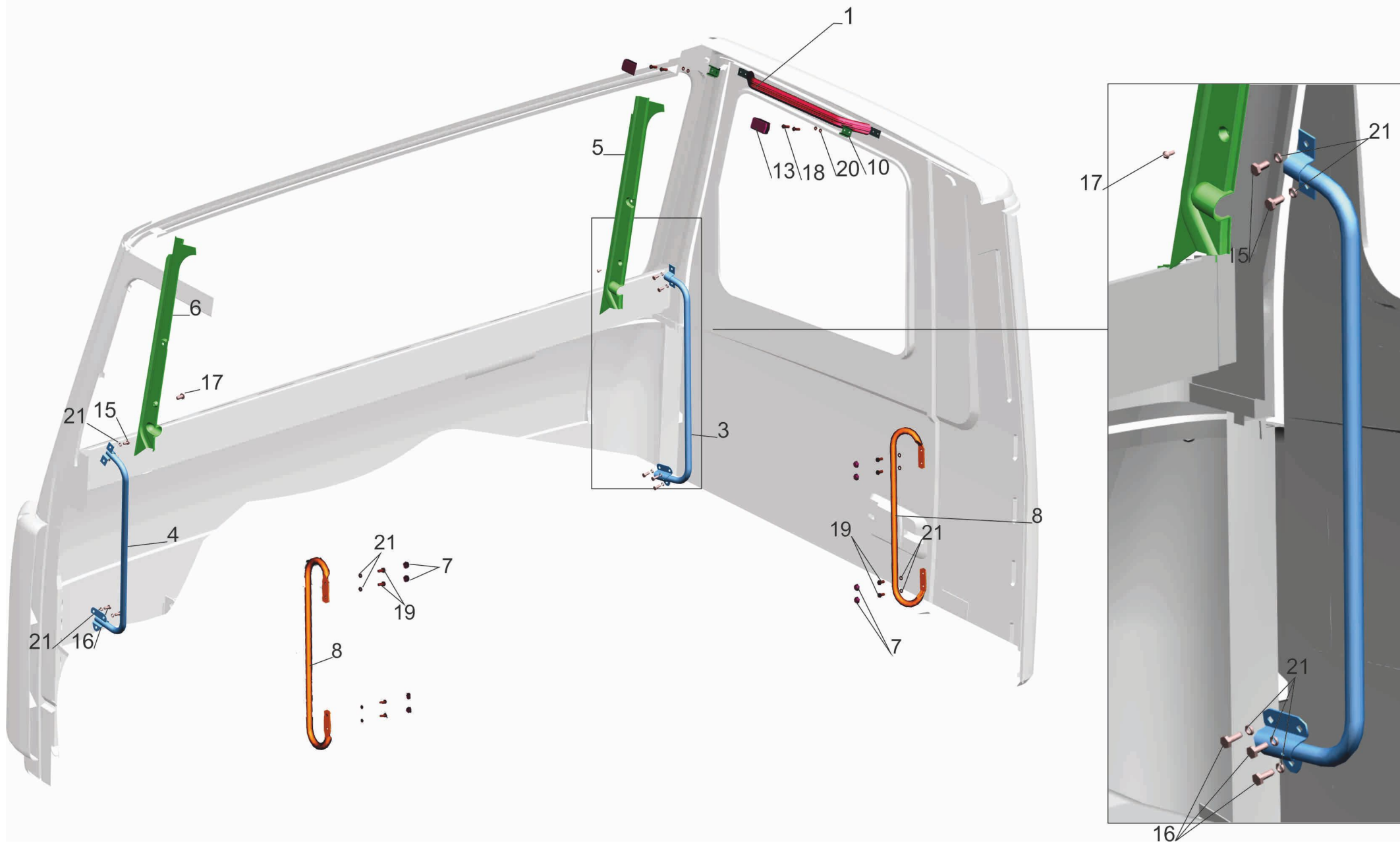
Fig. 267 Installation of grab handles in cab 6430-8200030
