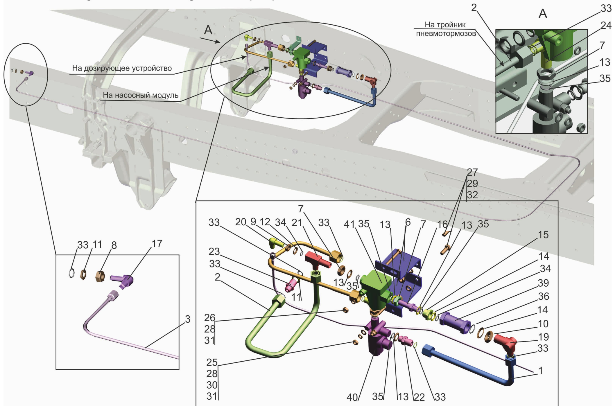
Fig. 38 Fastening device preparation air 544019-1401010
