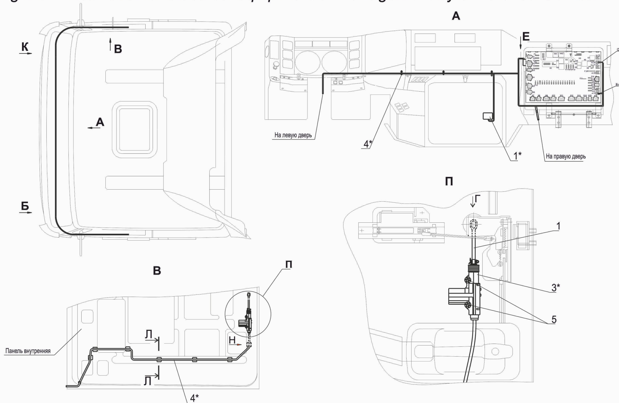
Fig. 201 Installation of electrical equipment of management by drive of central lock
