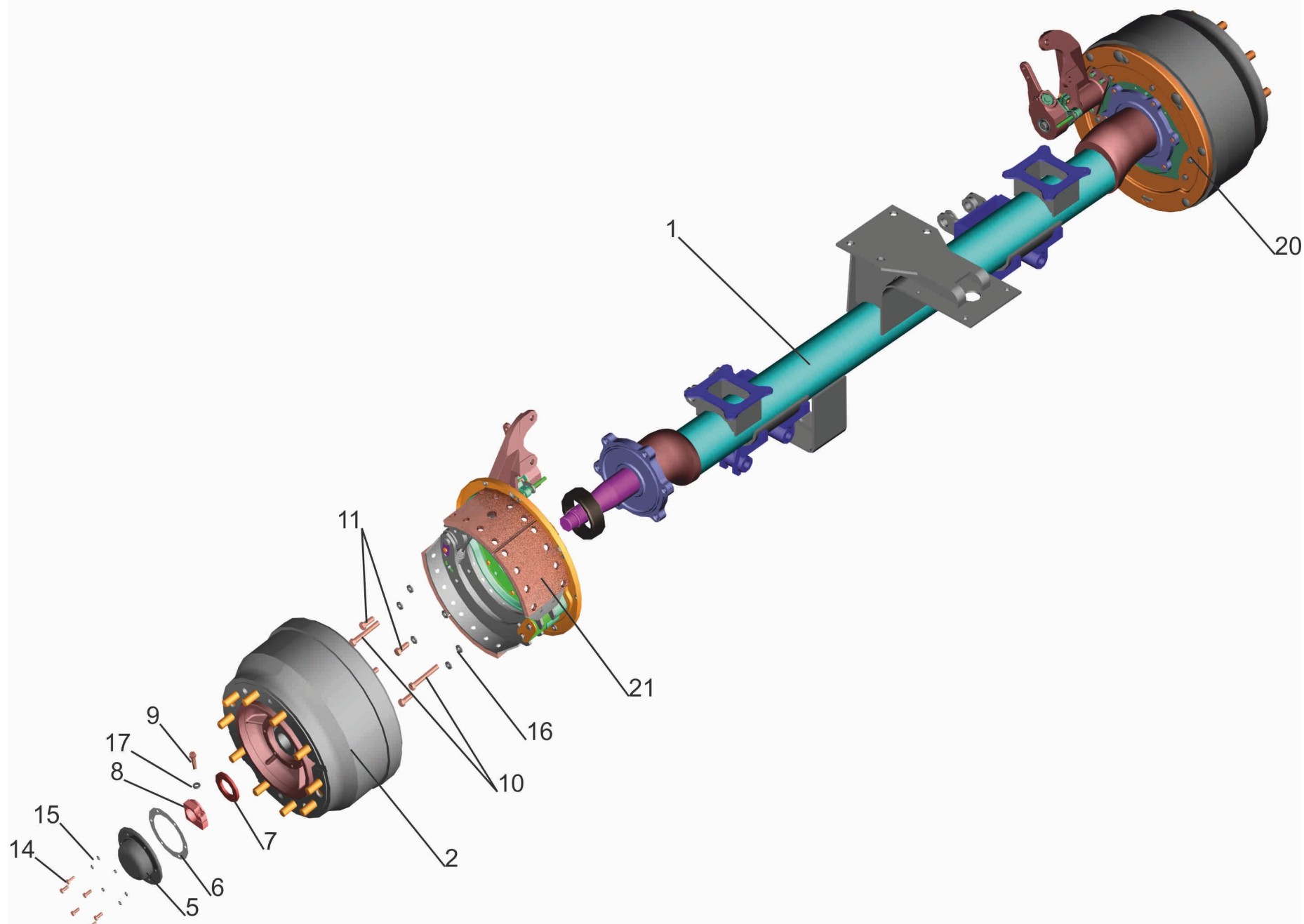
Fig. 113 Additional axle 631019-3000012-010
