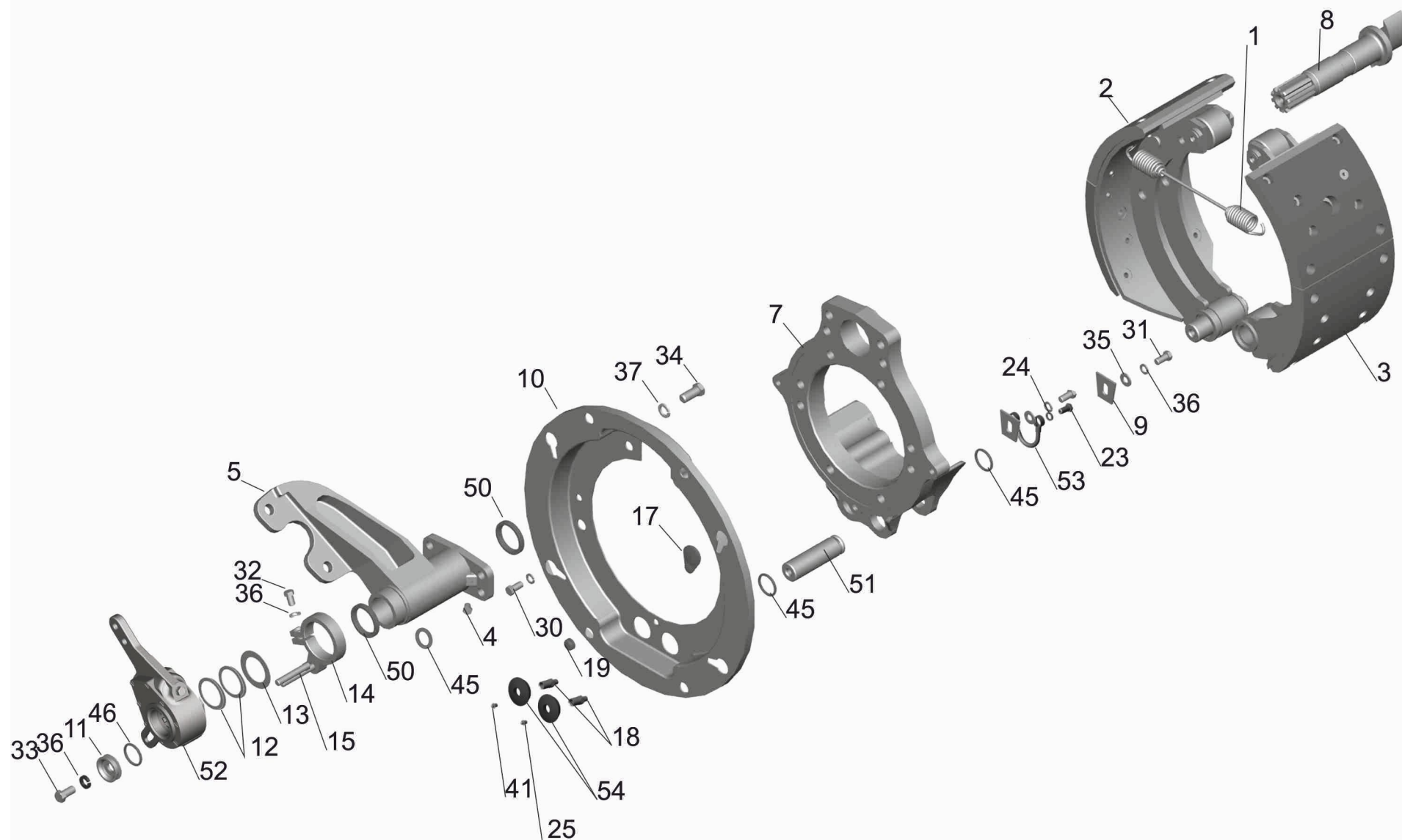
Fig. 118 Front brake 5440-3501004 (5440-3501005)
