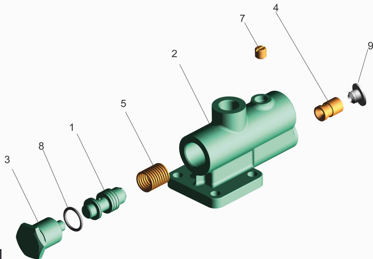
Fig. 160 Valve of expense of pressure 5336-3407260
