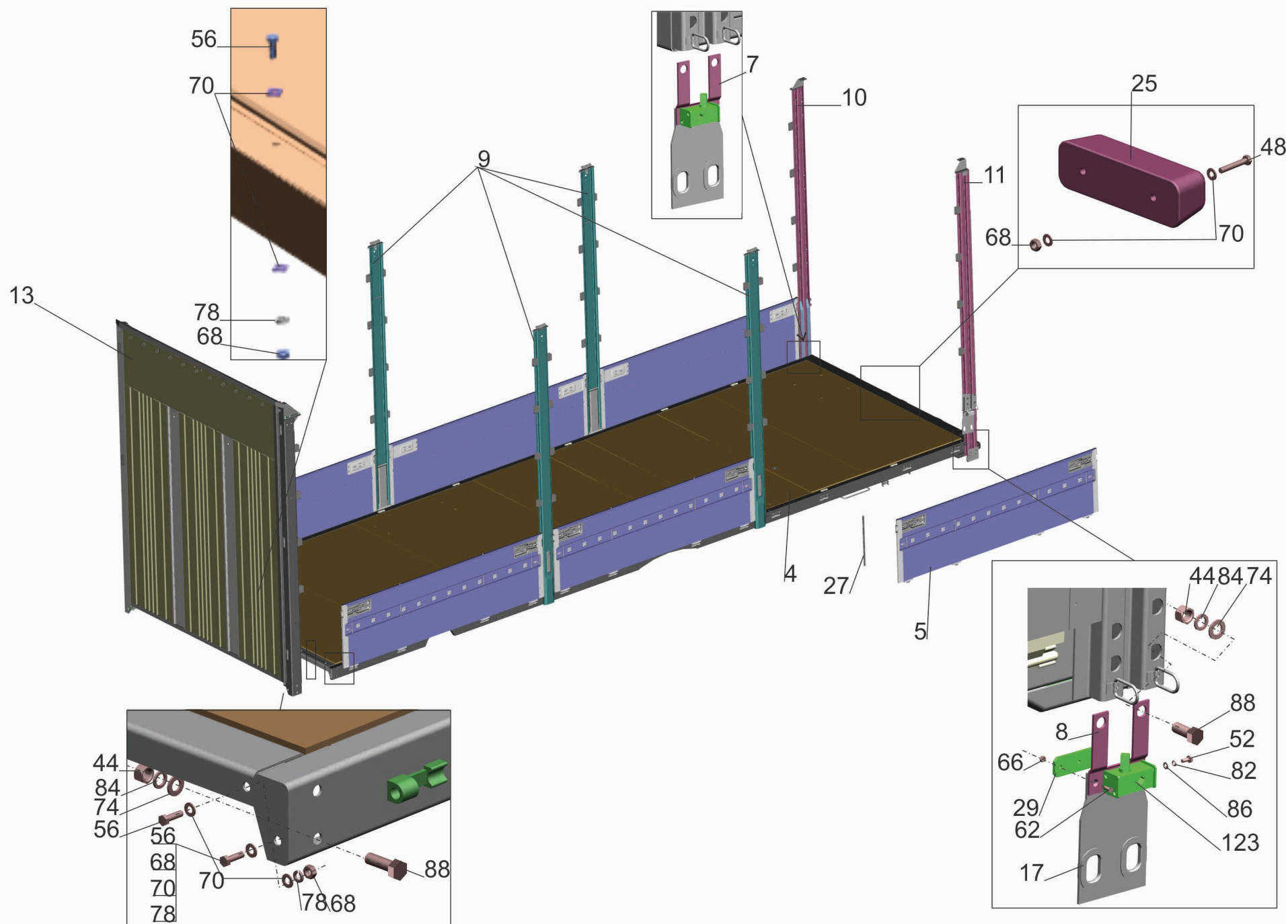
Fig. 318 Platform (sides and pillars) (page 2)
