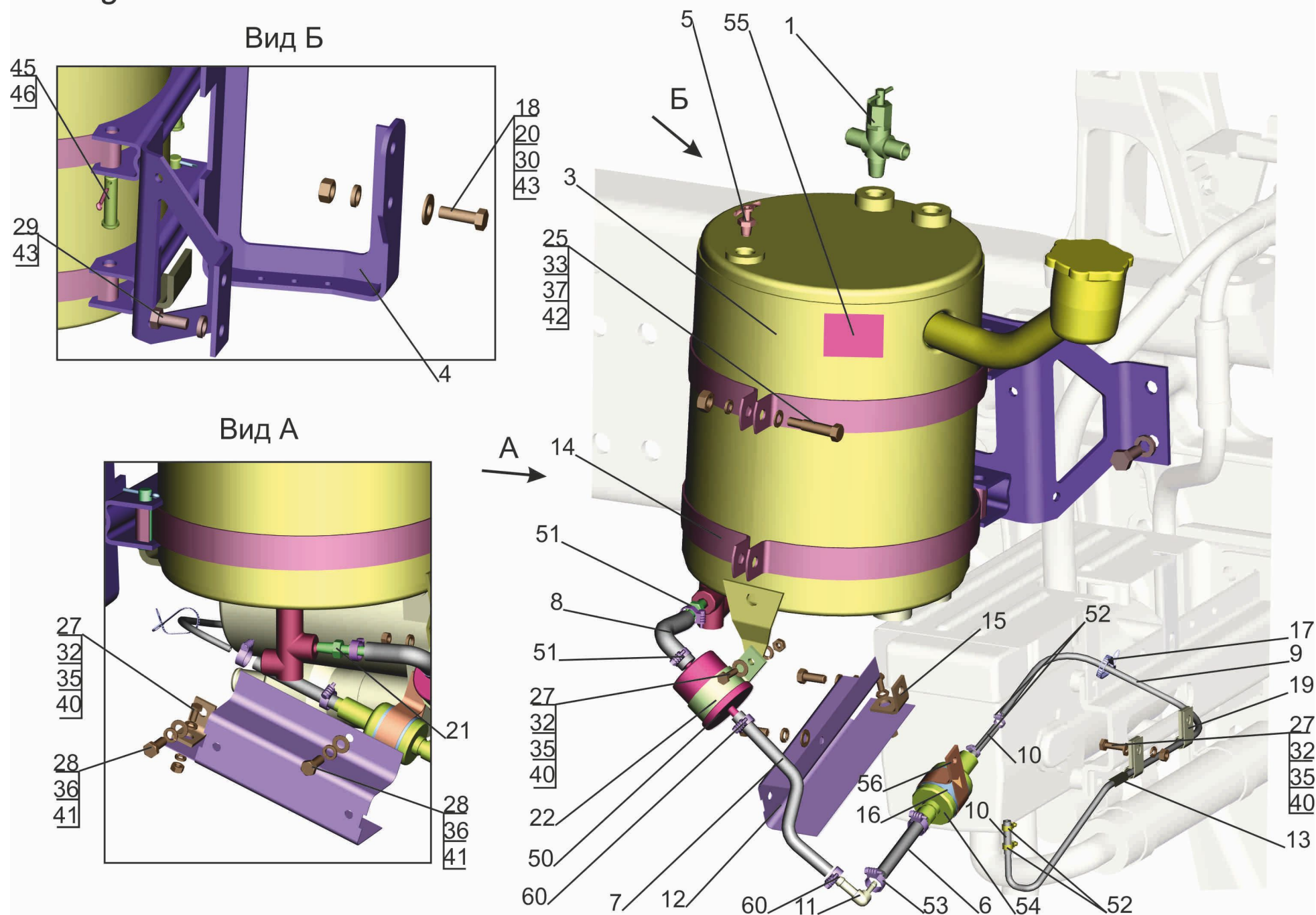
Fig. 6 Fuel lines of heater 544019-1015004
