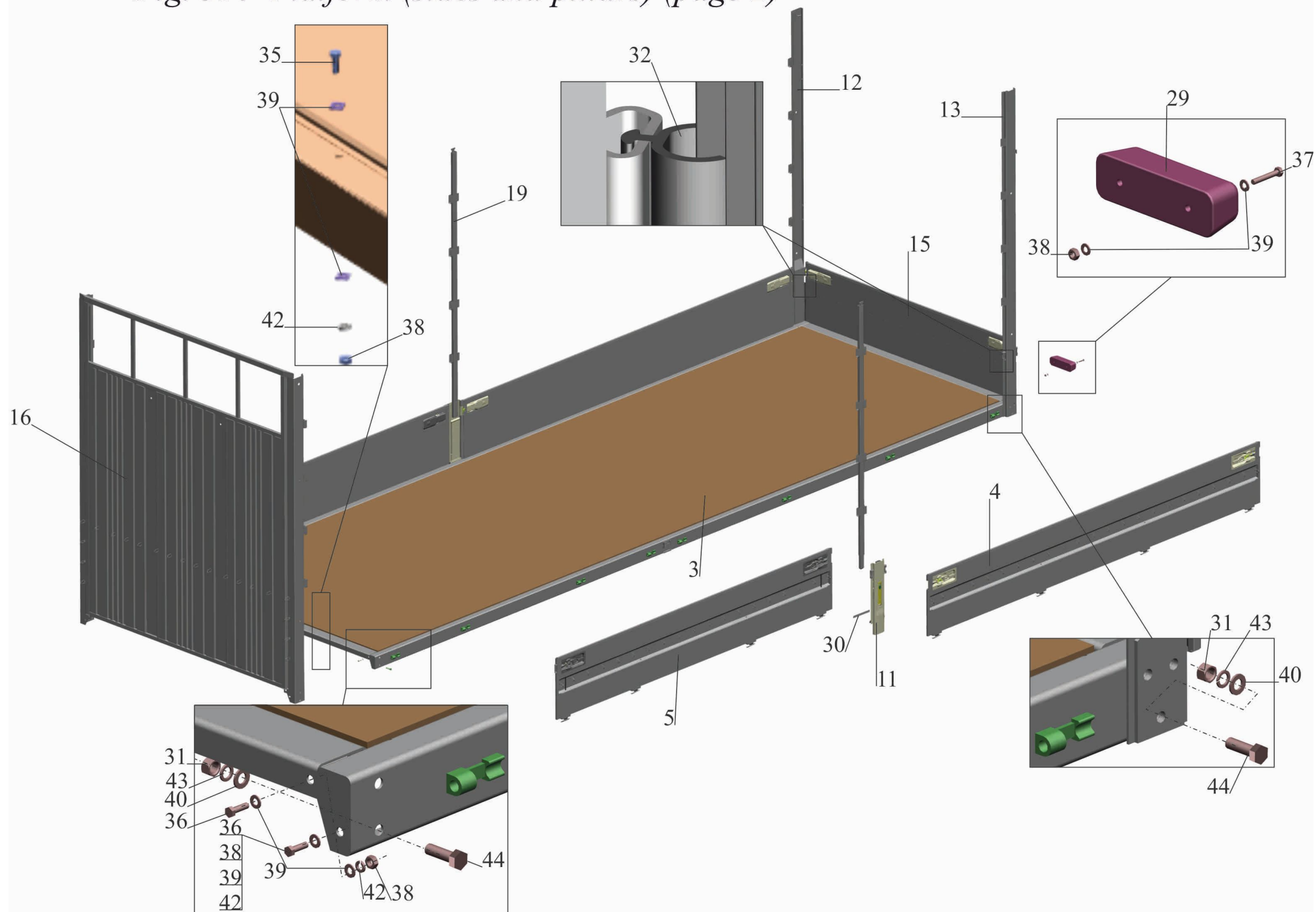
Fig. 314 Platform (sides and pillars) (page 2)
