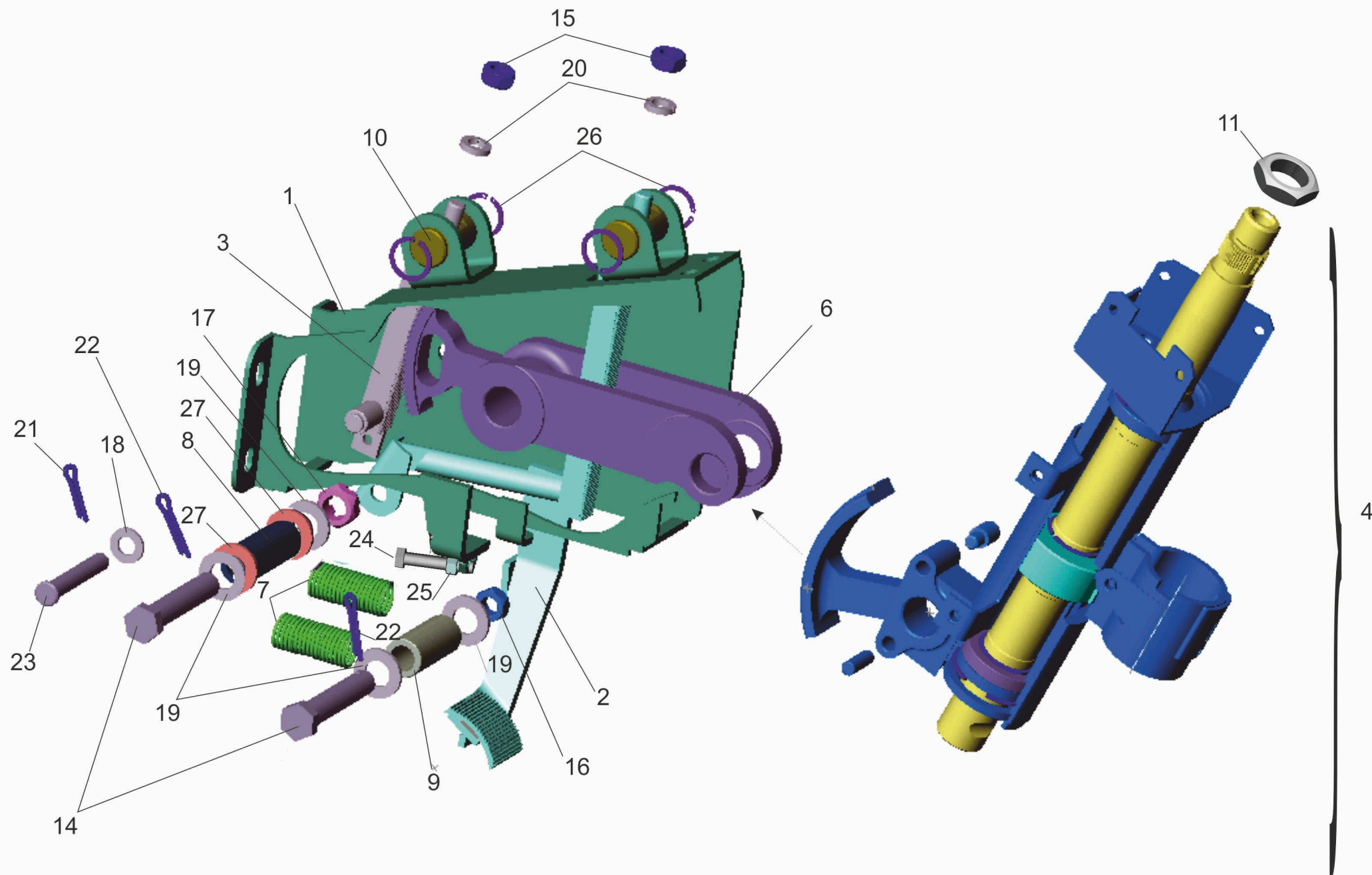
Fig. 149 Arm with a column 5440-3403008
