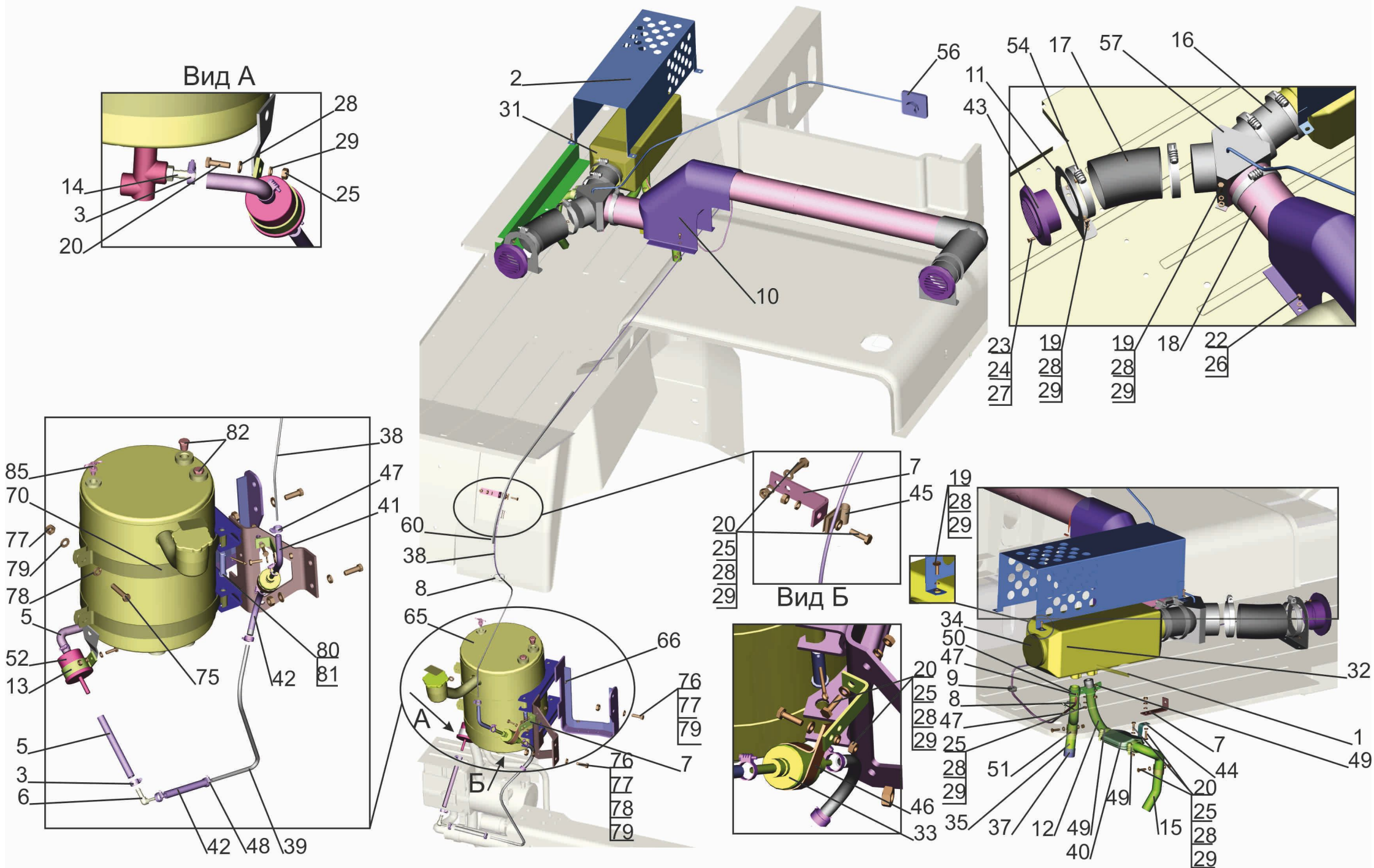
Fig. 292 Installation of the independent air heater 544019-8100002-010
