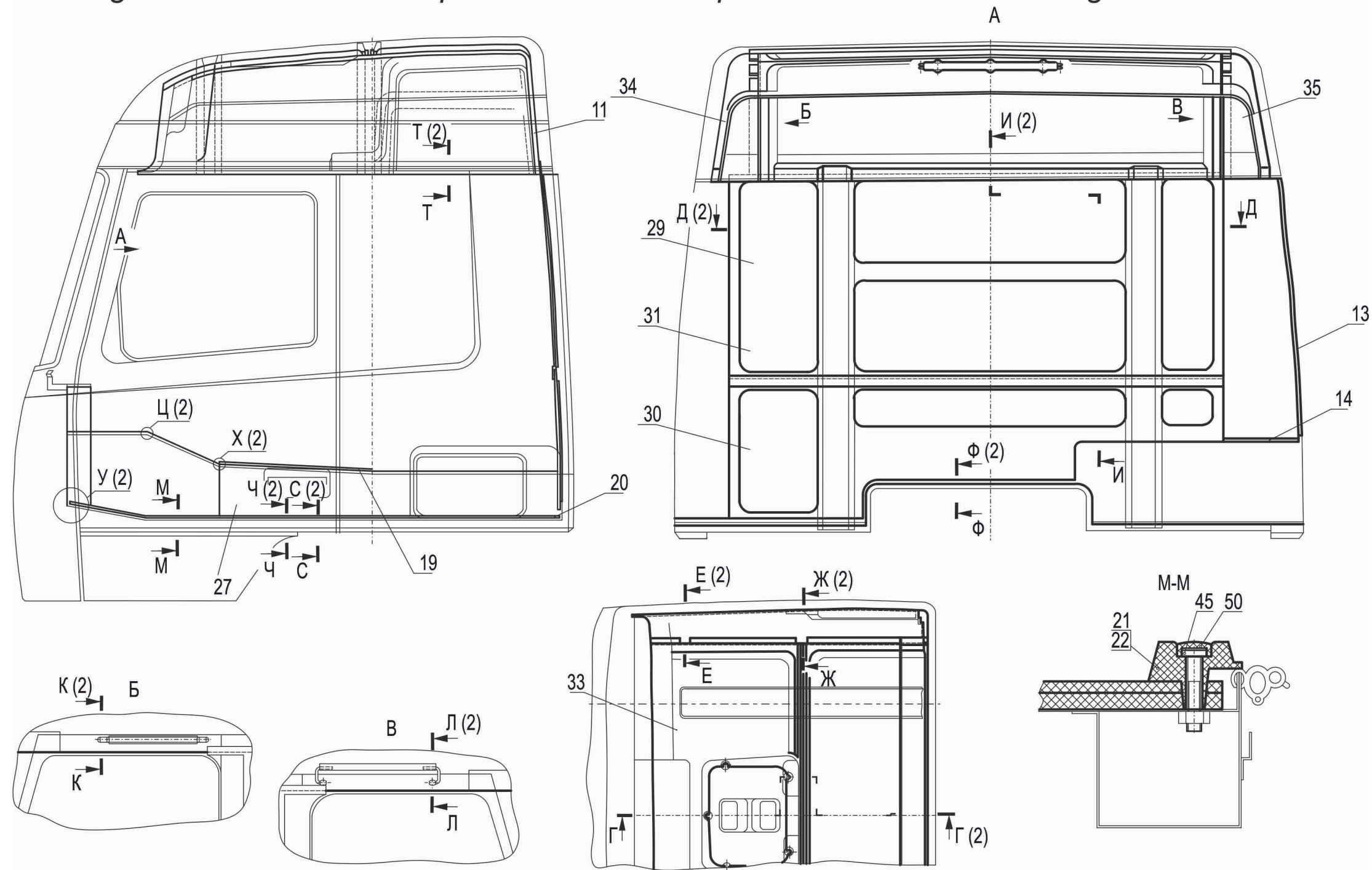
Fig. 240 Installation of upholsteries and carpets 643019-5000100 Page 1
