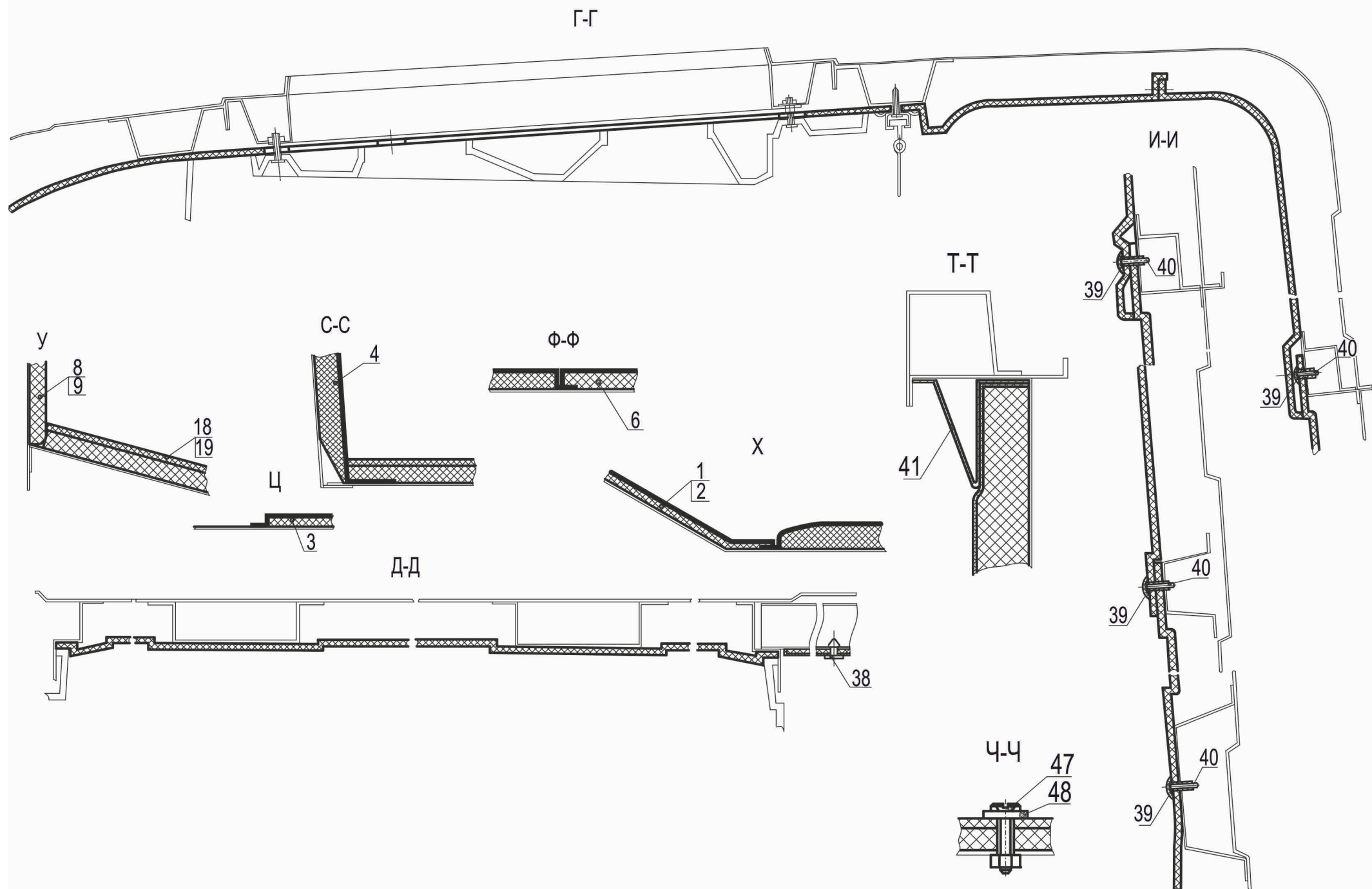
Fig. 240 Installation of upholsteries and carpets 643019-5000100 Page 2
