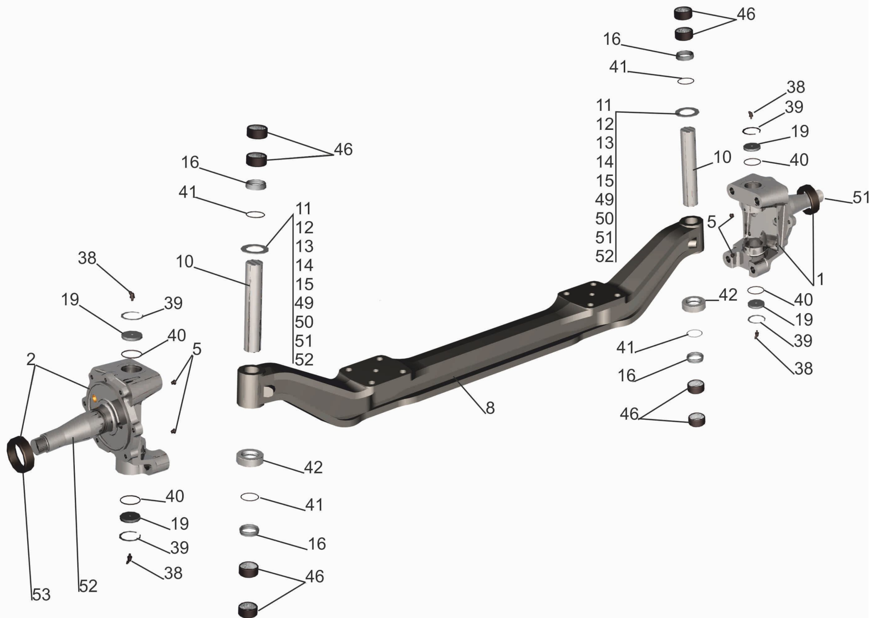
Fig. 121 Front axle 544019-3000015 (page 2)
