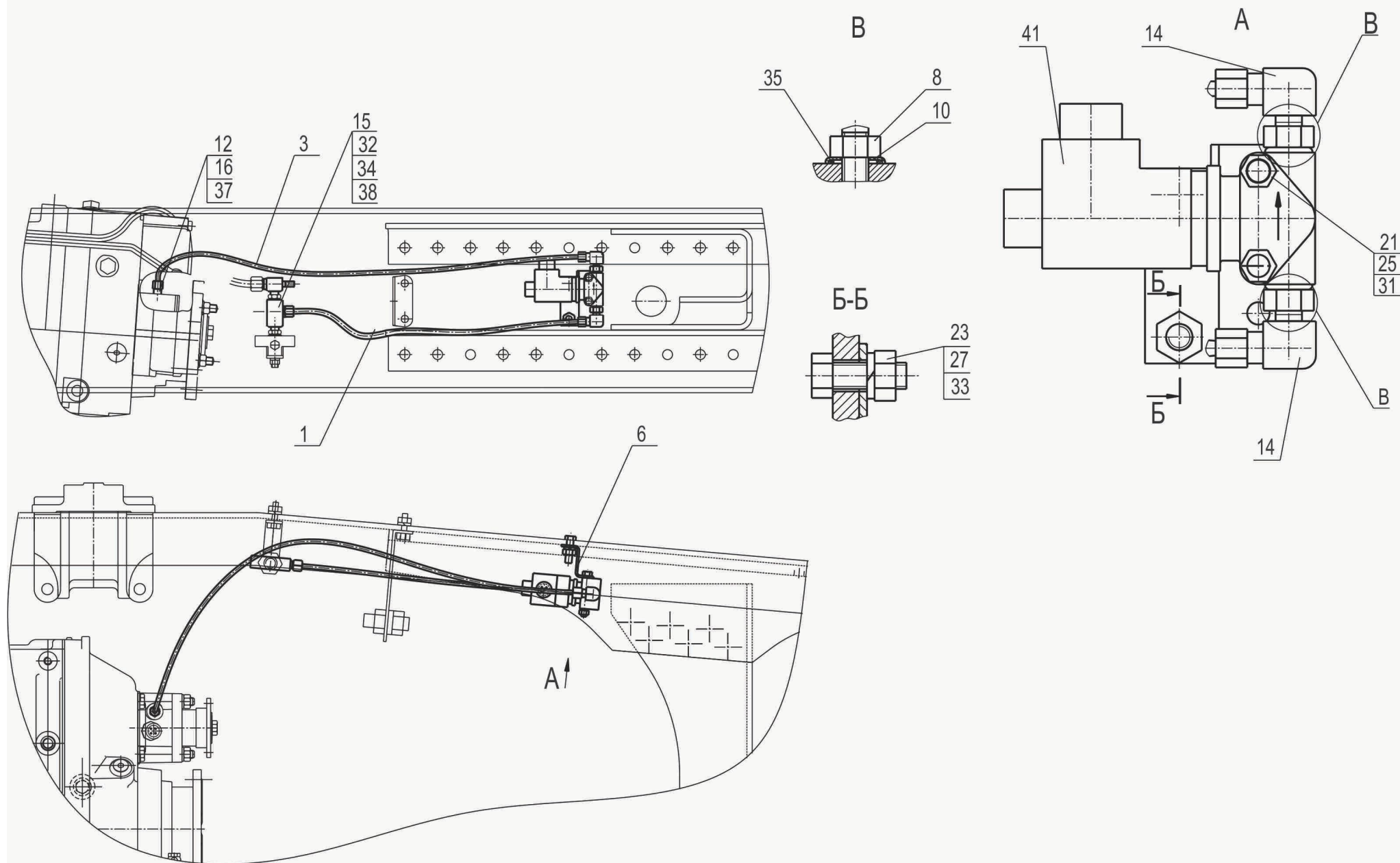
Рис. 225 Запитка коробки отбора мощности 631019-4200007-069 Fig. 225 Connection of power take-off gear box 631019-4200007-069
