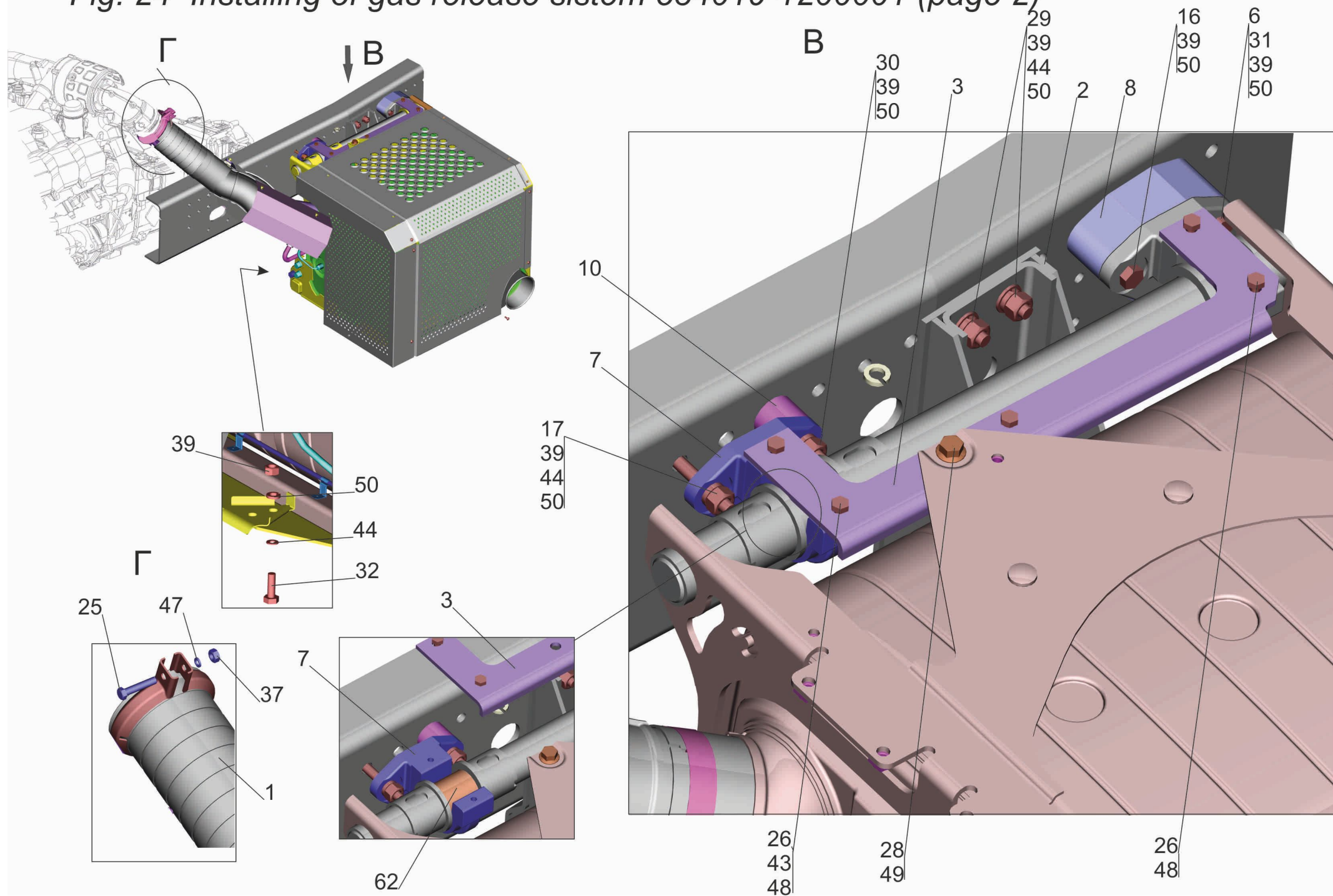
Fig. 24 Installing of gas release sistem 534019-1200001 (page 2)
