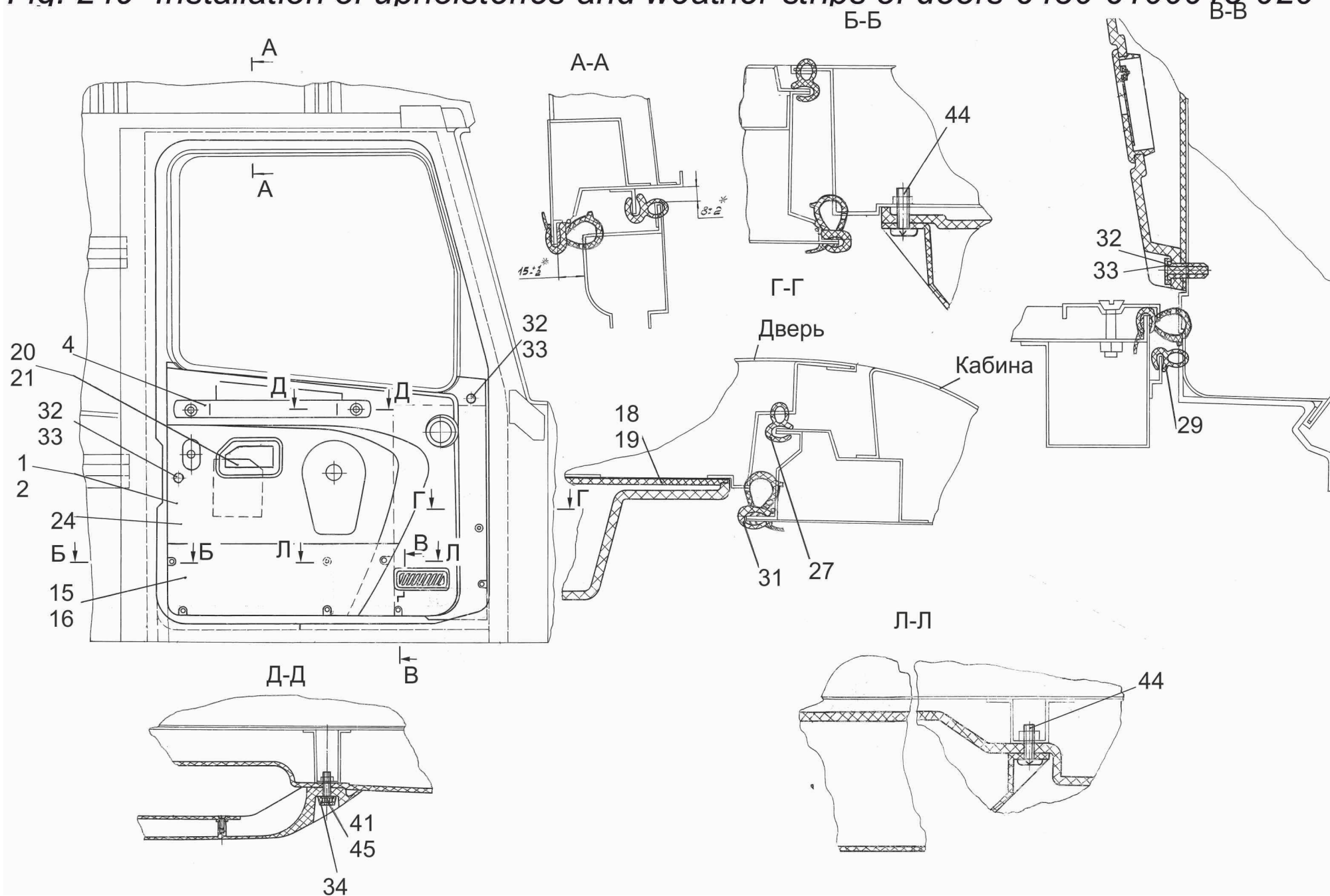
Fig. 249 Installation of upholsteries and weather strips of doors 6430-6100015-020
