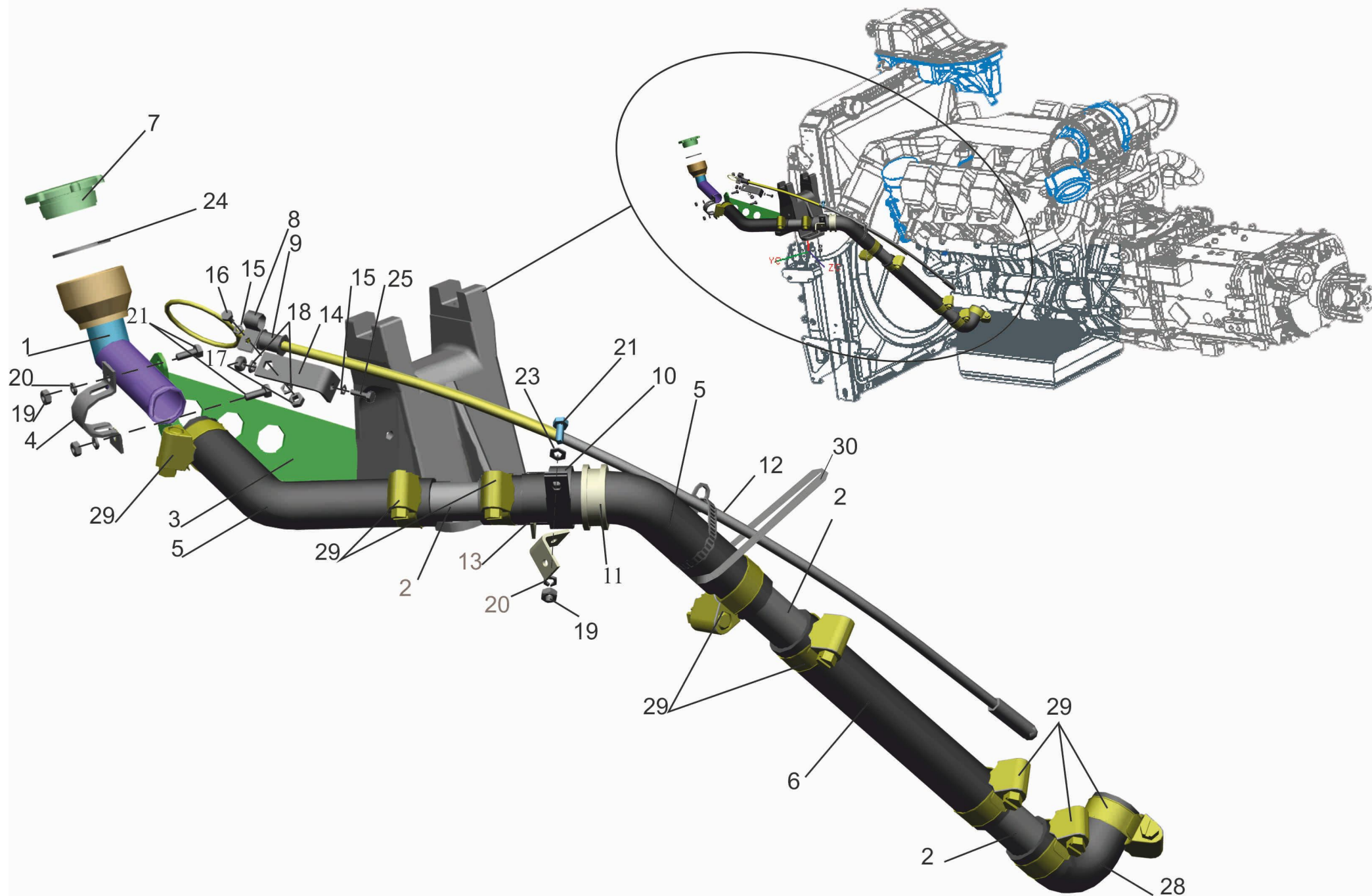
Fig. 4 Installation of system of oil priming and its level checking 544019-1018002
