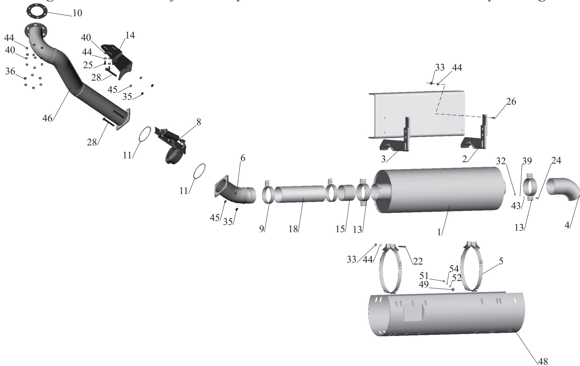
Fig. 21 Installation of exhaust system 551605-1200001-054 without body heating
