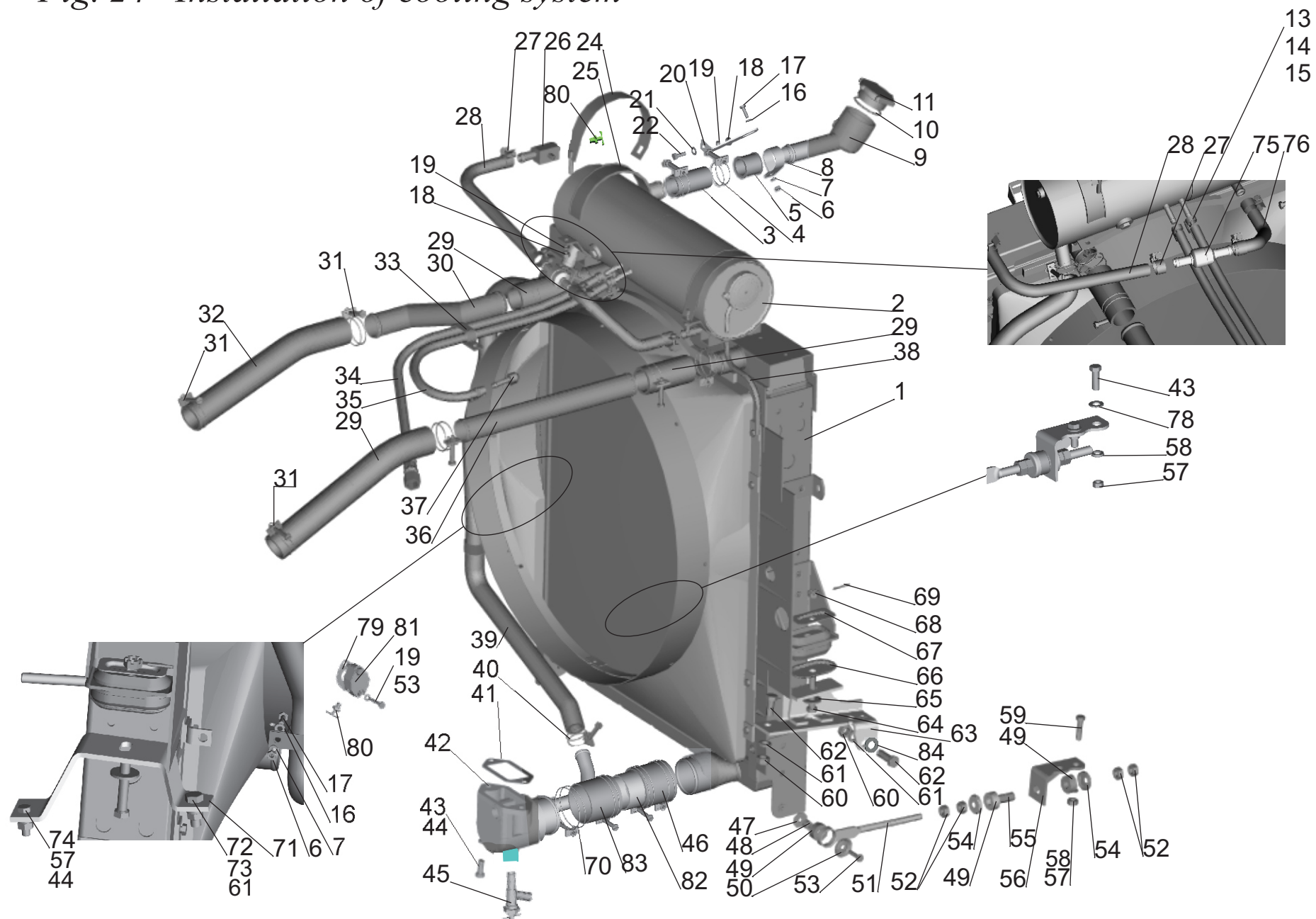
Fig. 24 Installation of cooling system
