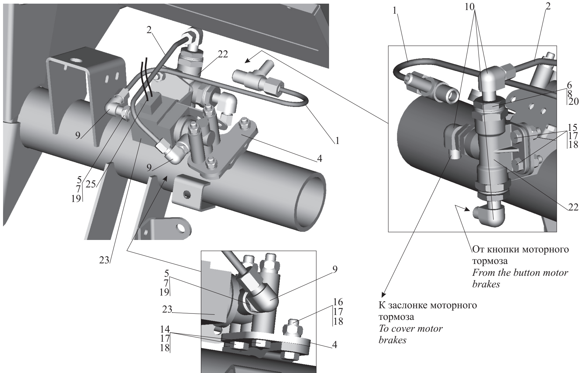
Fig. 17 Drive of switching engine 551605-1115004(-700)
