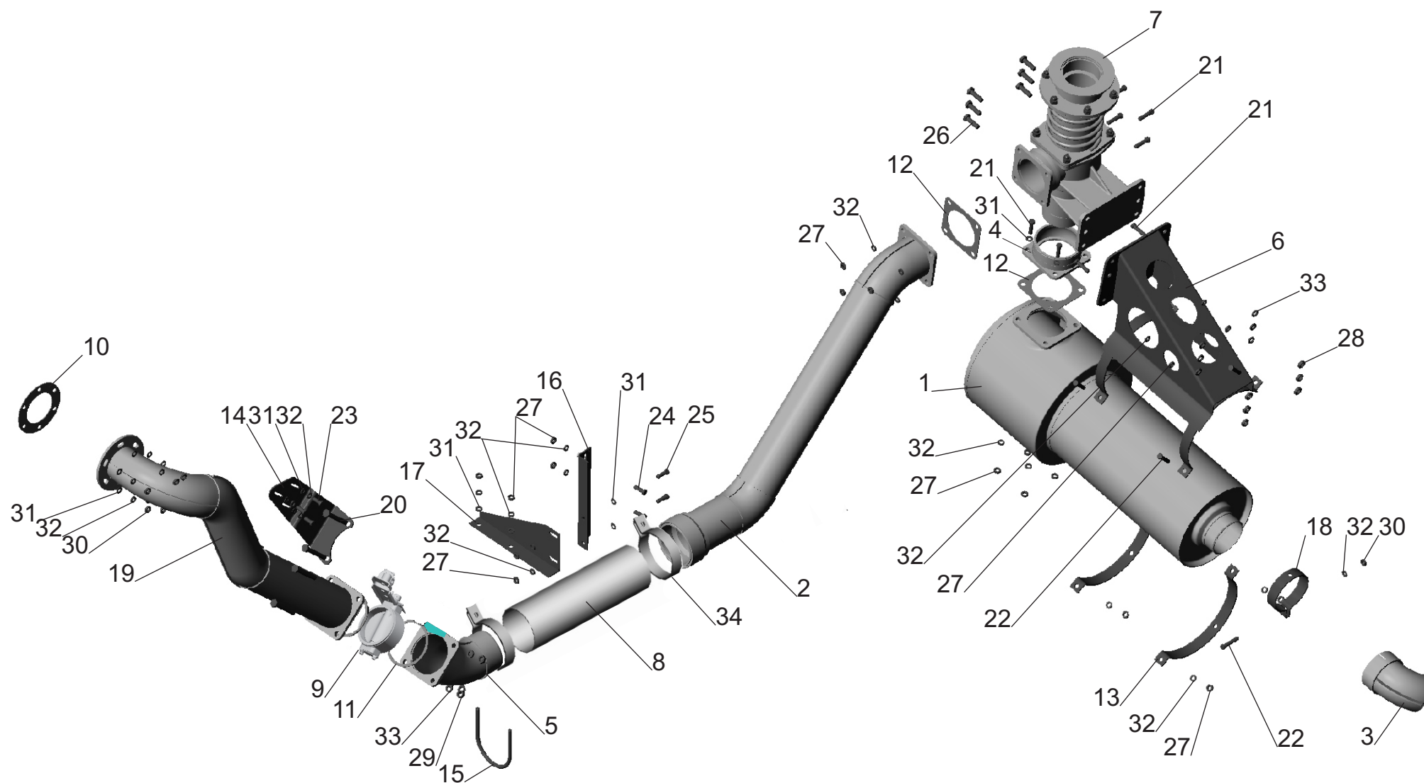
Fig. 20 Installation of exhaust system 551605-1200001-004 with body heating
