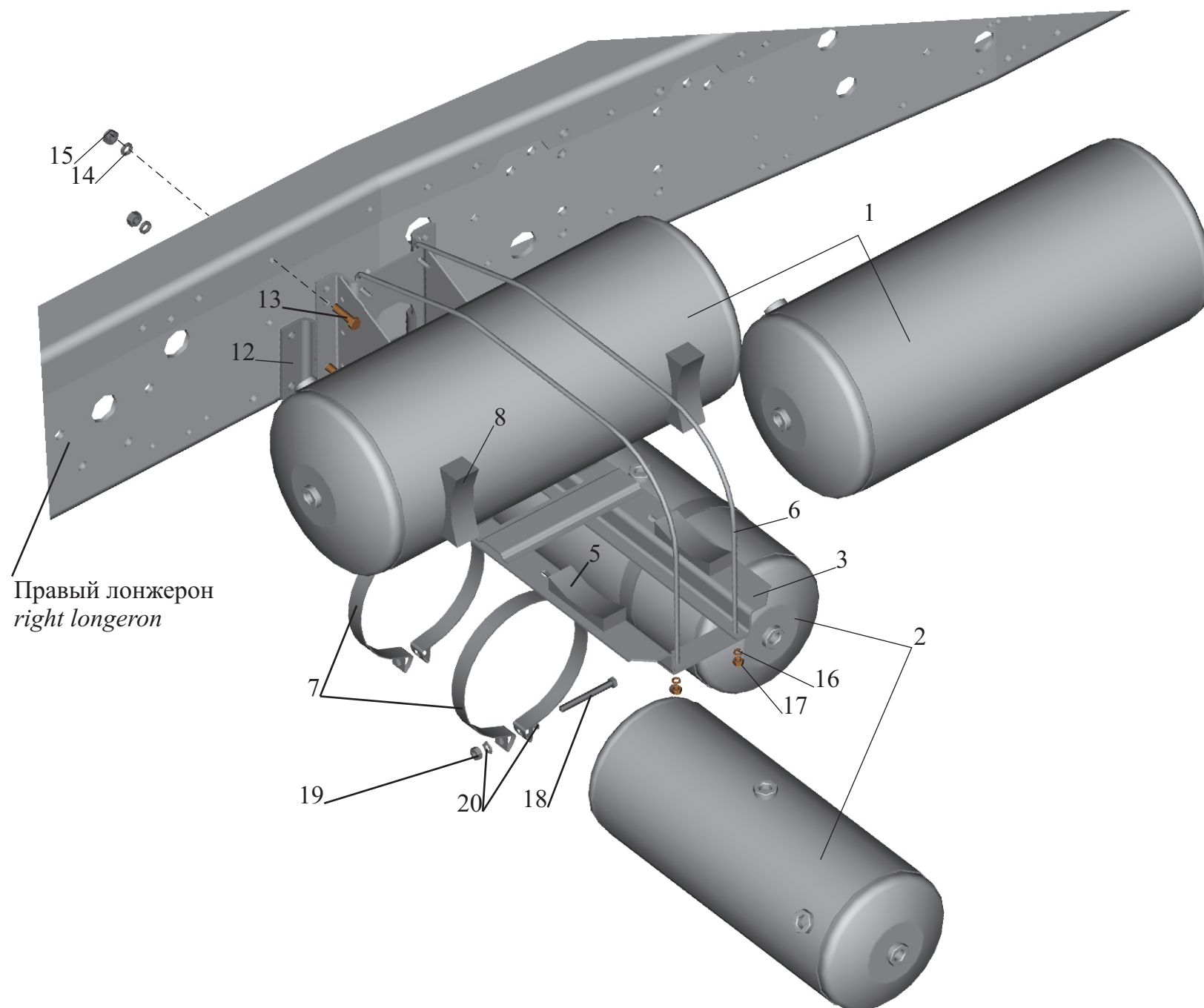
Fig. 104 Installation of receivers 551605-3513004
