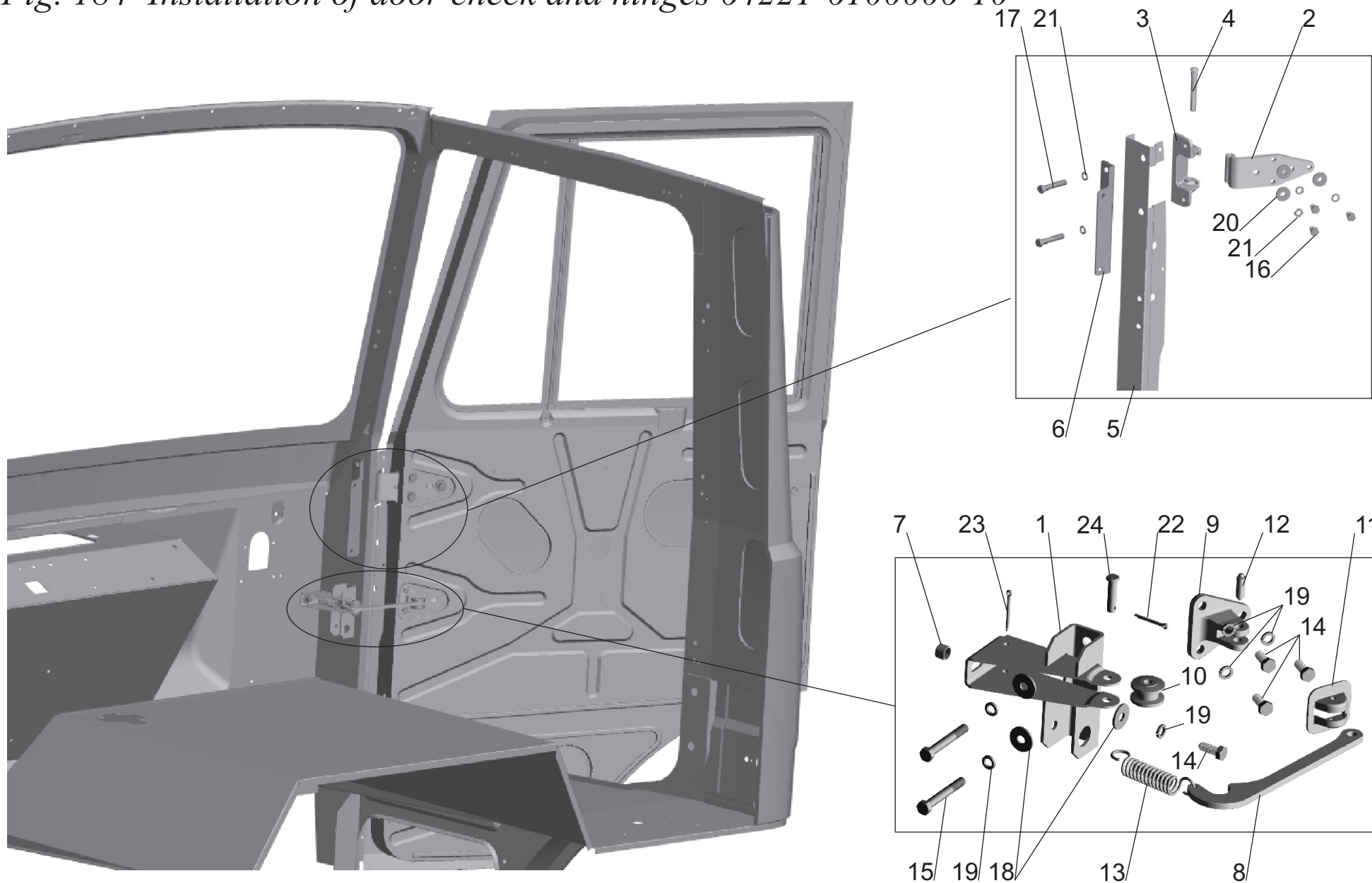
Fig. 184 Installation of door check and hinges 64221-6100006-10
