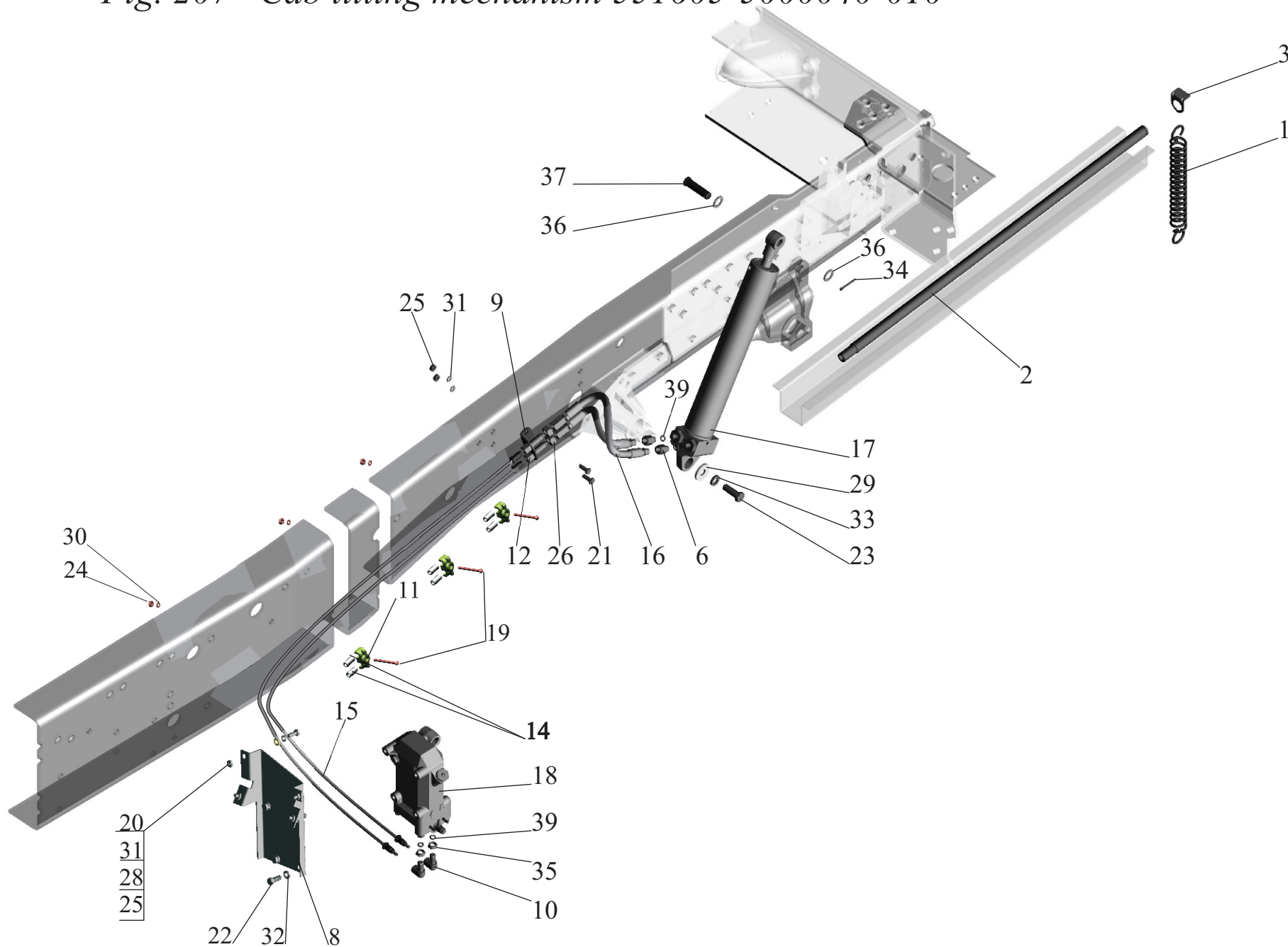
Fig. 207 Cab tilting mechanism 551605-5000040-010
