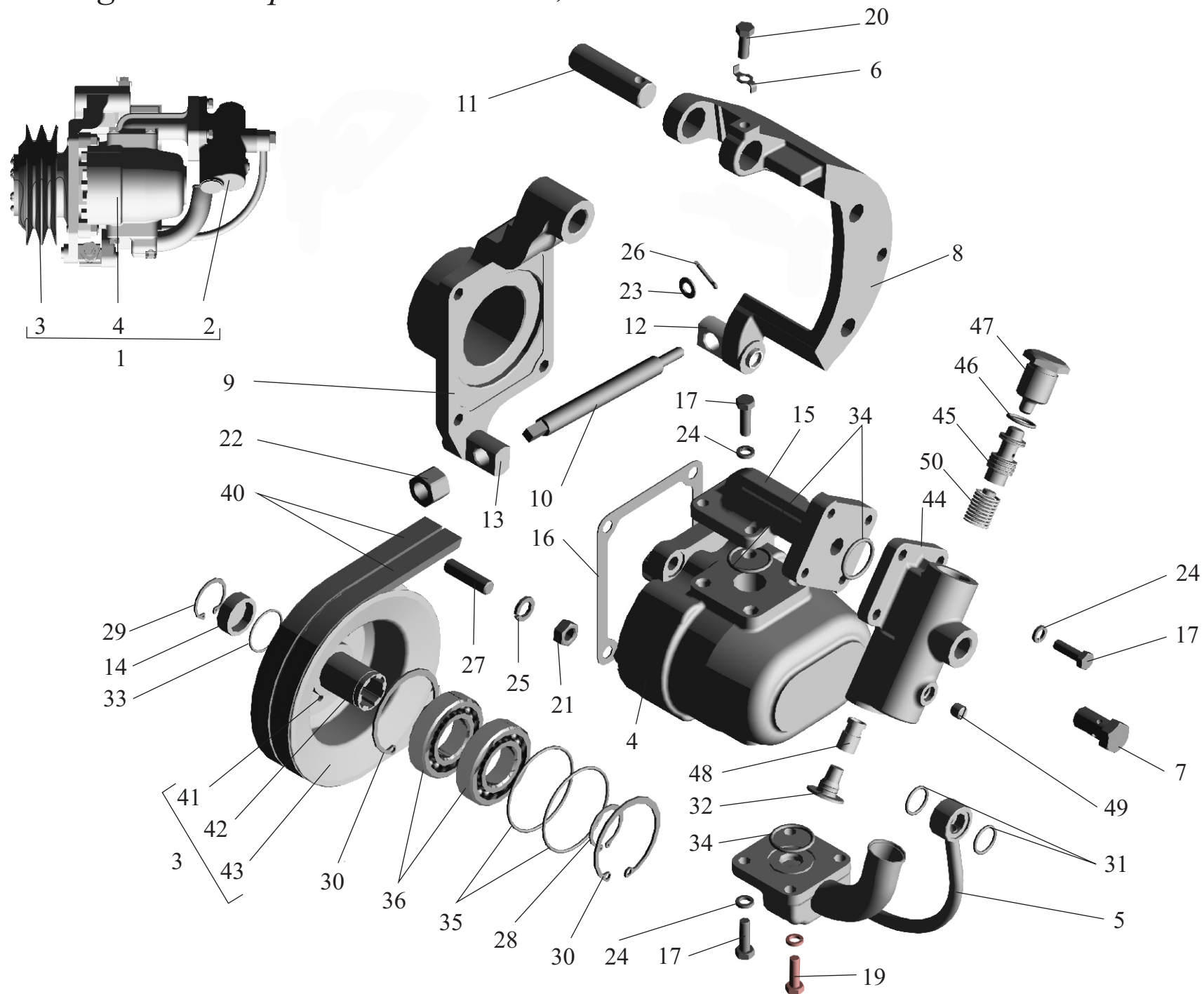
Fig. 92 Pump 543240-3407010, 543240-3407010-700
