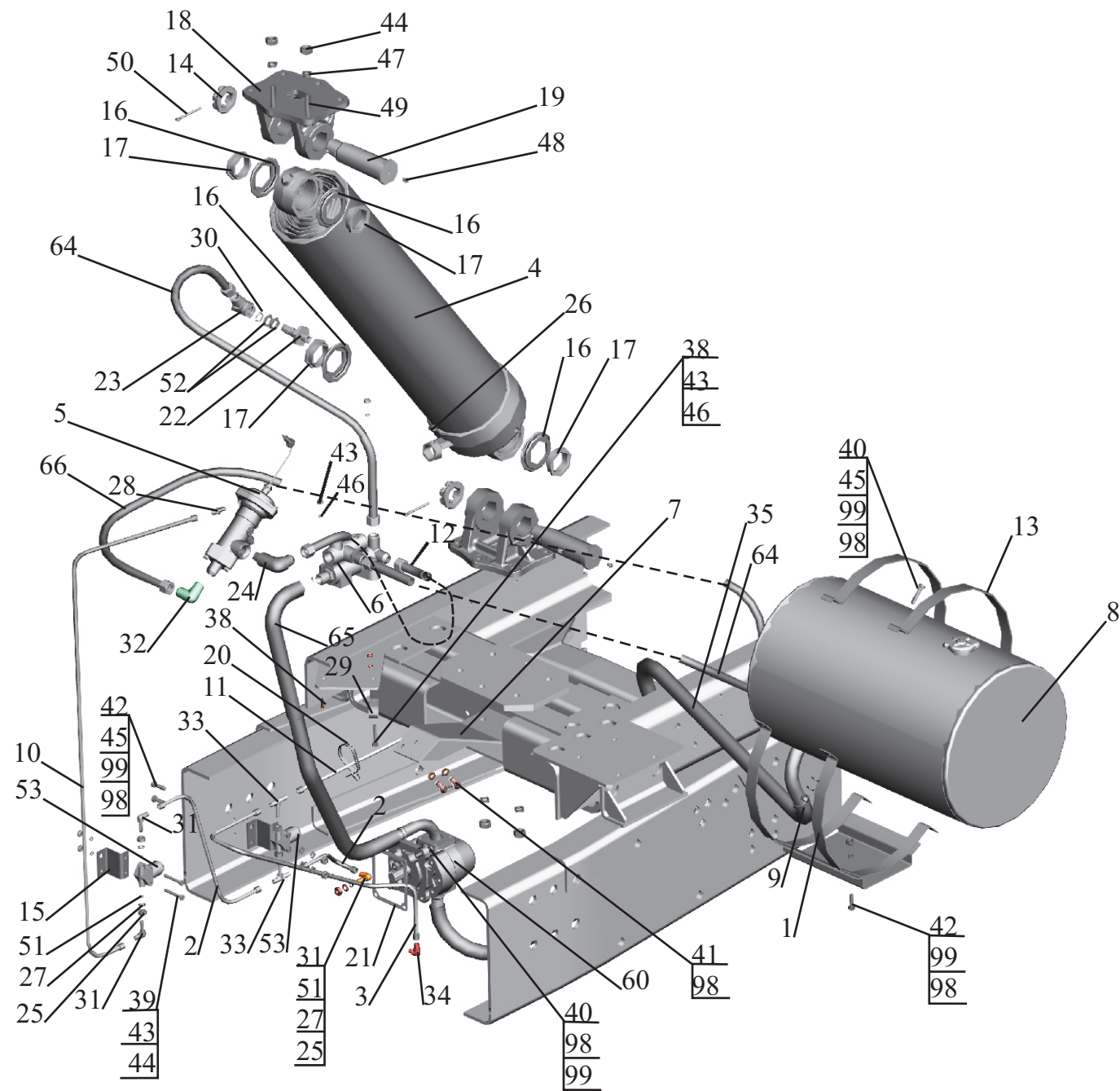
Fig. 243 Installation of hydroequipment
