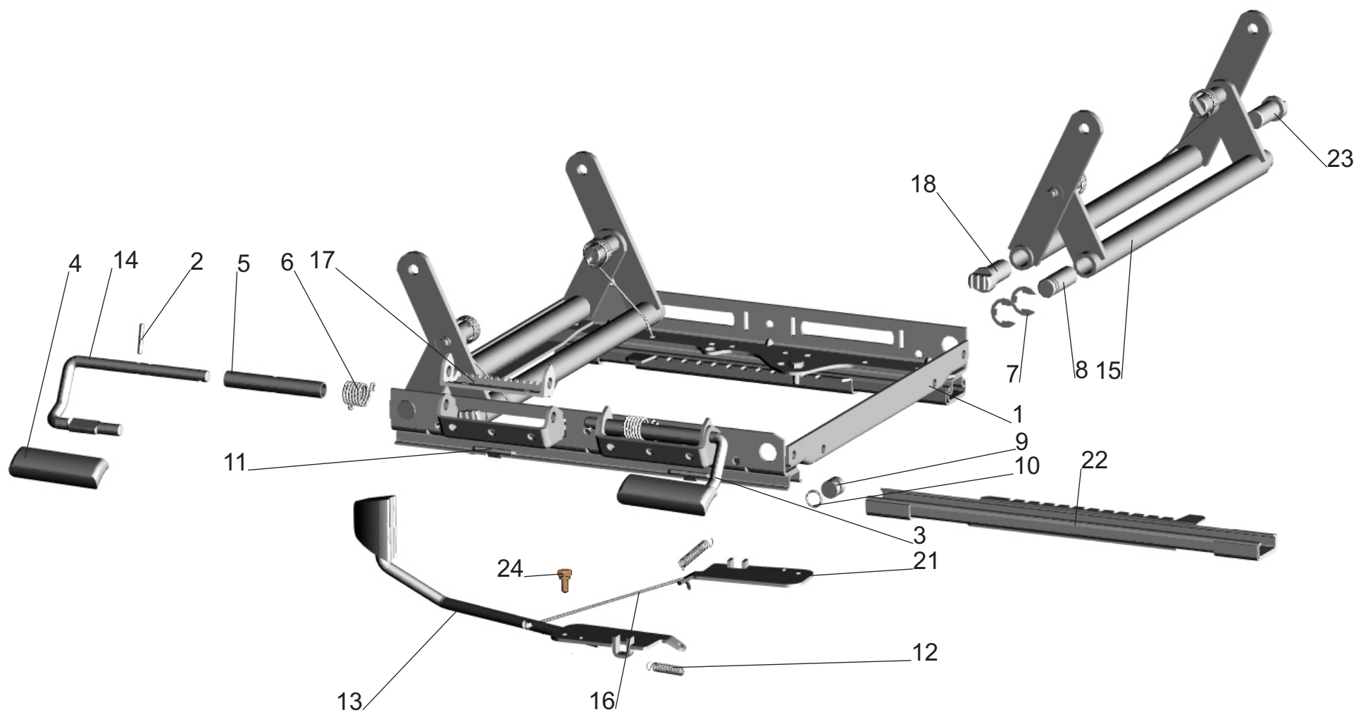
Fig. 194 Adjusting mechanisms of seat height 6430-6804100-010
