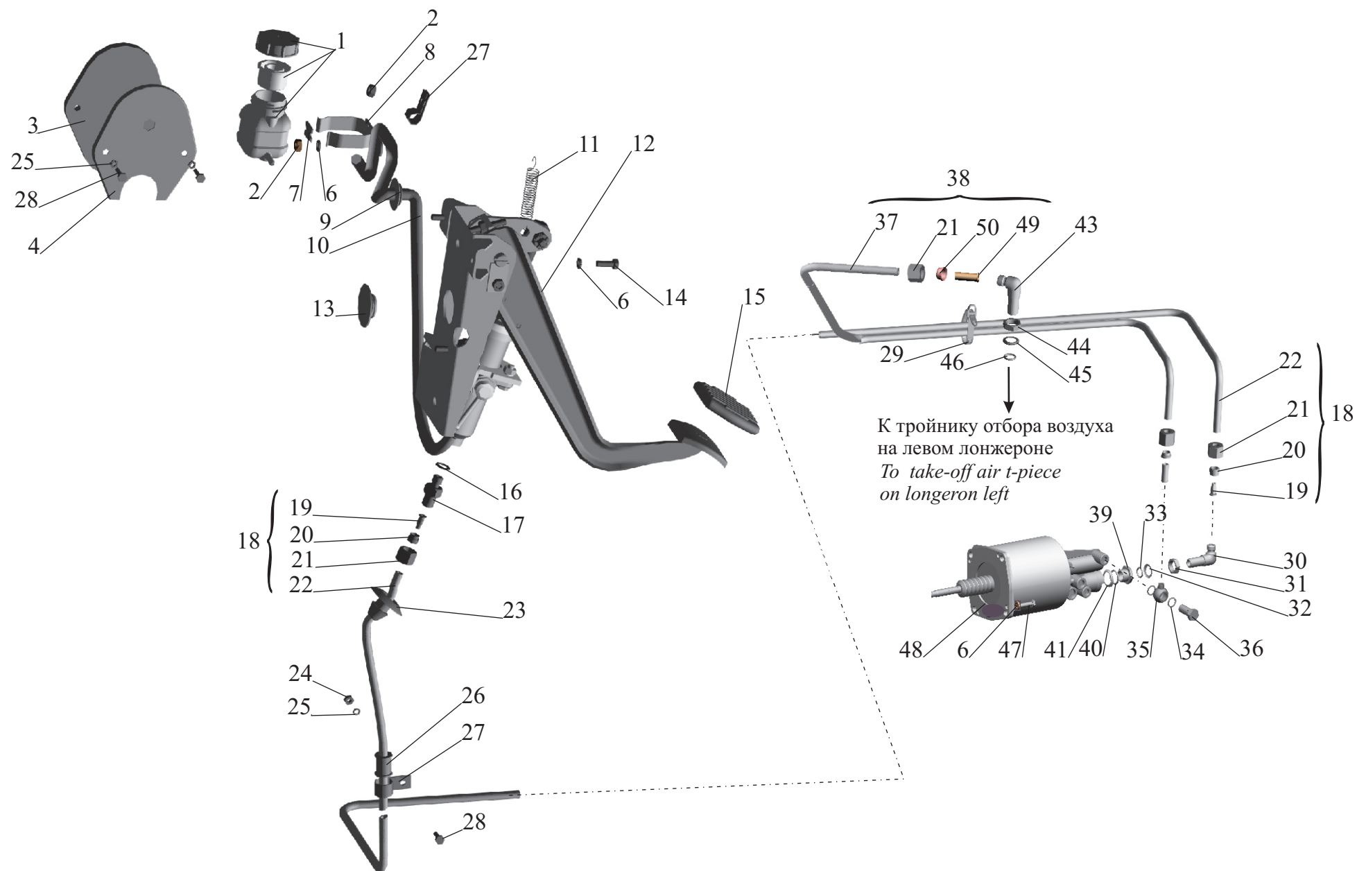
Fig. 28 Clutch control mechanism 64229-1600005-050
