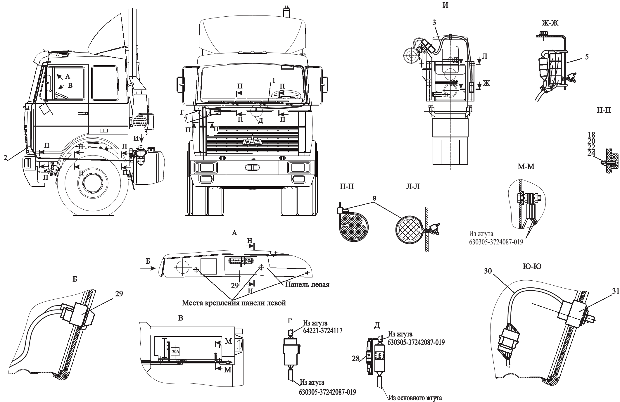
Fig. 145 Installation of electrical equipment heater 630305-3700085
