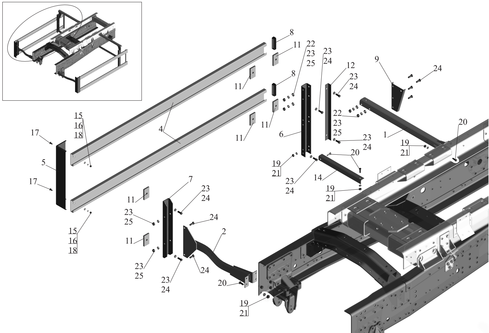
Fig. 73 Installation of a lateral protection 551605-2800040-020 (page 1)
