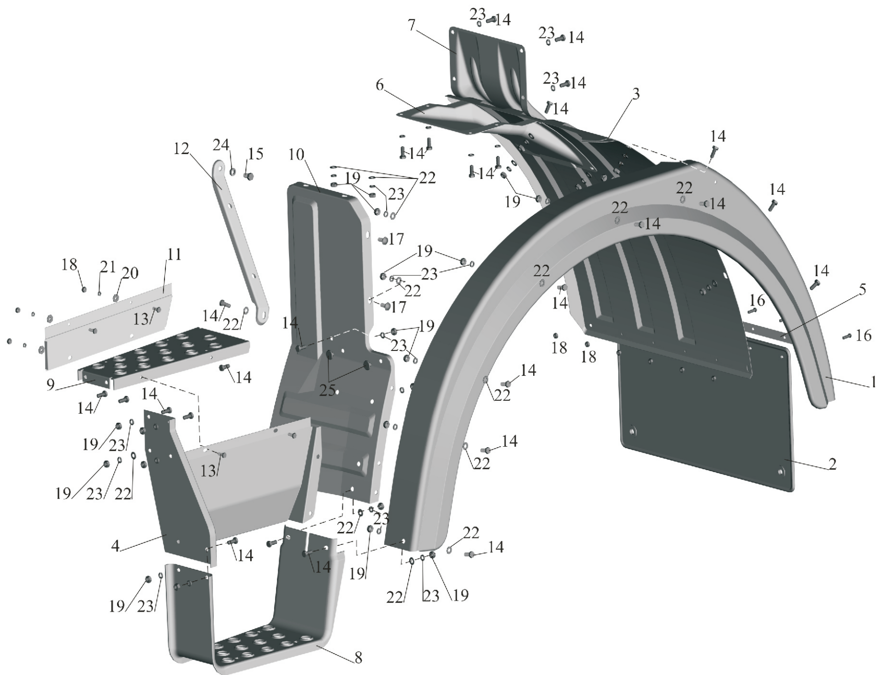
Fig. 201 Installation of plumage on small cab
