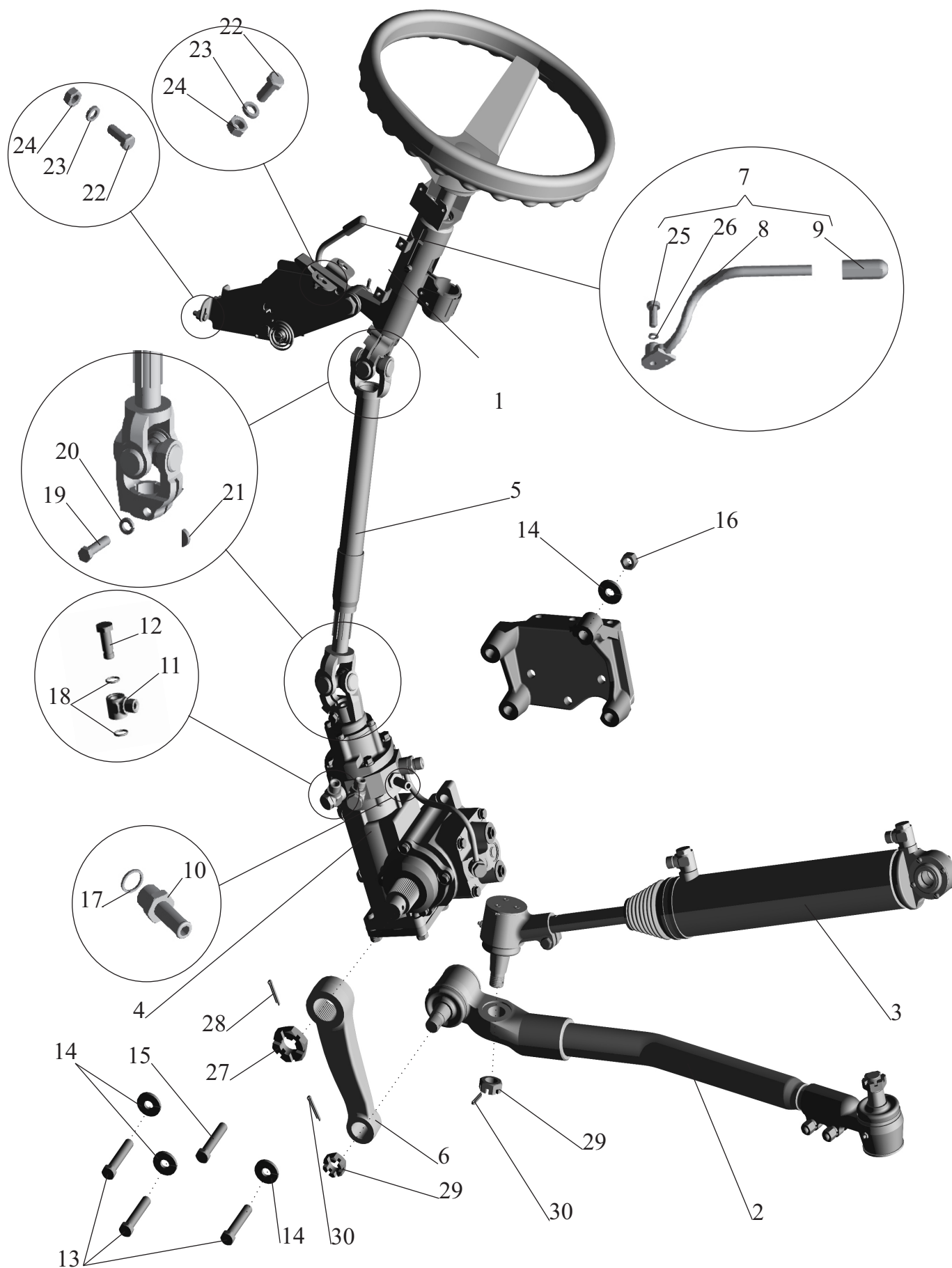
Fig. 89 Steering column and steering mechanism mounting
