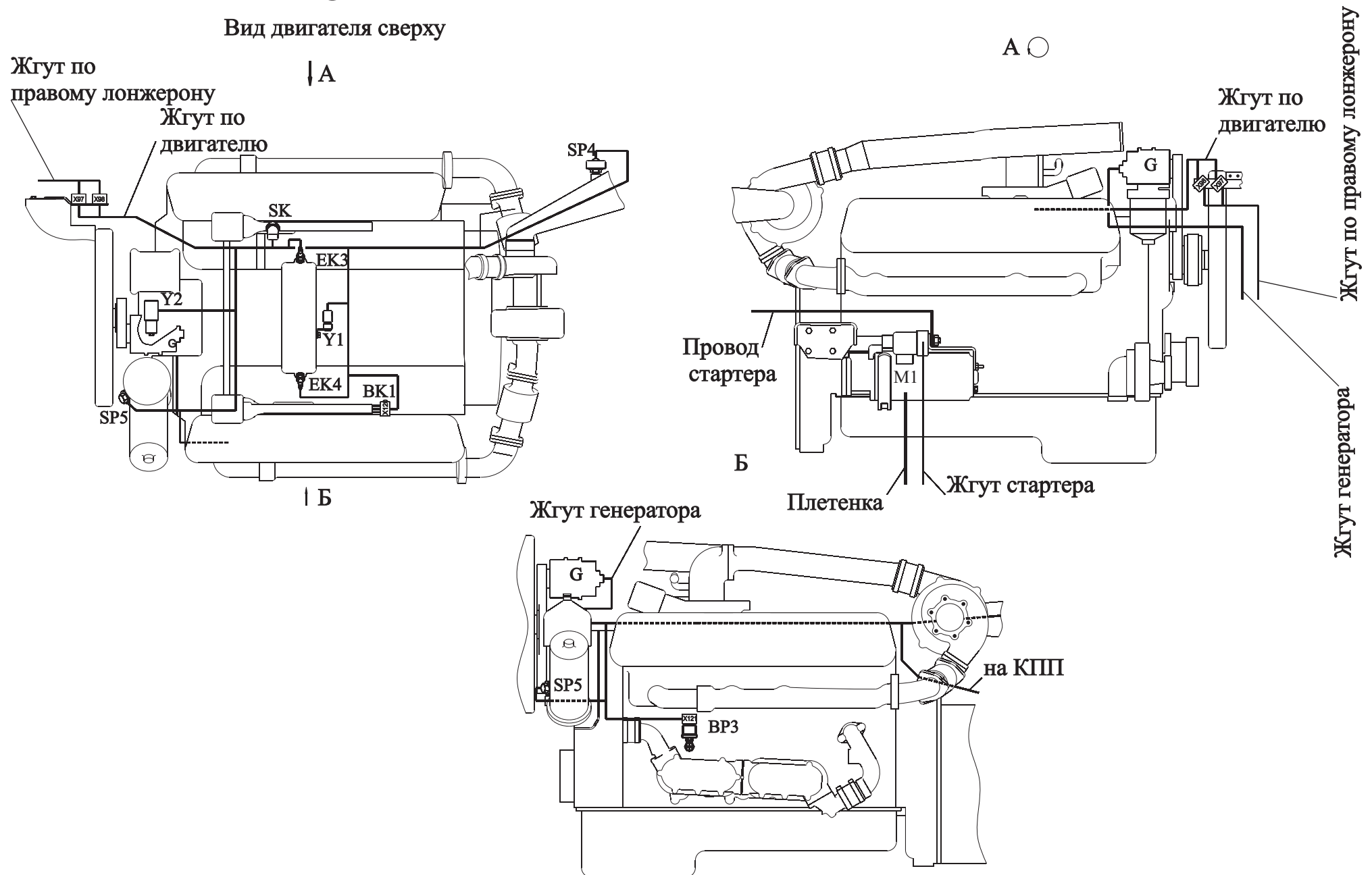
Fig. 150 An arrangement of sockets and elements of an electric equipment on engine JAMZ-238DE2, JAMZ-7511
