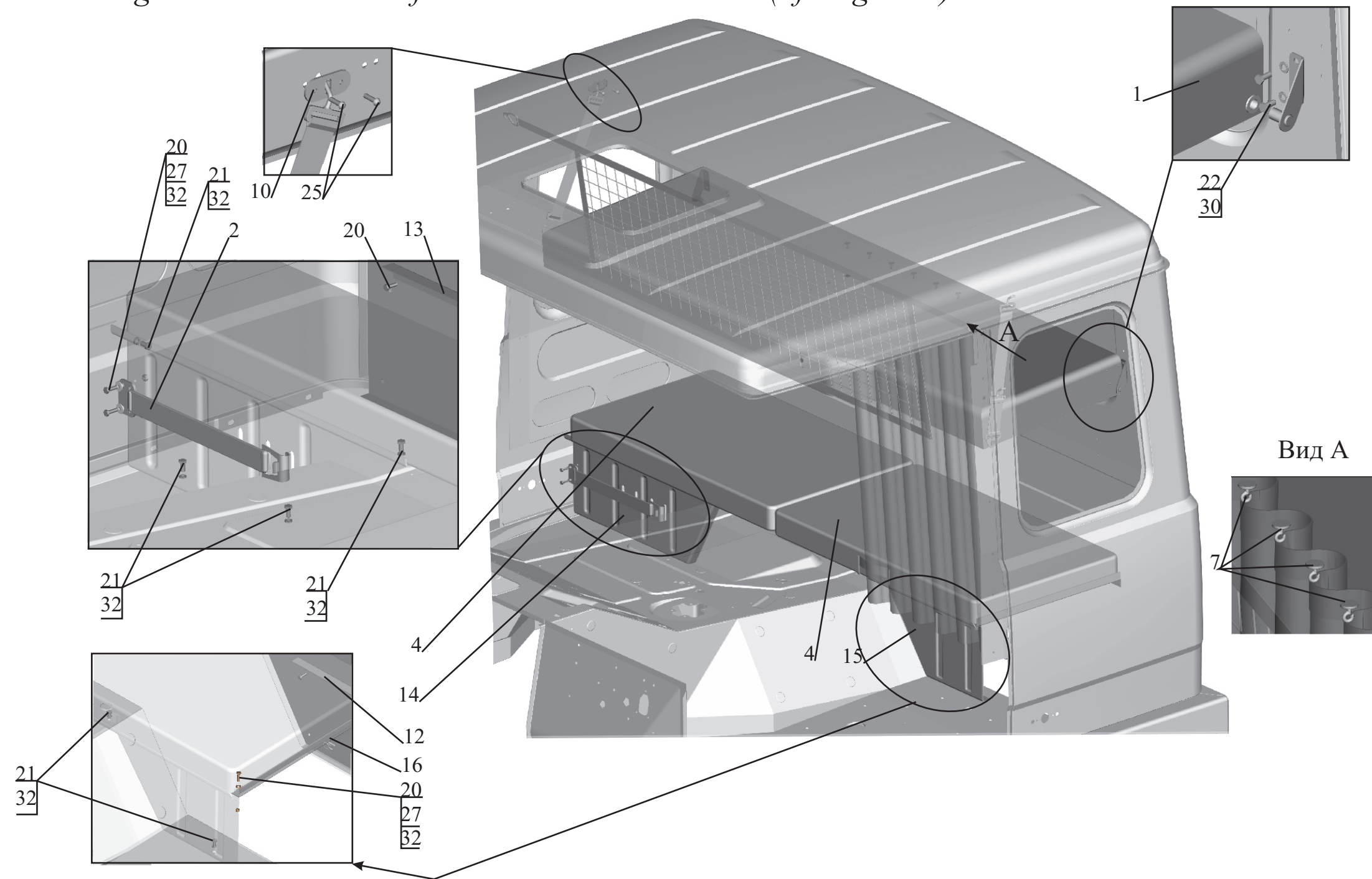
Fig. 197 Installation of a berths 64221-8200010 (of large cab)
