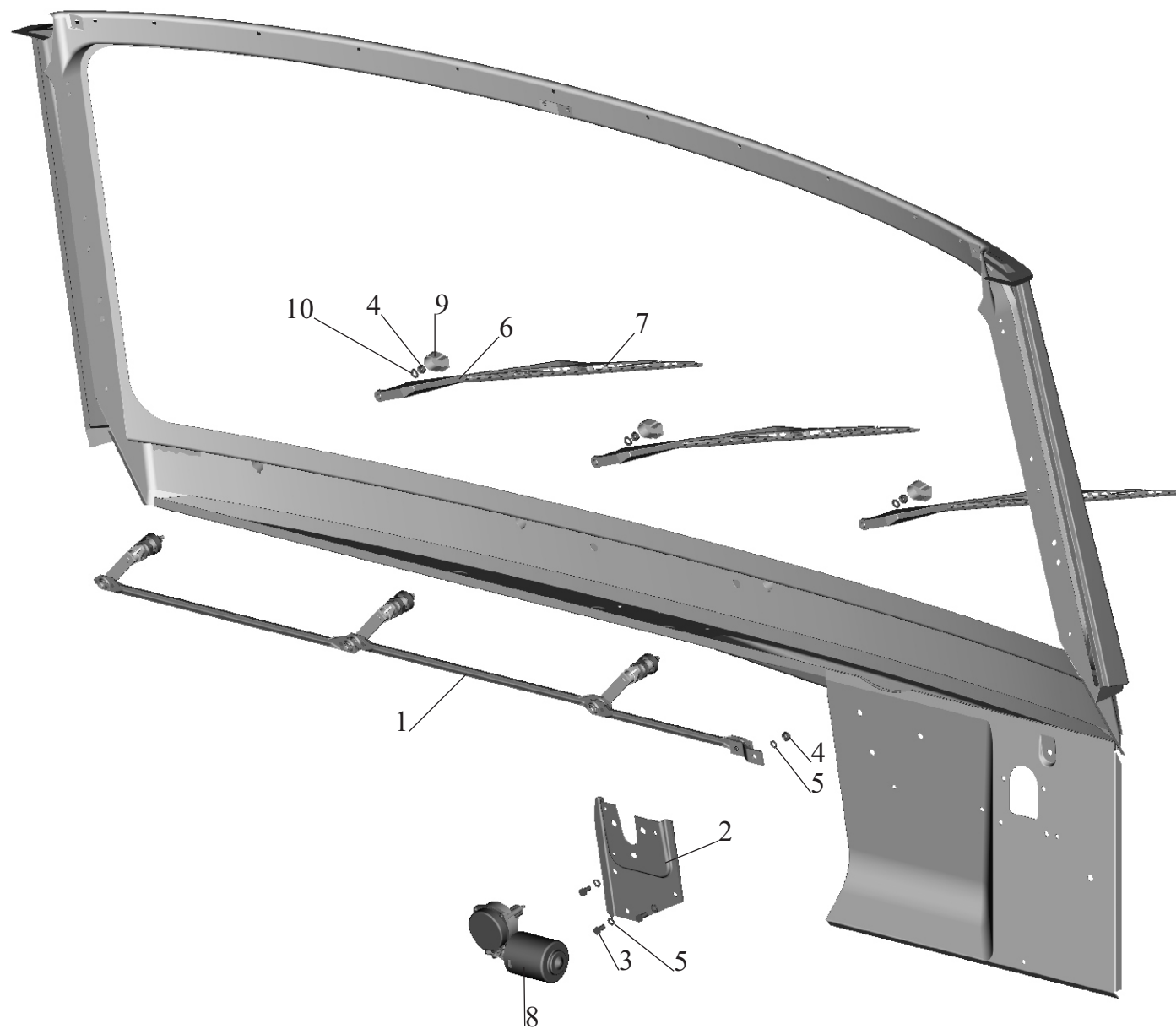
Fig. 135 Installation of cleaner of glasses 64221-3700041-010
