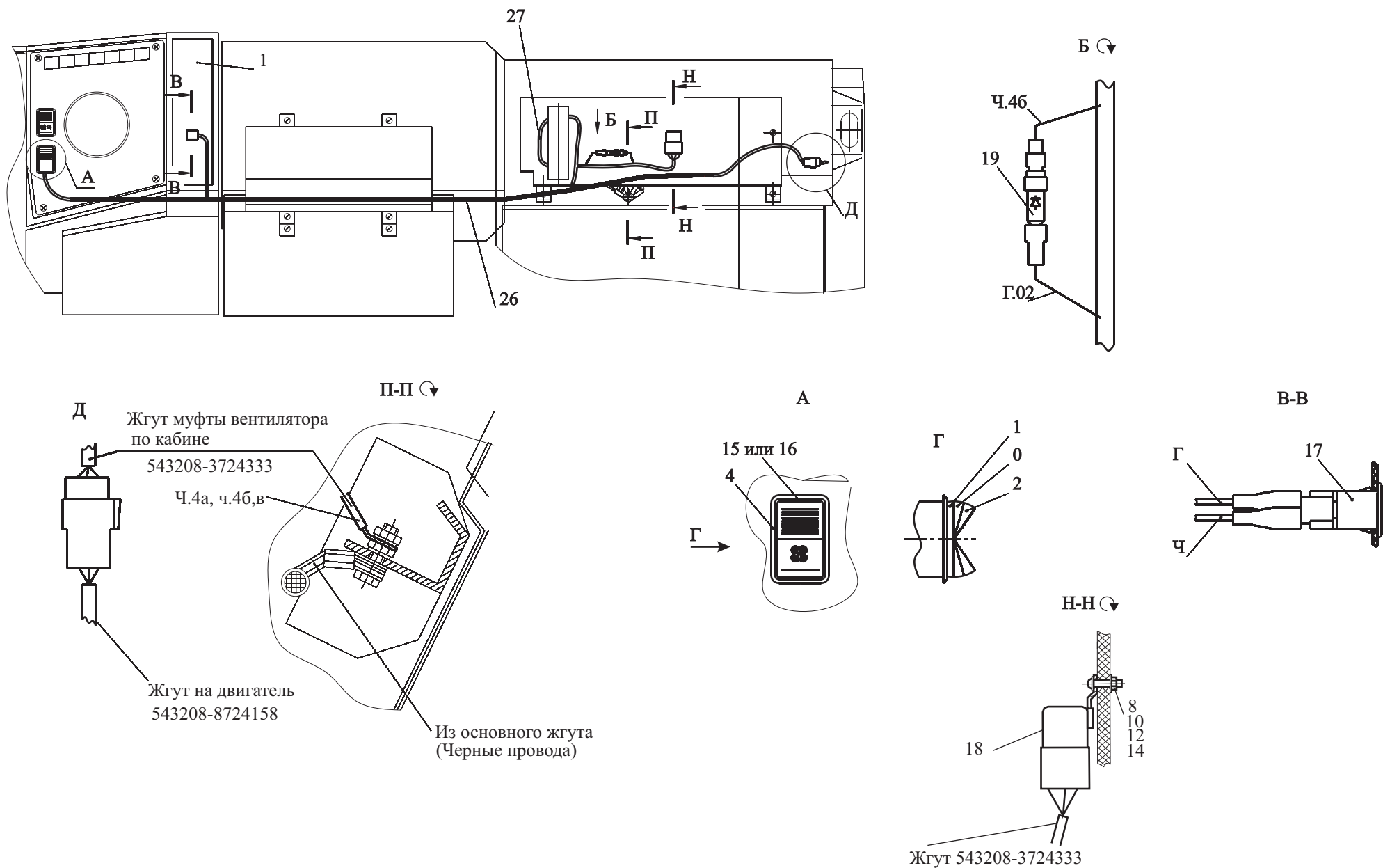
Fig. 134 Installation of an electric equipment of fan clutch 543208-37000073, 543208-37000073-700
