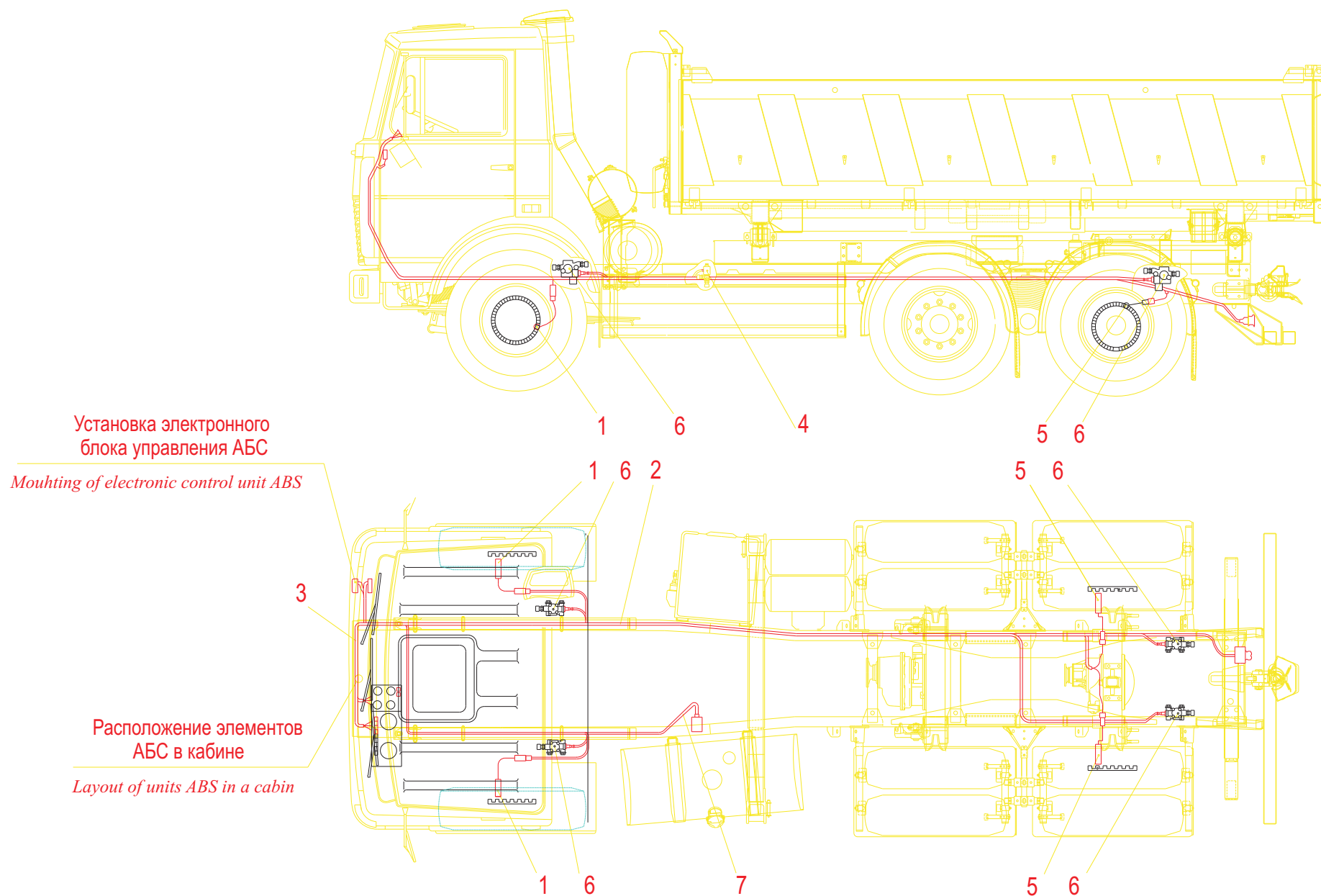
Fig. 164 Mounting of electrical equipment elements of ABS on MAZ-551605
