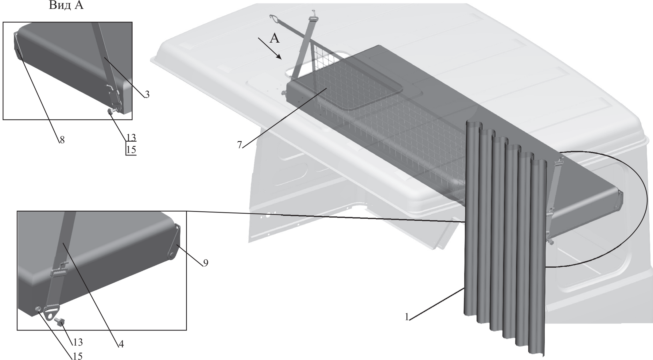
Fig. 198 Installation of upper berth 64221-8200011
