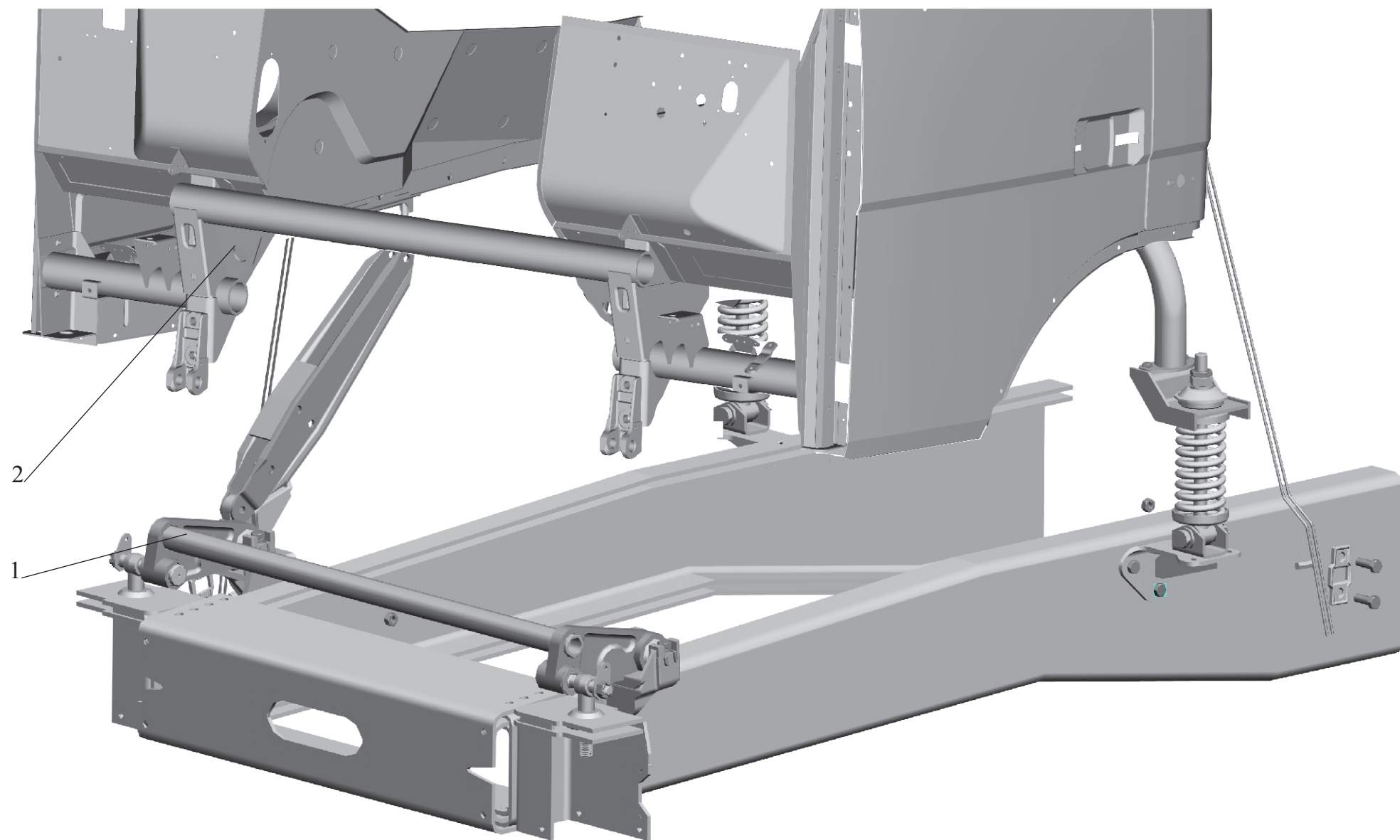
Fig. 175 Installation cab
