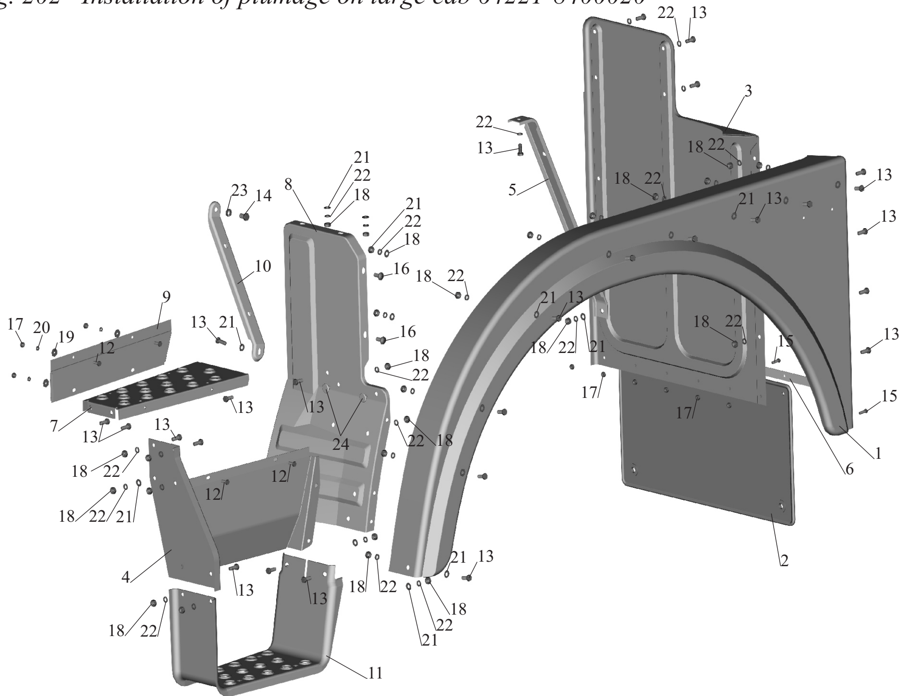
Fig. 202 Installation of plumage on large cab 64221-8400020
