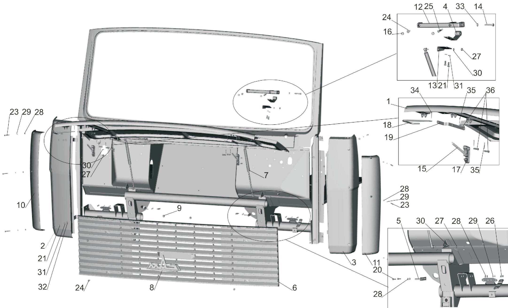
Fig. 200 Installation of facing and side flaps
