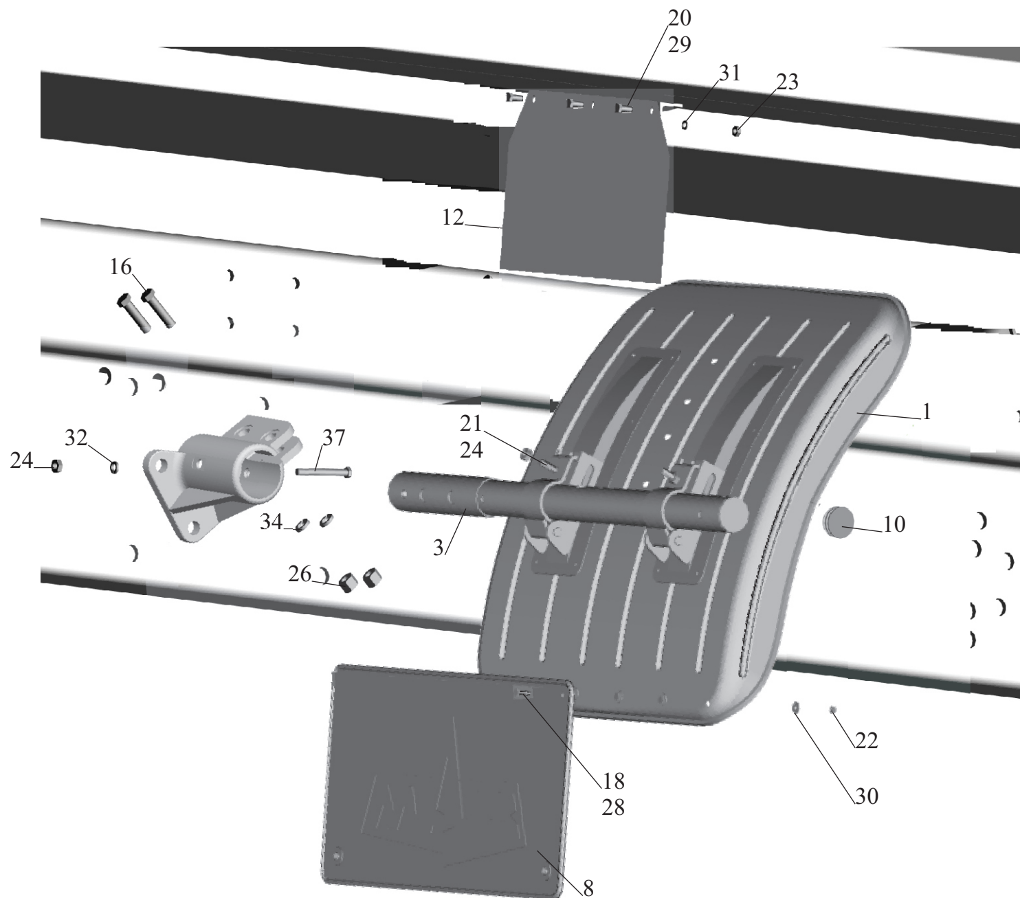
Fig. 230 The fenders installation 551605-8500048-020
