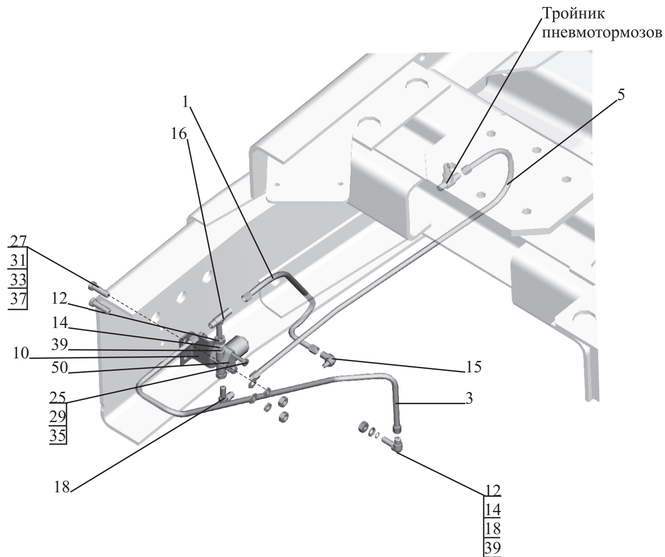
Fig. 172 Connection of power take-off gear box 551605-4200007-032
