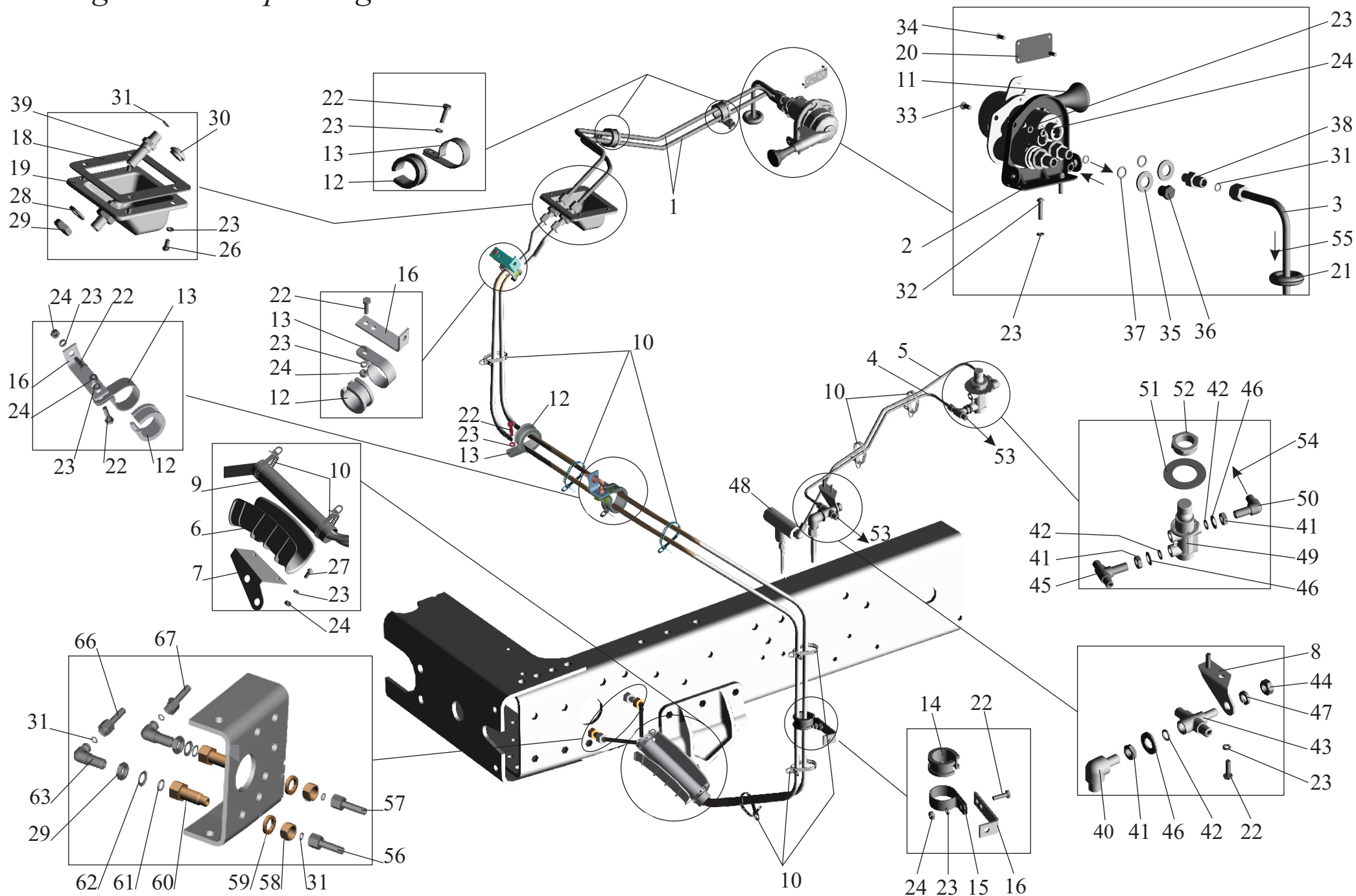
Fig. 120 The parking and motor brakes drive 5516-3537004
