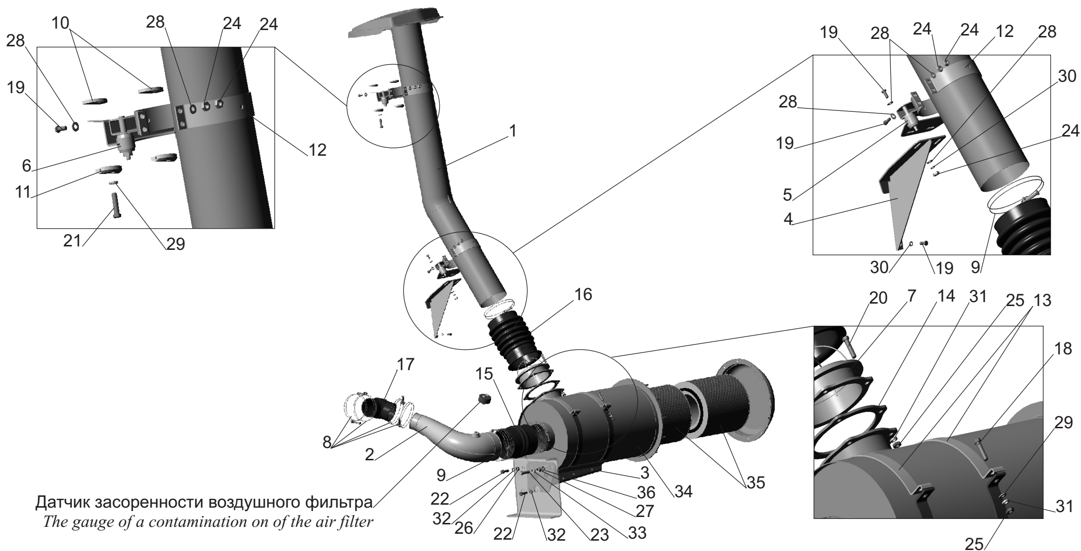
Fig. 18 Mounting air cleaner 551605-1109002-030
