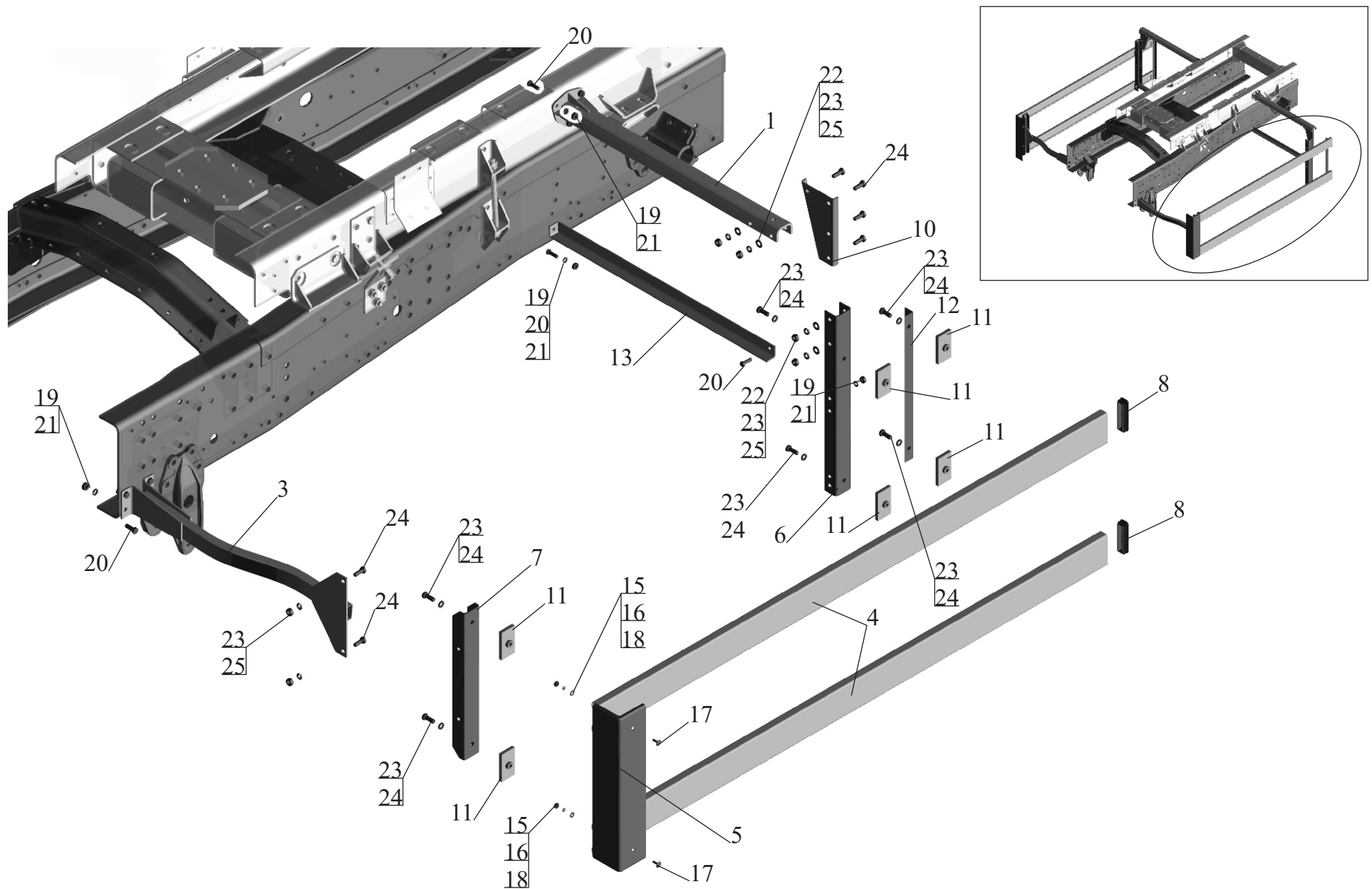
Fig. 73 Installation of a lateral protection 551605-2800040-020 (page 2)
