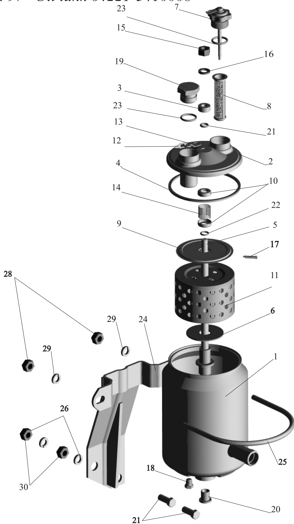
Fig. 97 Oil tank 64221-3410008
