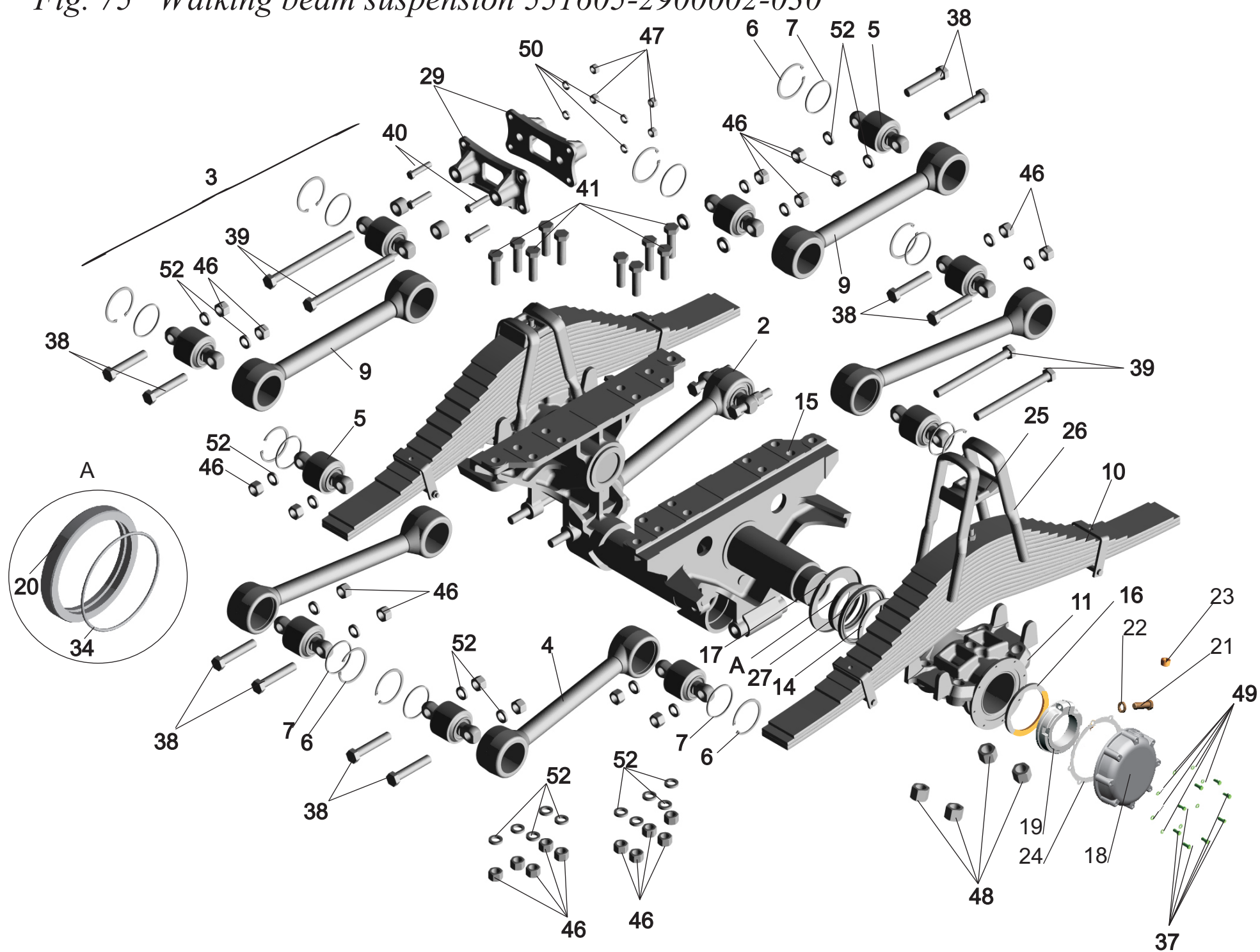
Fig. 75 Walking beam suspension 551605-2900002-030
