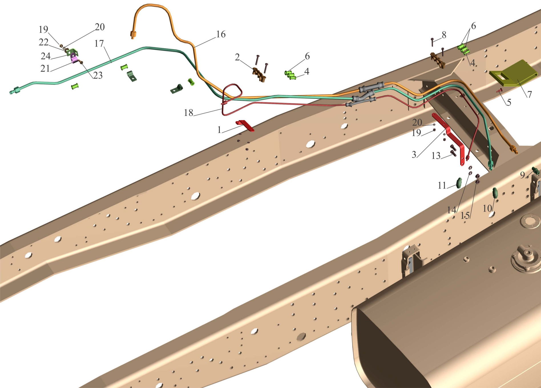
Fig.23 Installation of fuel lines MAZ-543203, 543202 (without heater)
