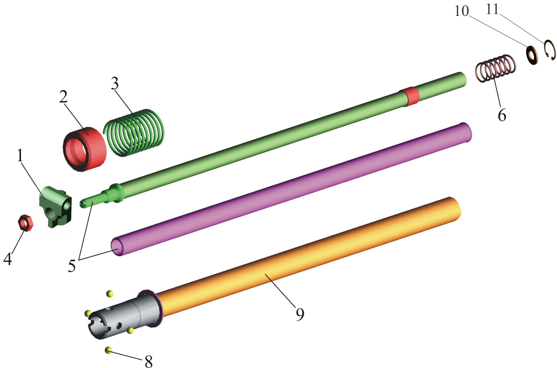
Fig. 54 Intermediate linkage
