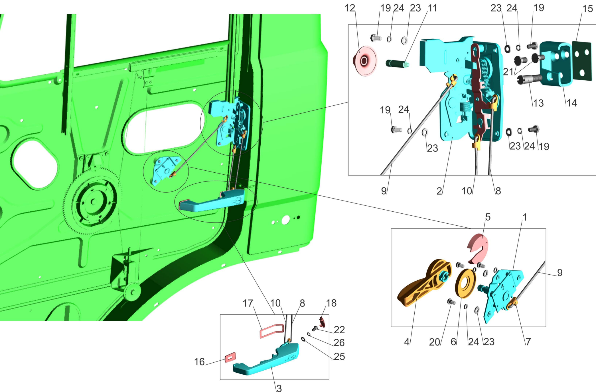
Fig.229 Installation at door outside handle and lock
