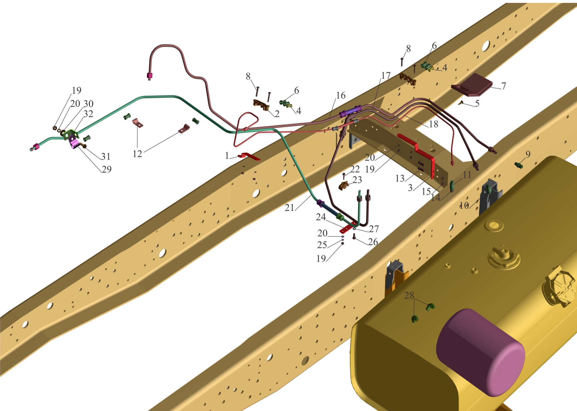
Fig.22 Installation of fuel lines MAZ-543203, 543202 (with heater)
