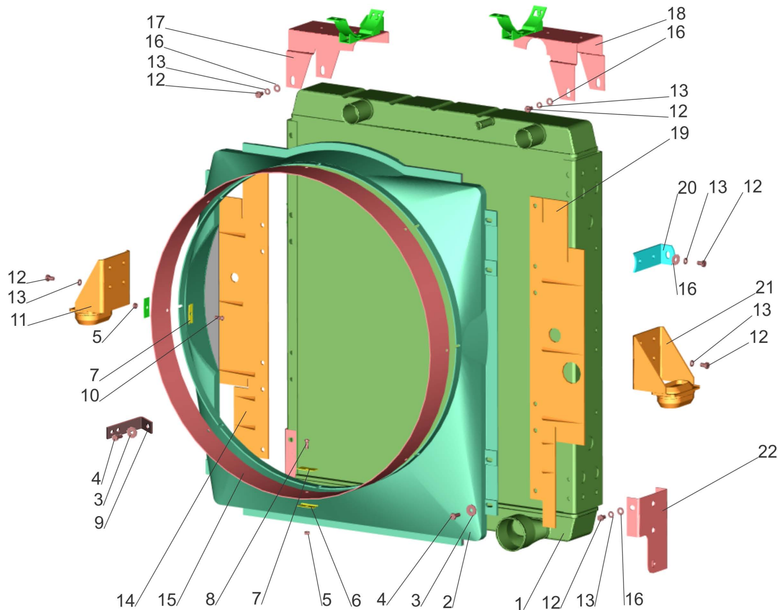
Fig. 46 Radiator with housing MAZ-642205,543205,543203,543202, 555102,551605,551603
