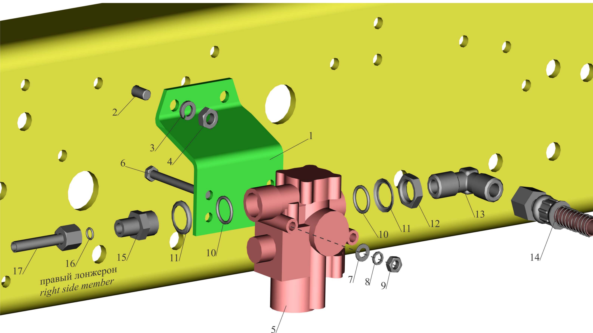
Fig.163 Installation of front modulators and attach accessories MAZ-555102, 551605, 551603
