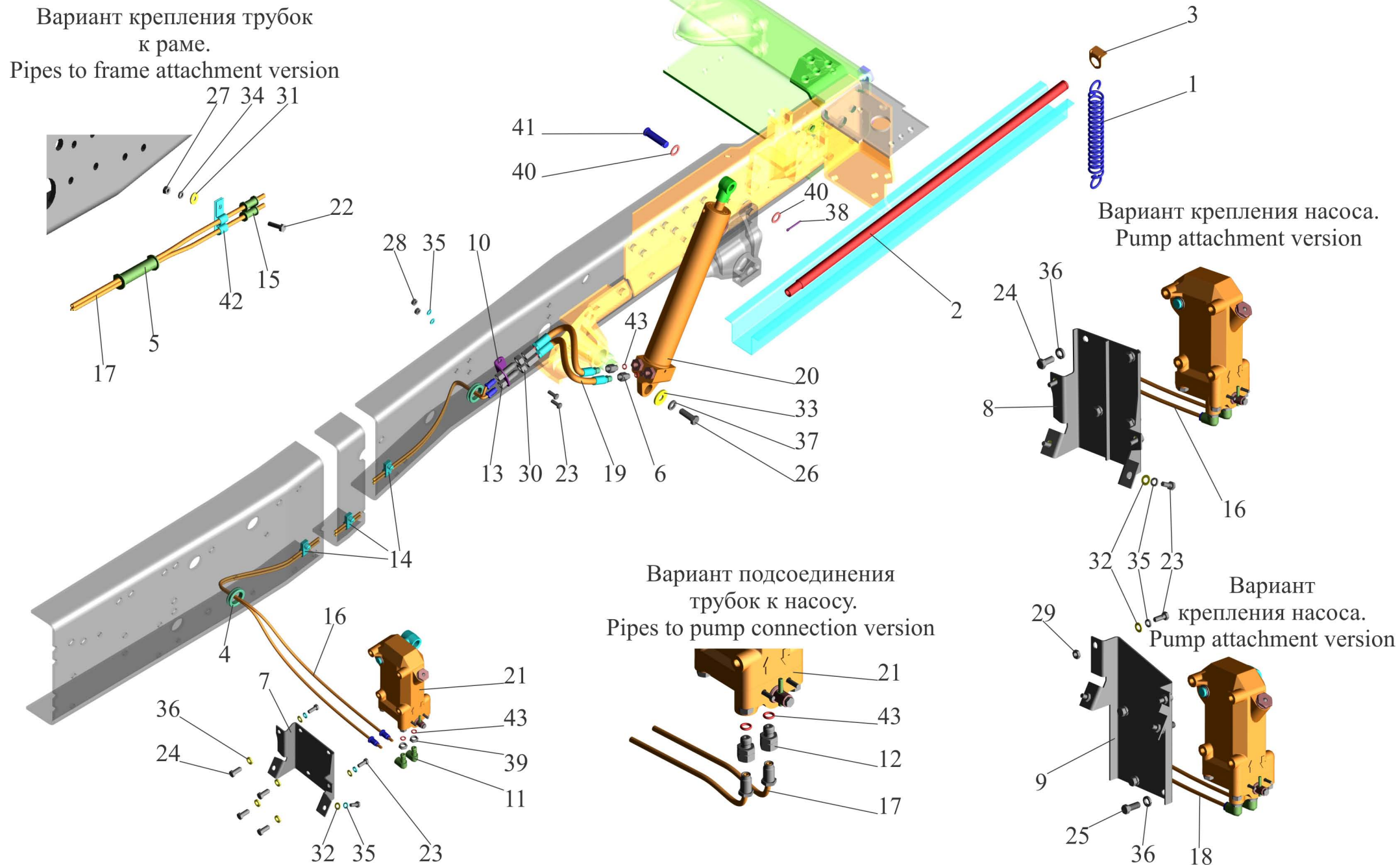
Fig.220 Cab tilting mechanism
