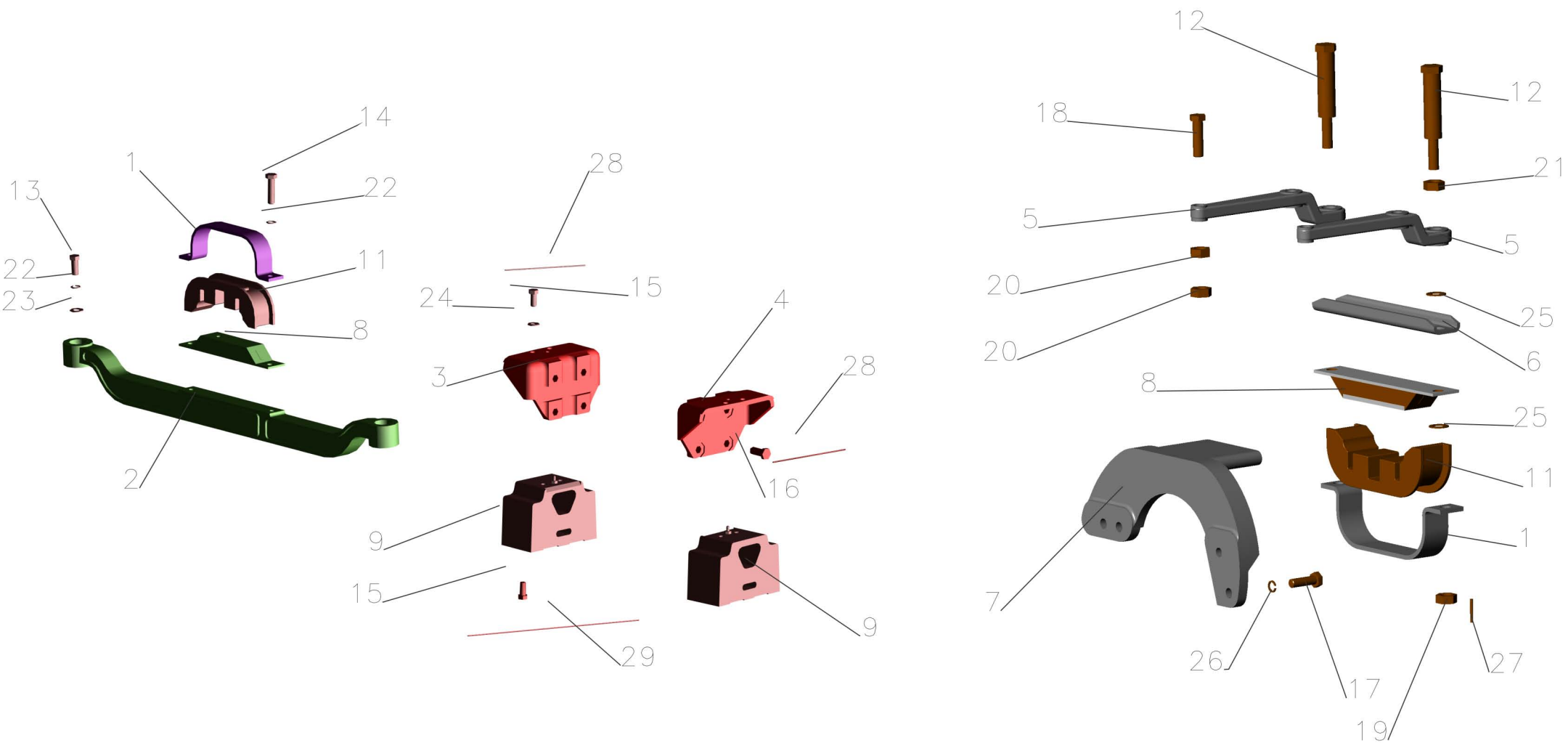
Fig.6 Mounting of engine on vehicle MAZ-555102.
