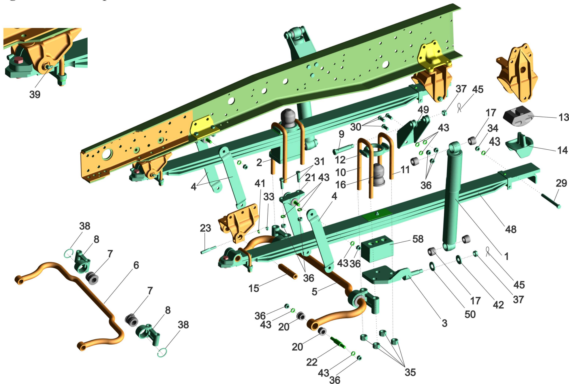
Fig.98 Front Suspension 543208-2900001.
