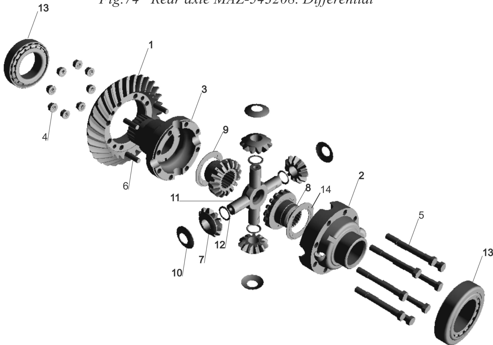
Fig.74 Rear axle MAZ-543208. Differential
