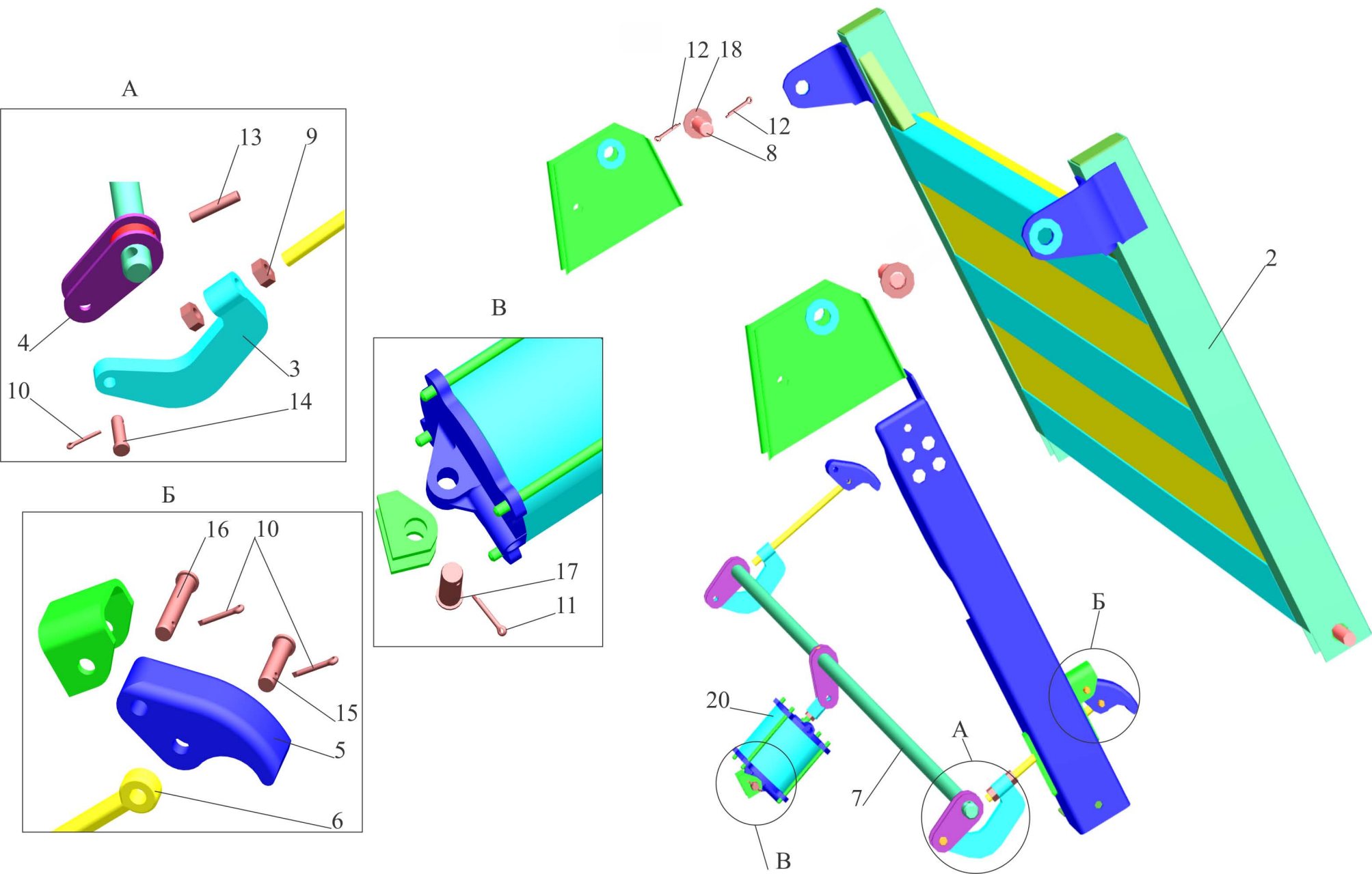
Fig. 251 Platform 555102-8500020 (page 2)
