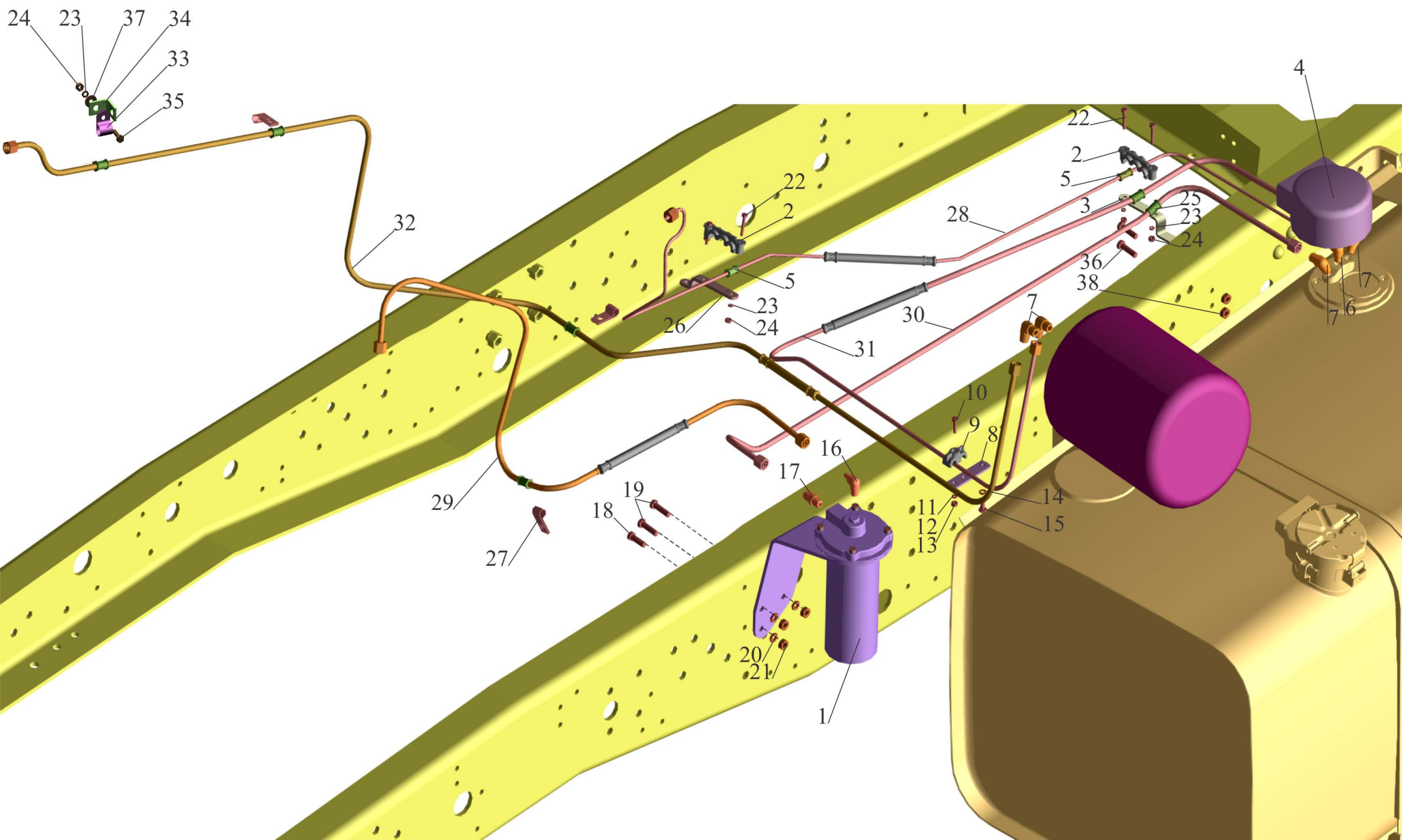
Fig.20 Installation of fuel lines MAZ-642205, 543205 (with heater)
