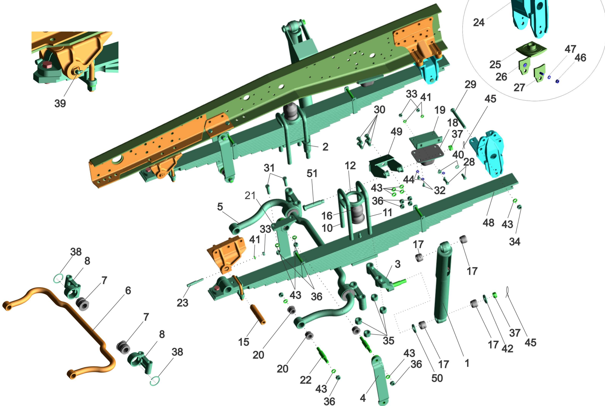
Fig.99 Front suspension 551605-2900001-010.
