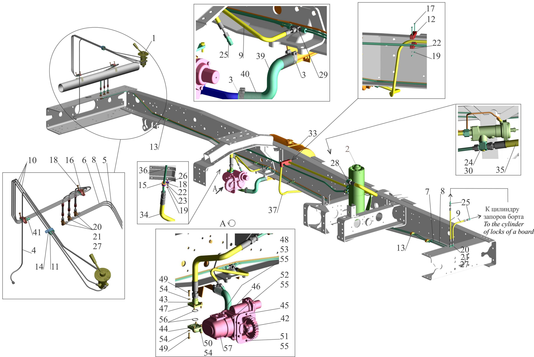
Fig.261 Installation platform tipping mechanism MAZ-555102.
