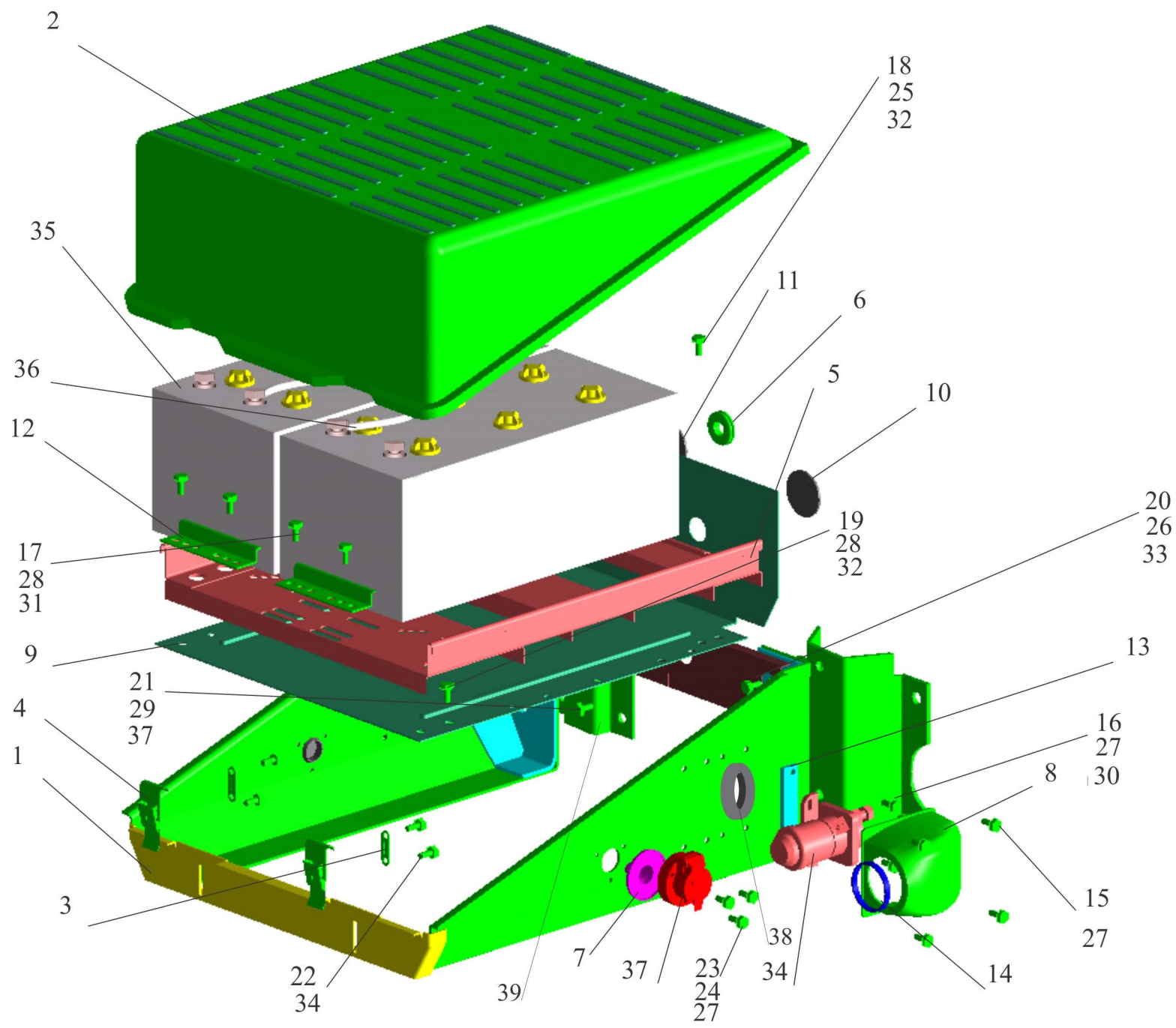
Fig.192 Installation of storage batteries.
