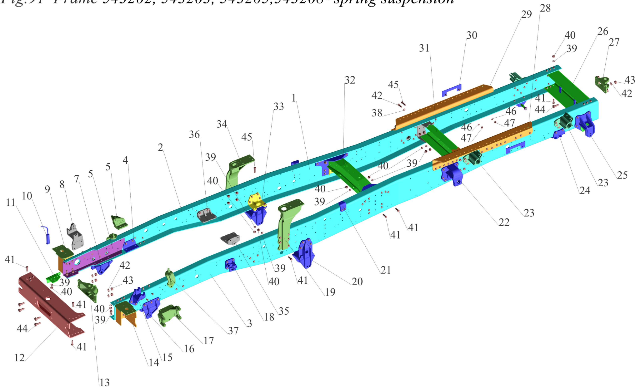
Fig.91 Frame 543202, 543203, 543205,543208- spring suspension
