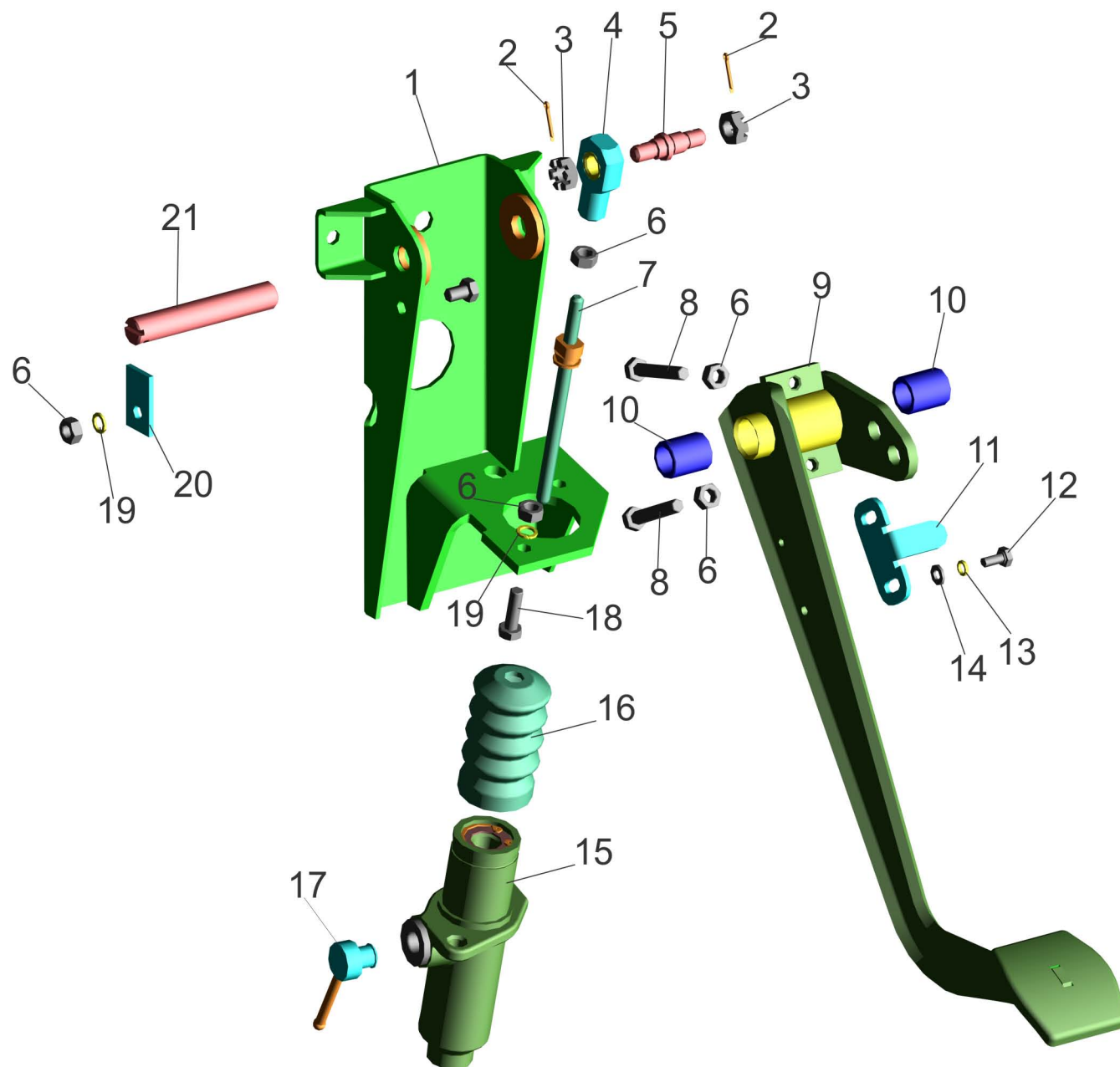
Fig.49 Pedal base 64226-1602004, 64221-1602004-10
