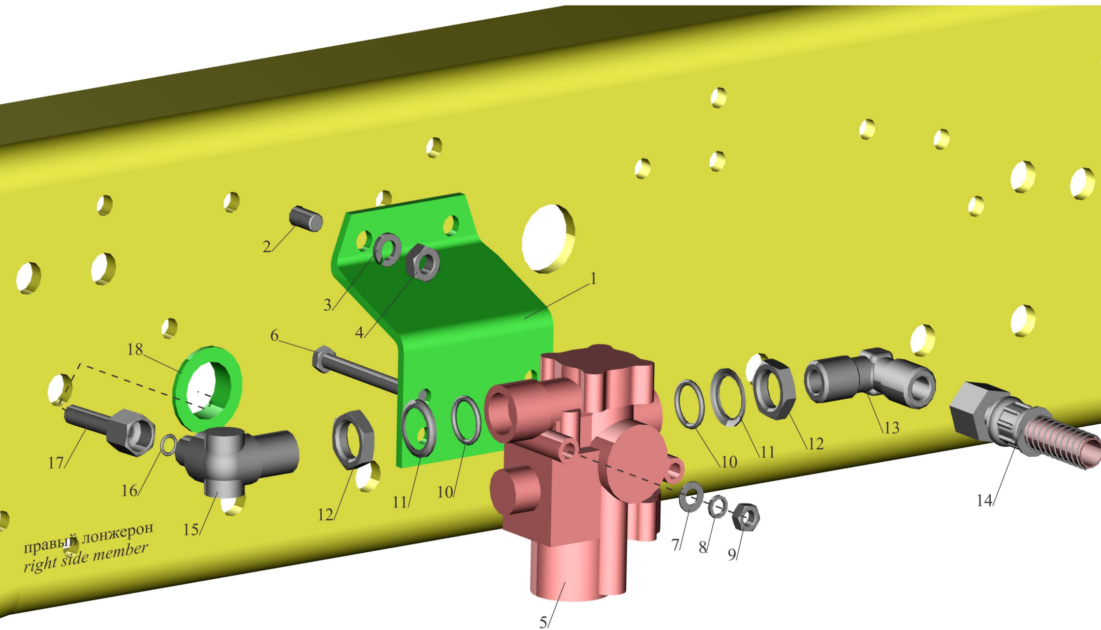
Fig.159 Installation of front modulators and attach accessories MAZ-642208,642205,543208,543205,543203,543202
