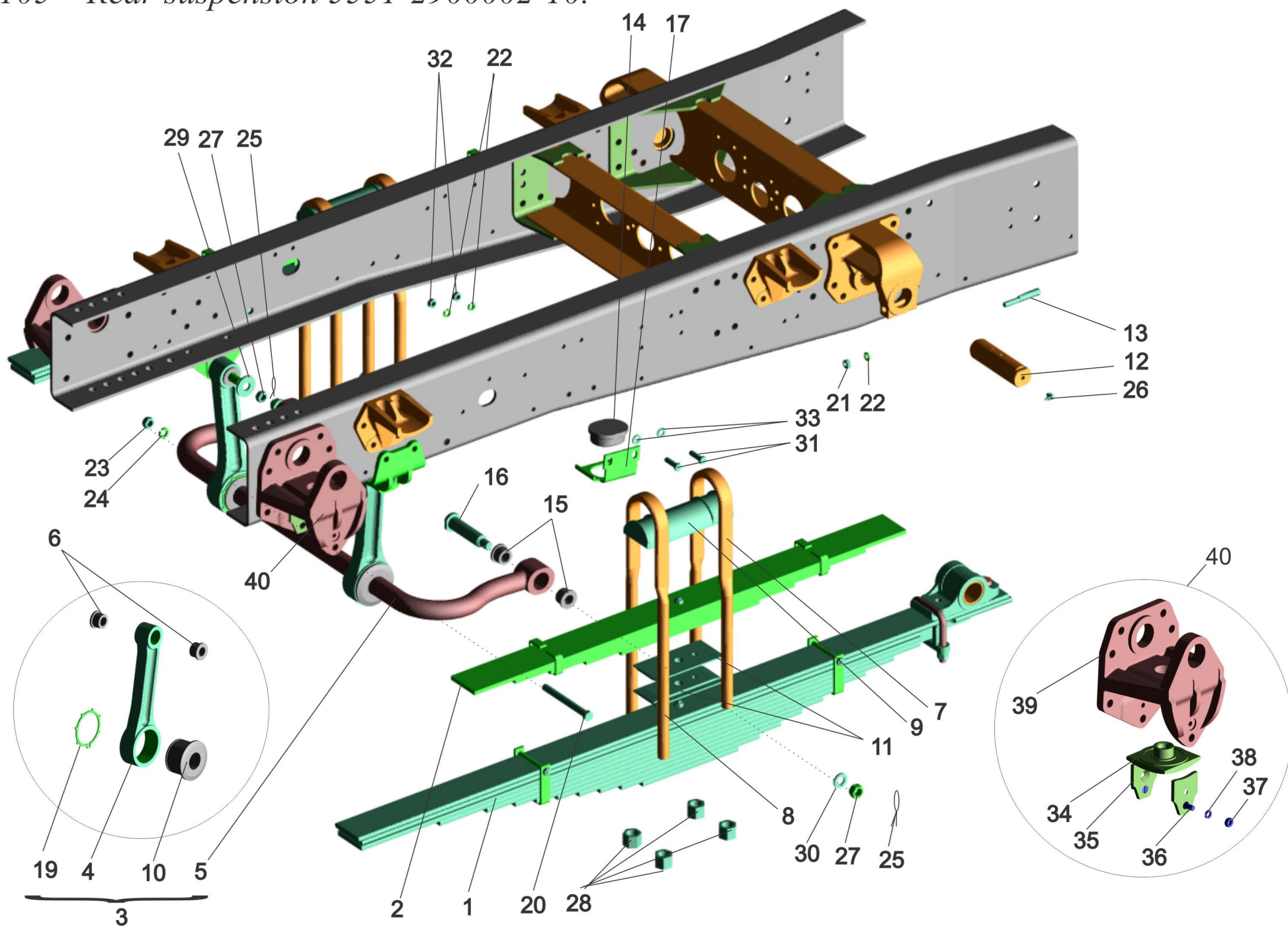
Fig.105 Rear suspension 5551-2900002-10.
