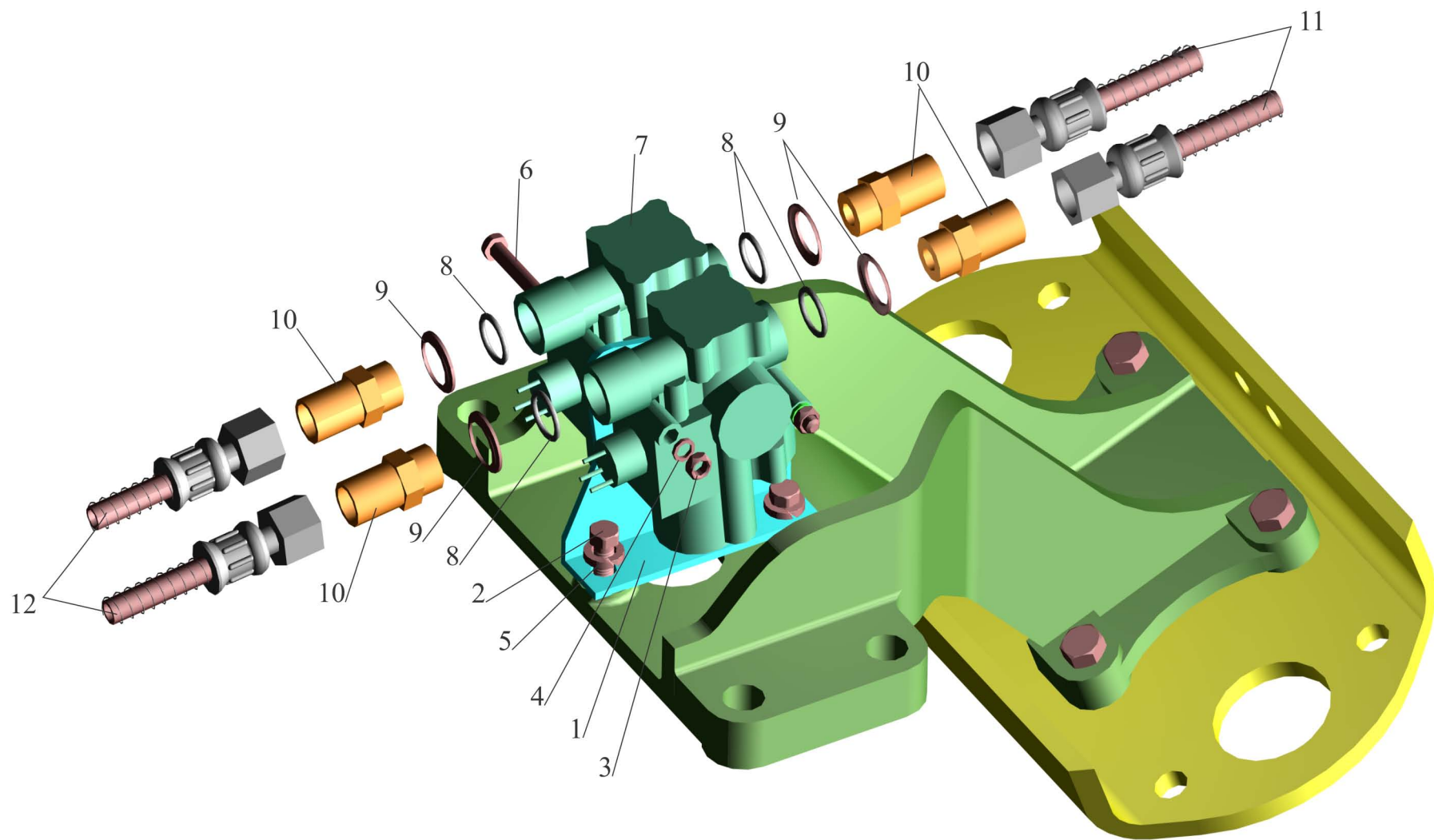
Fig.162 Installation of rear modulators and attach accessories MAZ-543208,543205,543203,543202
