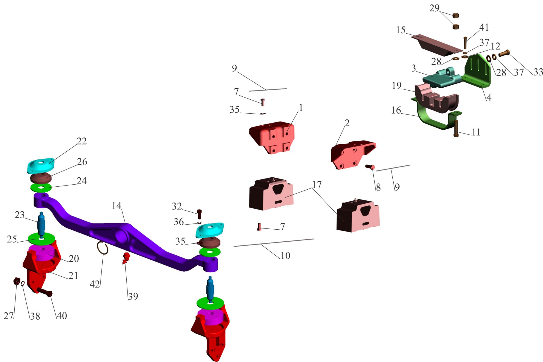
Fig. 4 Mounting of engine 551605-1001002-001.
