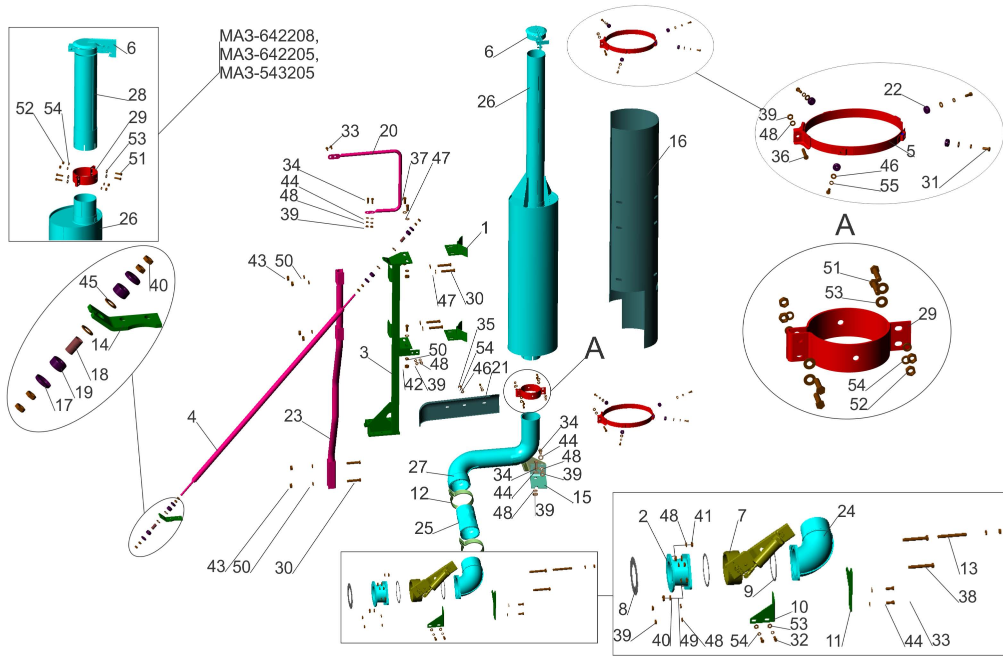
Fig.38 Installation of exhaust system MAZ-642208,642205,543208,543205,543202,543203
