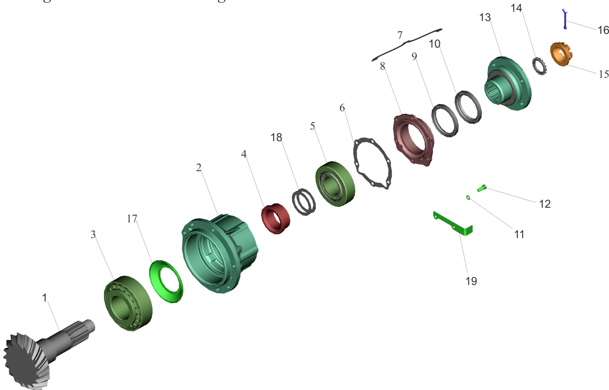
Fig.66 Rear axle reduction gear. Drive Pinion
