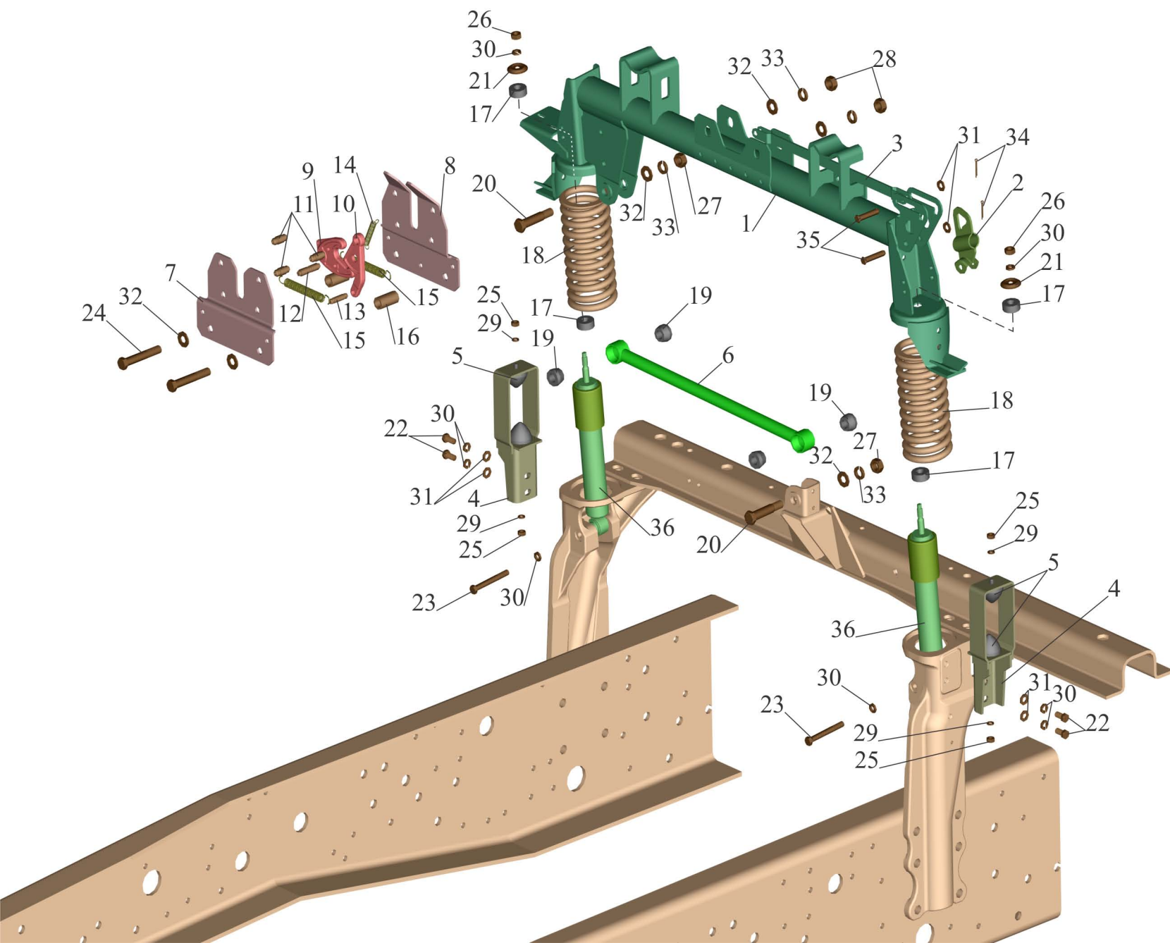
Fig.216 Rear springing the large cab
