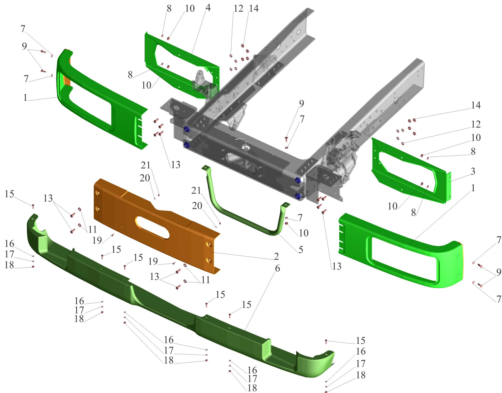
Fig.94 Mounting bumper.
