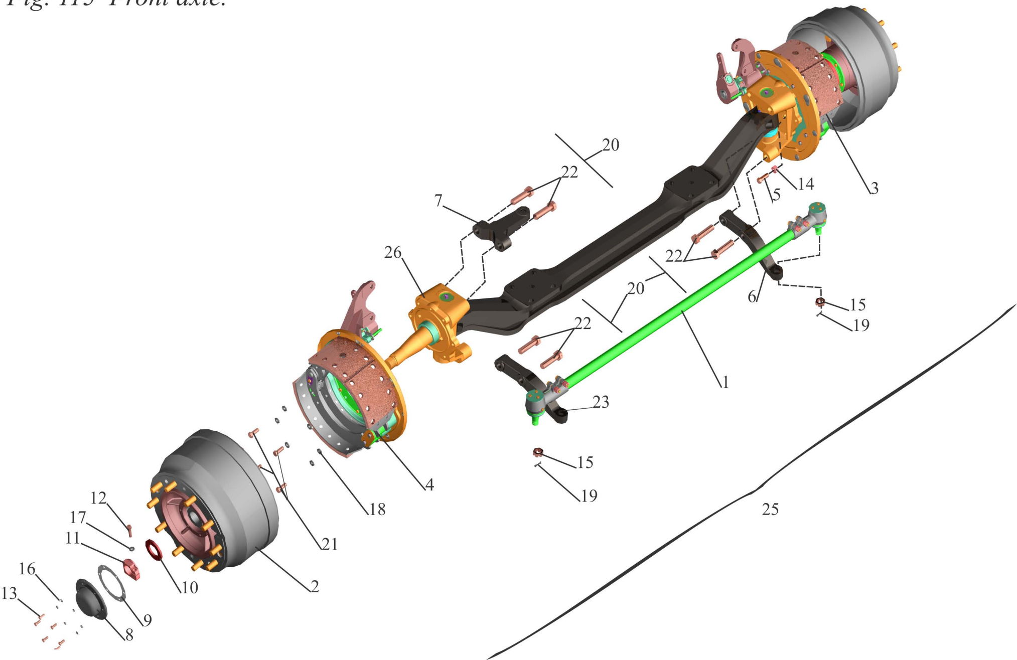
Fig. 115 Front axle.
