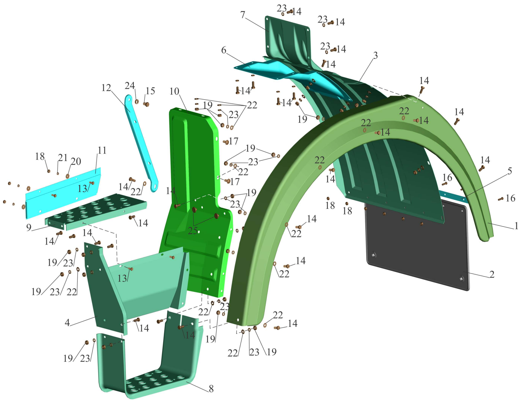
Fig.236 Installation of plumage on small cab
