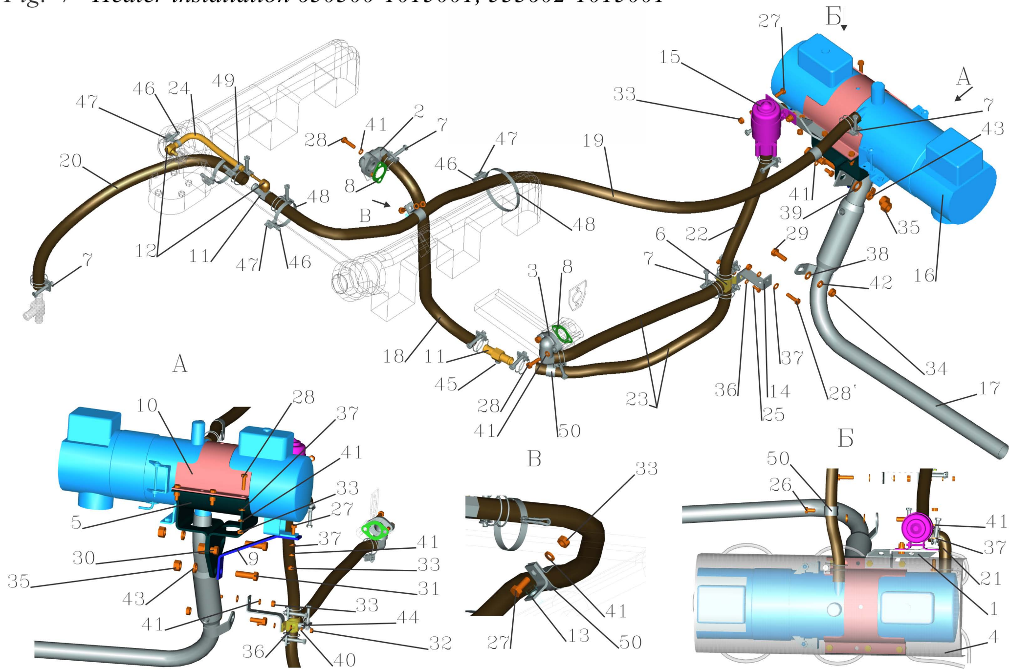
Fig. 7 Heater installation 630300-1015001, 533602-1015001
