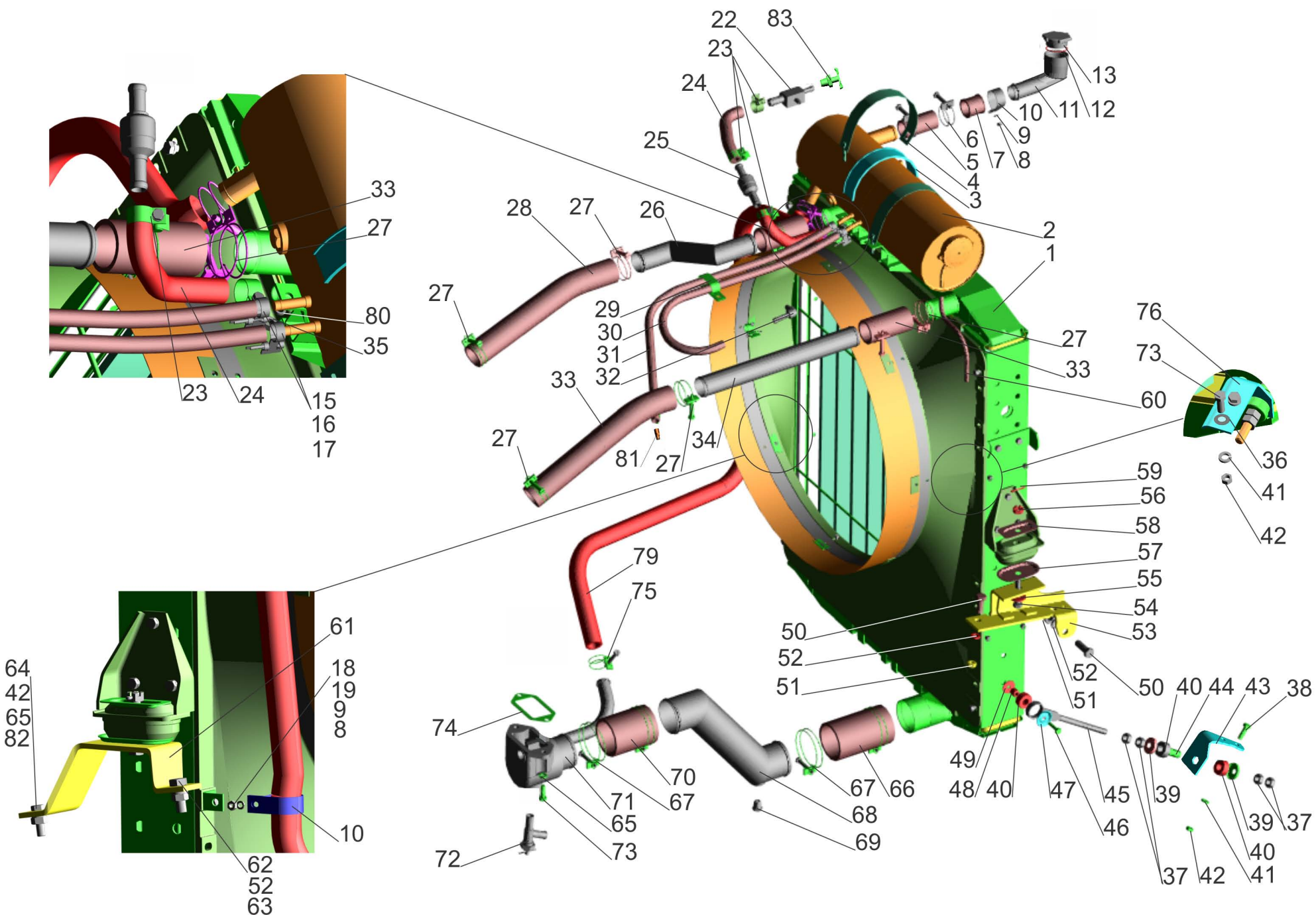
Fig. 43 Installation of cooling system MAZ-642208, 543208
