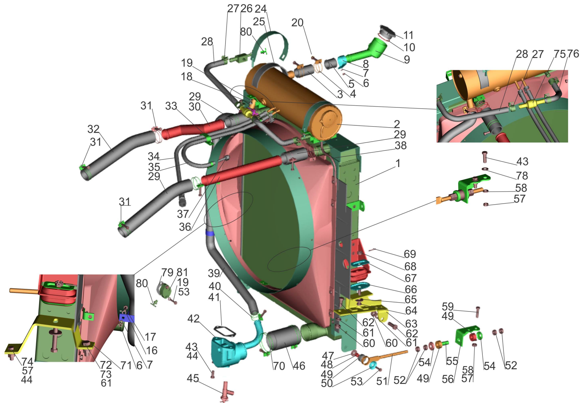
Рис. 44 Установка системы охлаждения МАЗ-642205,543205,543203,543202,555102,551605,551603 Fig. 44 Installation of cooling system MAZ-642205,543205,543203,543202,555102, 551605,551603
