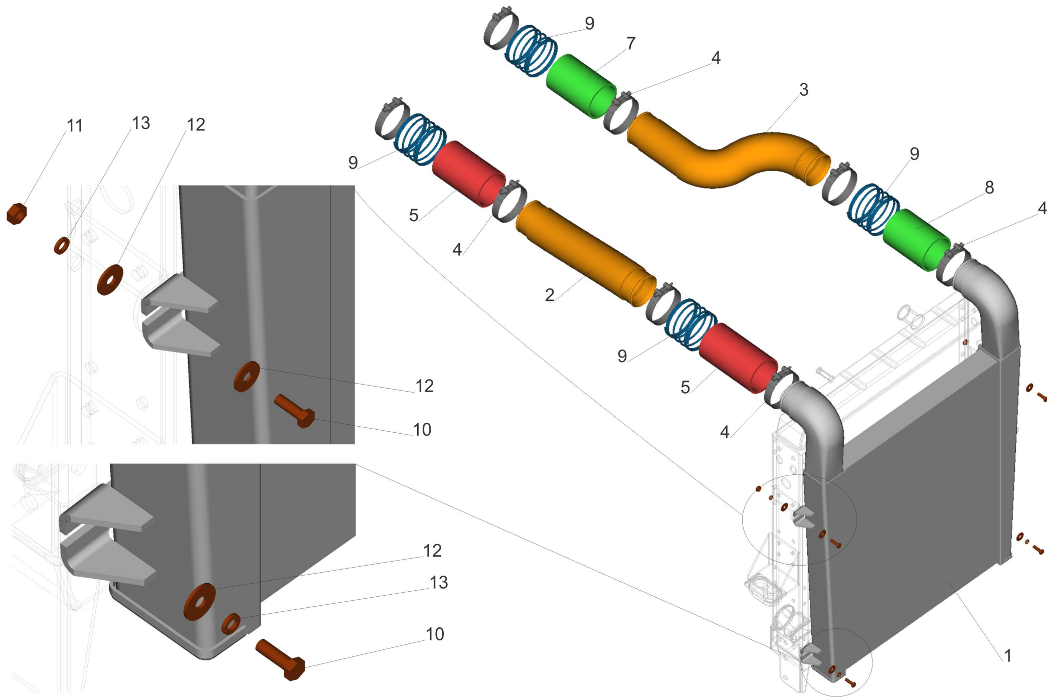
Fig.47 Supercharging air cooling system
