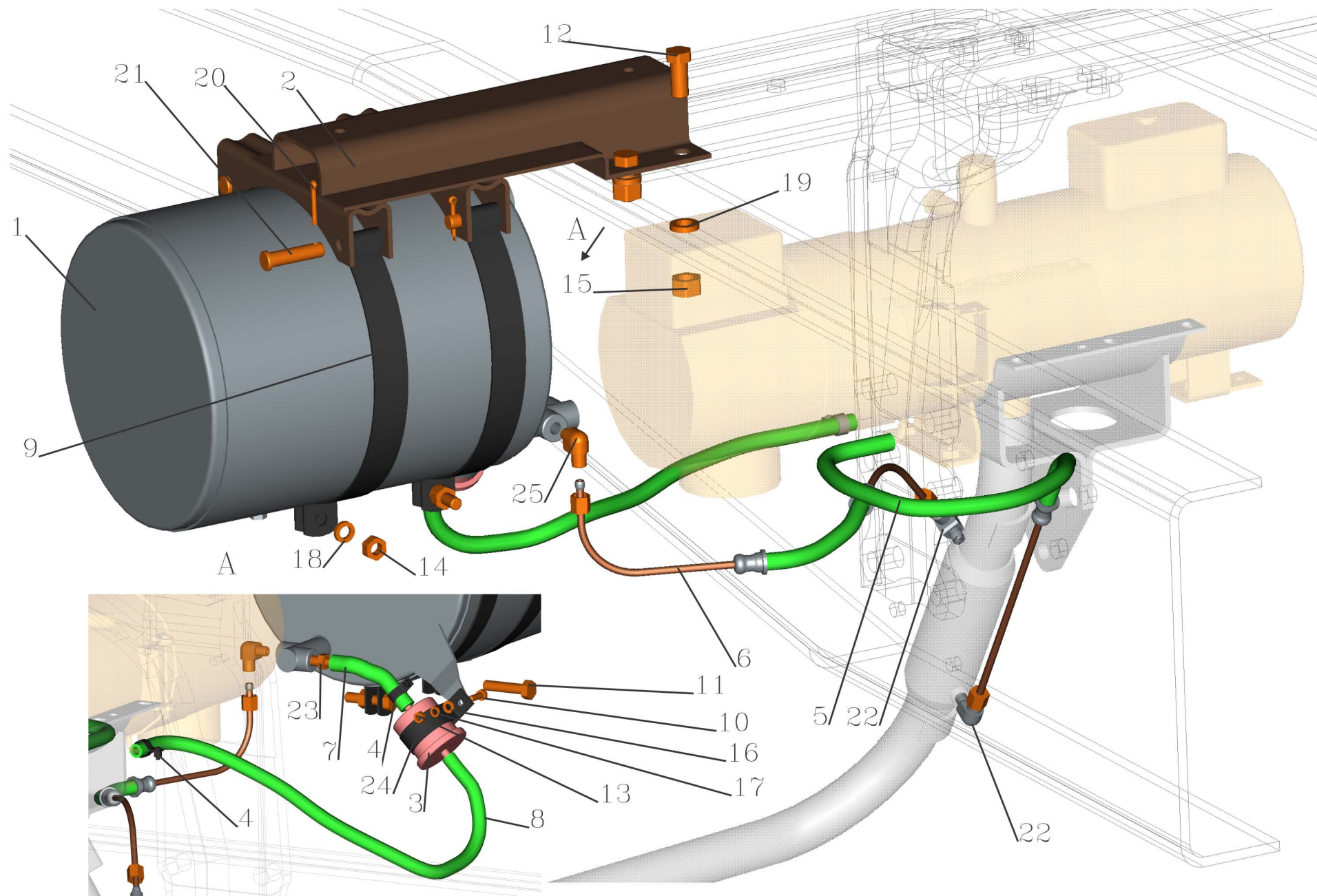
Fig. 11 Installation of heater's fuel lines 53362-1015004
