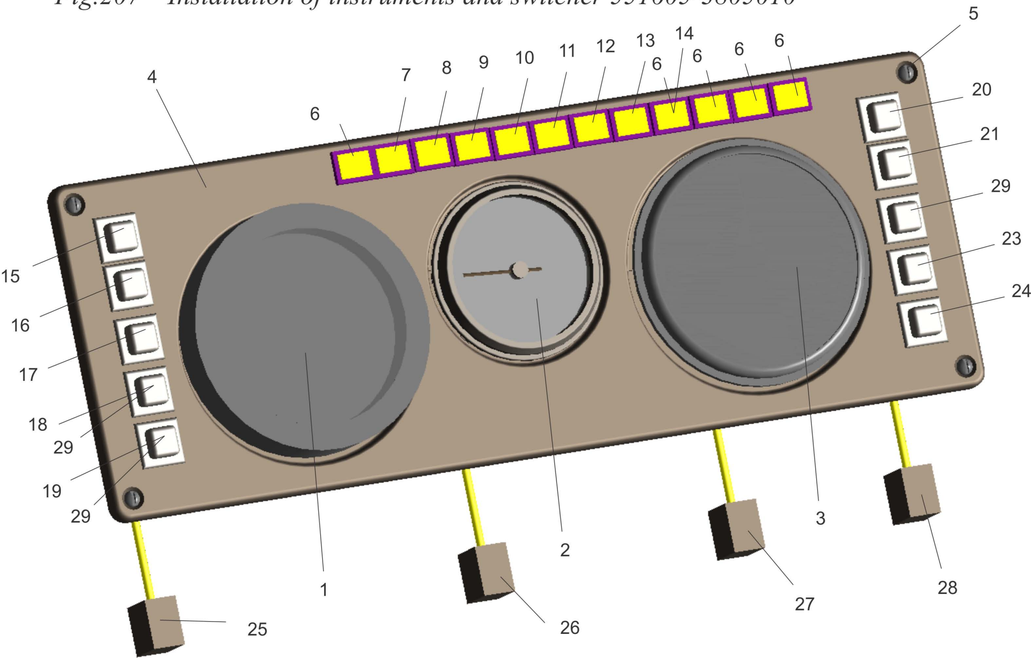
Fig.207 Installation of instruments and switcher 551605-3805010
