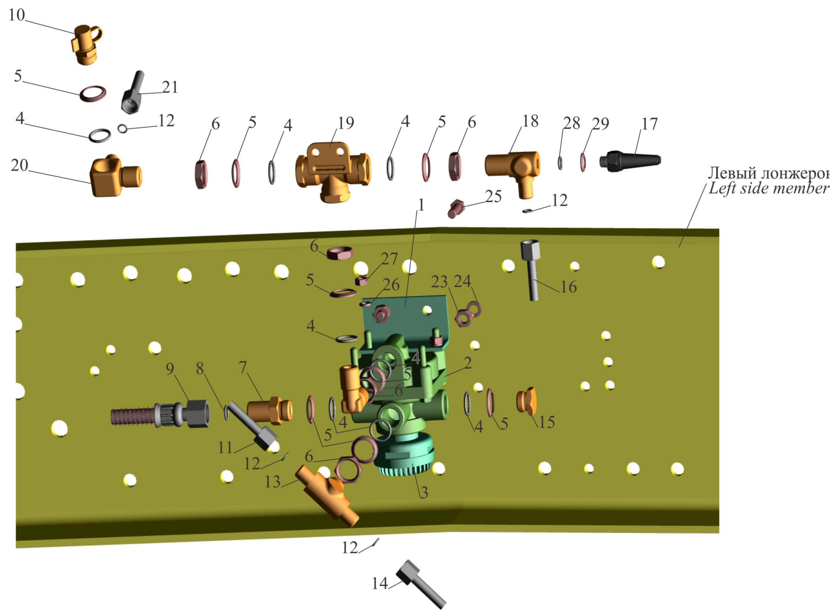
Fig. 152 Installation of relay valve and attach accessories MAZ-555102.
