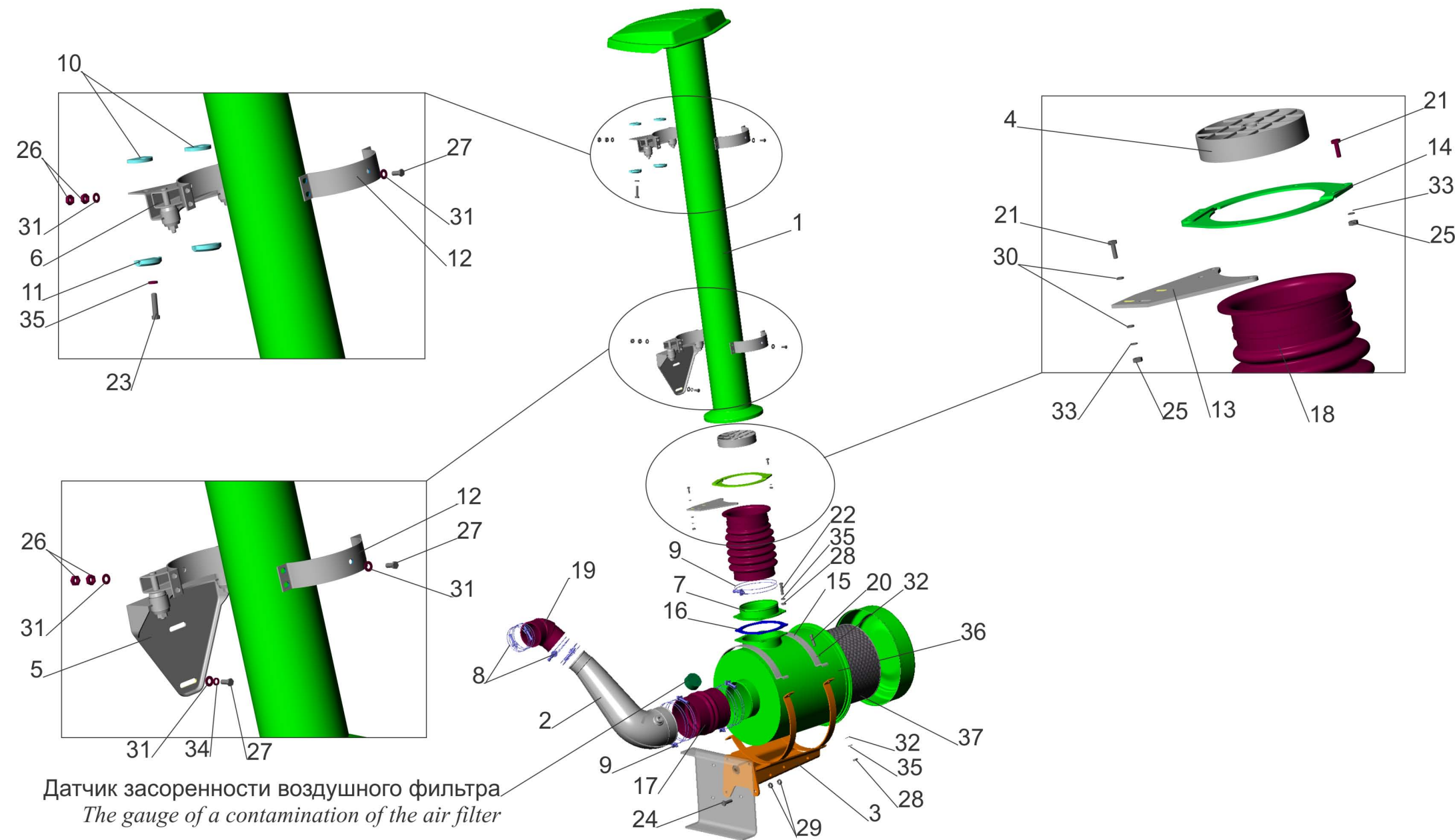
Fig.34 The power supply system air MAZ 543202,543203
