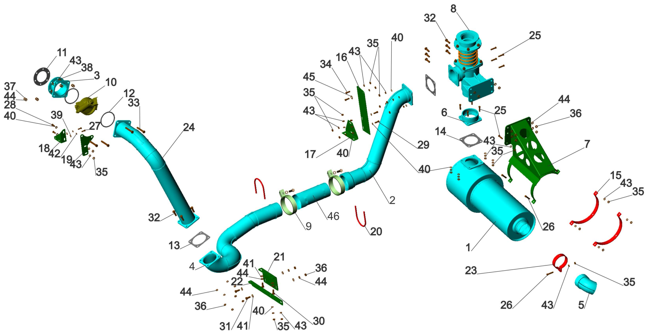
Fig.39 Installation of exhaust system MAZ-551605 with gear box MAZ-543205 and body heating
