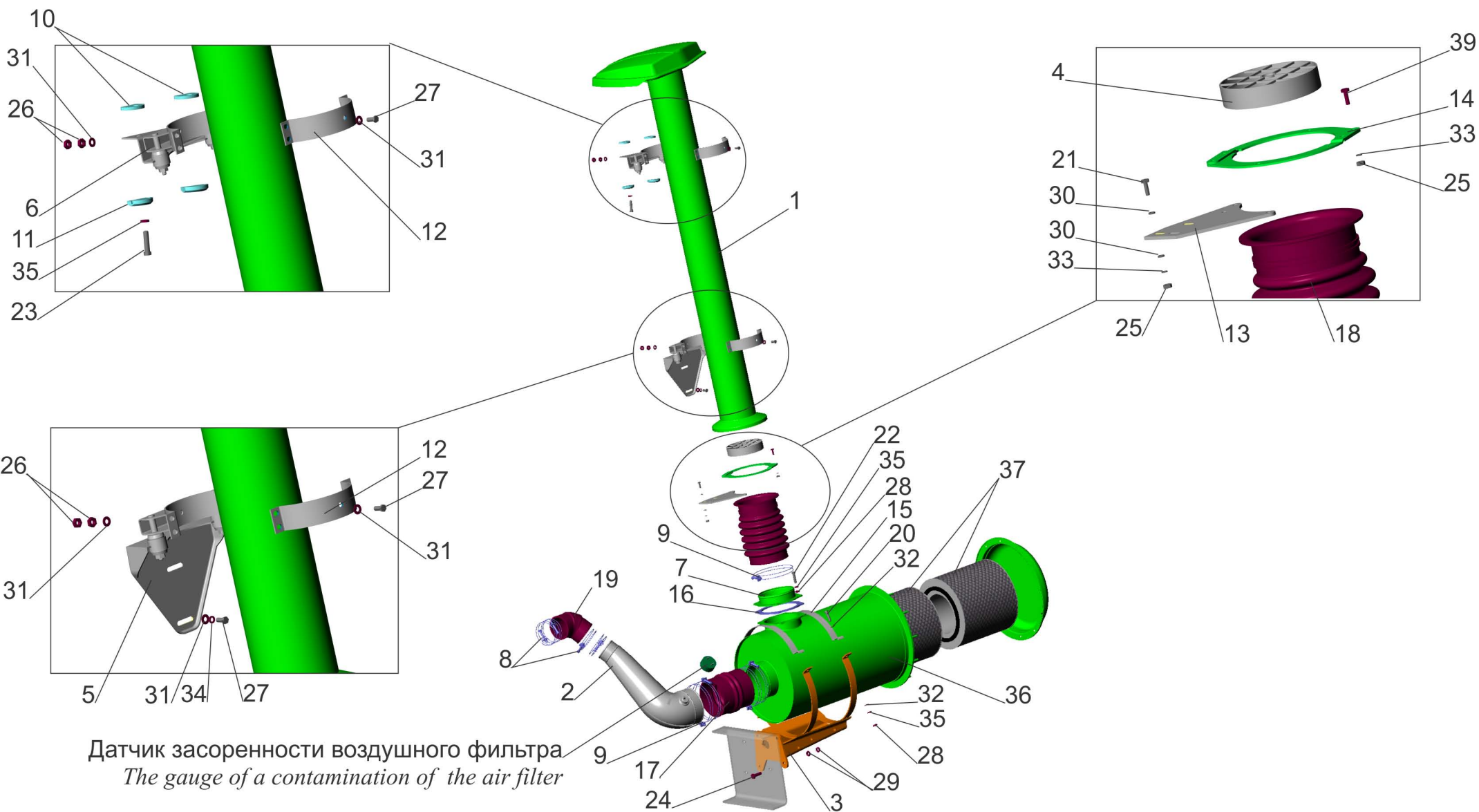
Fig.33 The power supply system air MAZ-642208, 543208, 642205,543205
