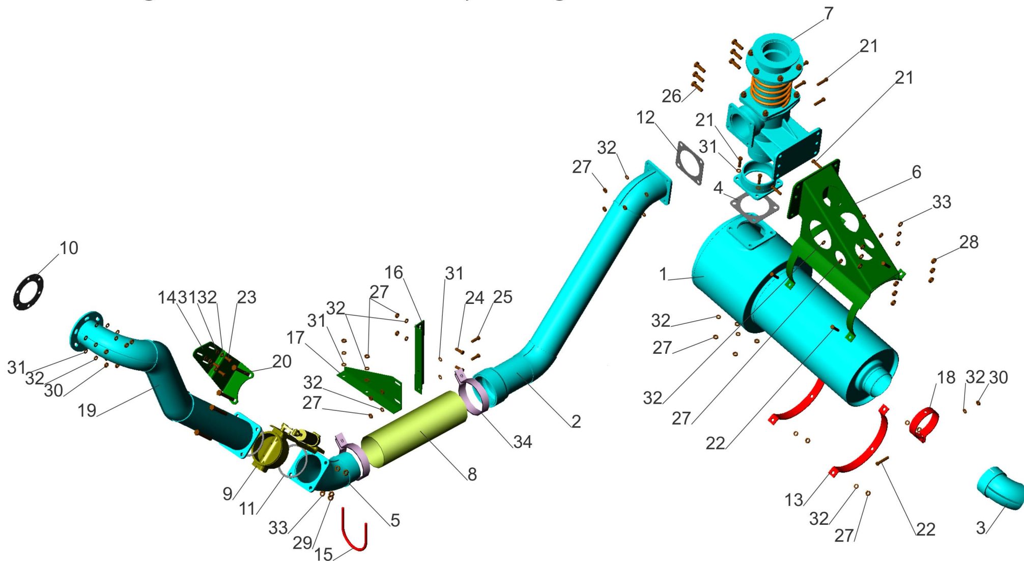
Fig.41 Installation of exhaust system MAZ-551605 with gear box ЯМЗ-238М and body heating
