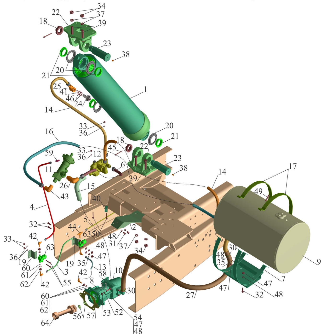
Fig.255 Platform tipping mechanism with back unloading MAZ-551605, 551603
