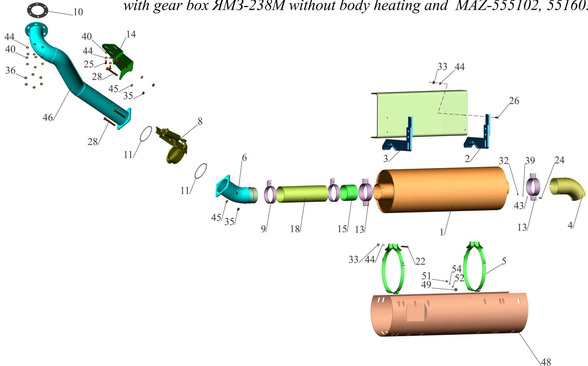
Fig.42 Installation of exhaust system MAZ-551605
