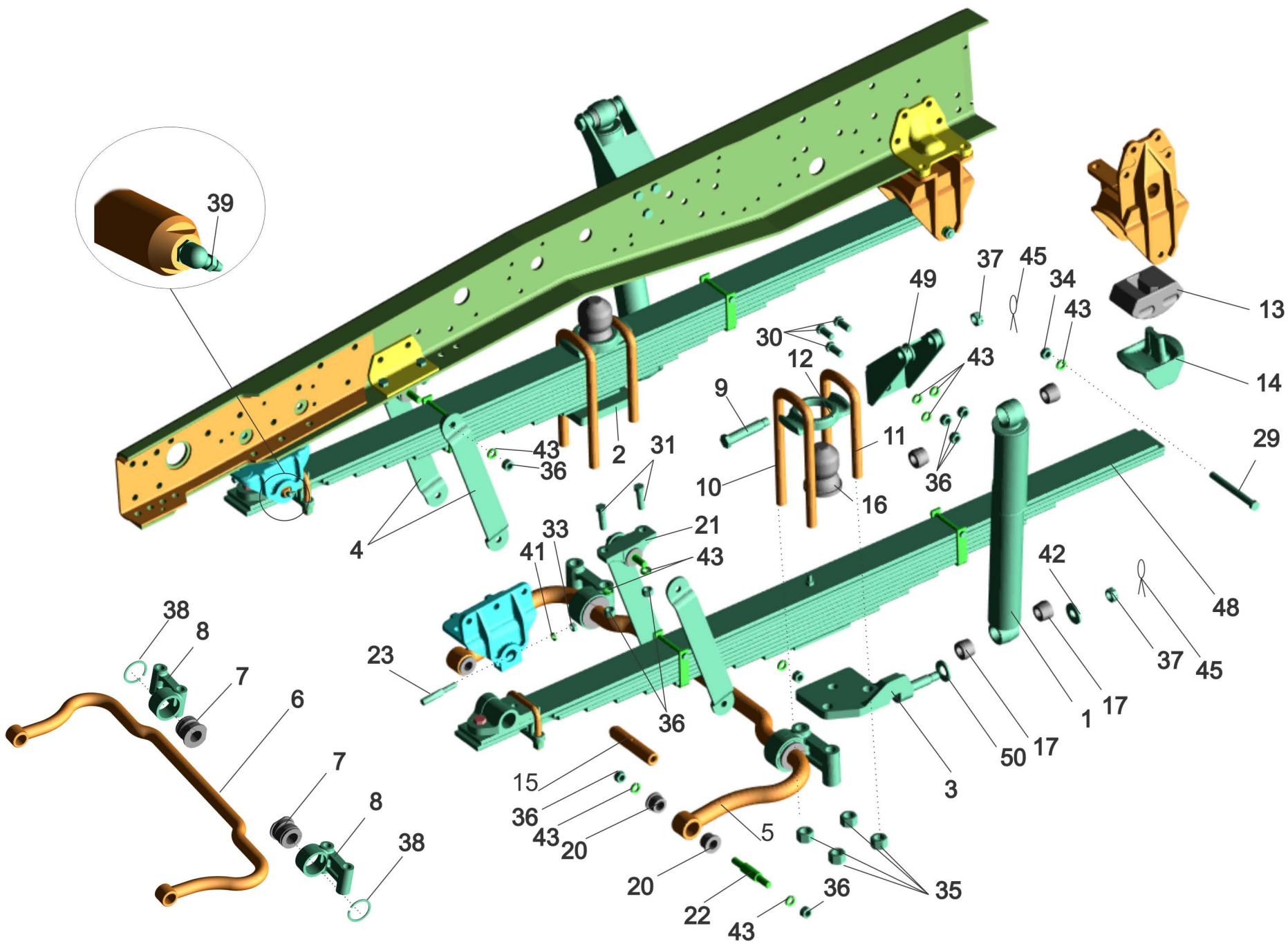
Fig.97 Front suspension 642208-2900001.
