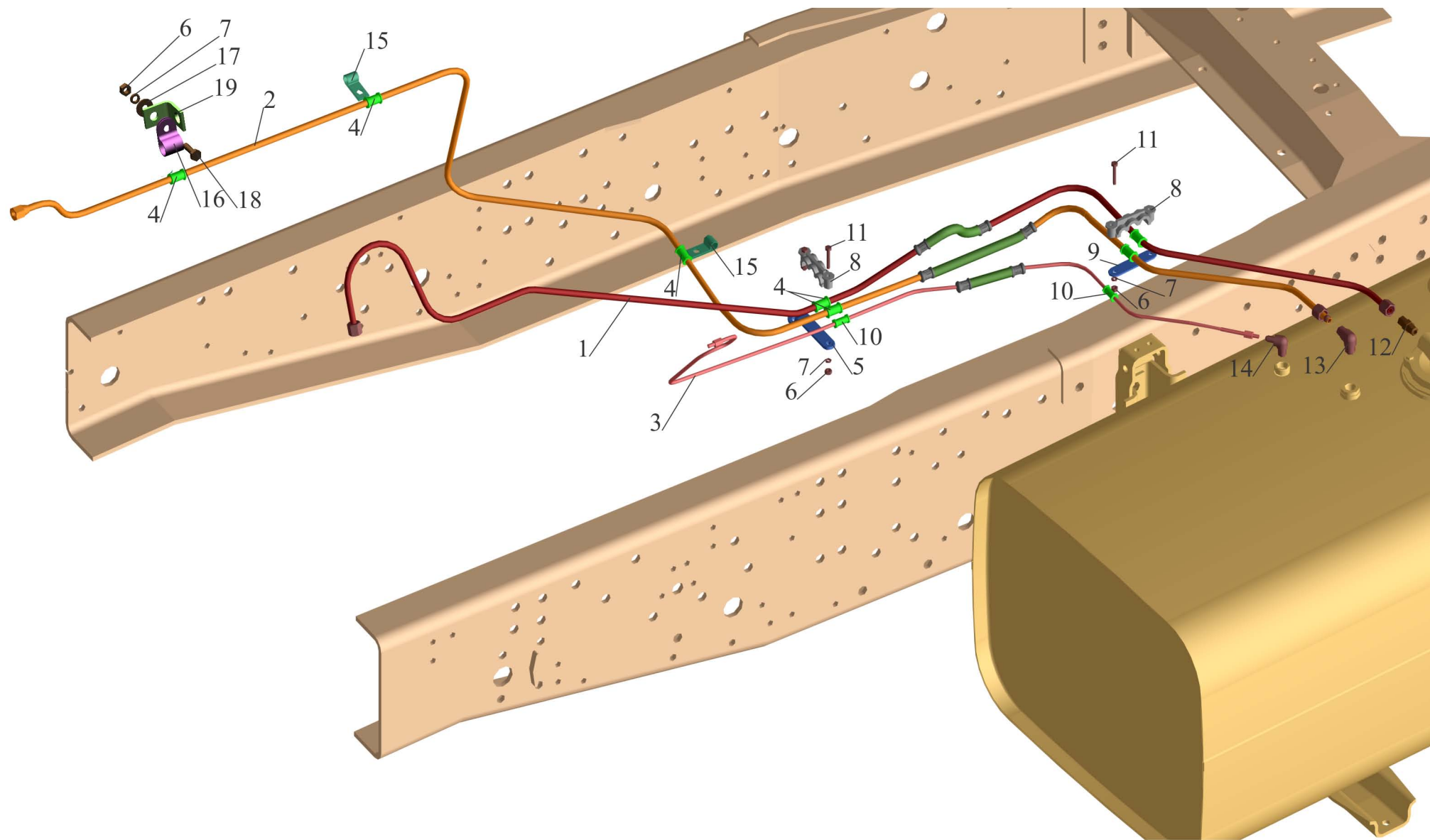
Fig.25 Installation of fuel lines MAZ 551605 (without heater)
