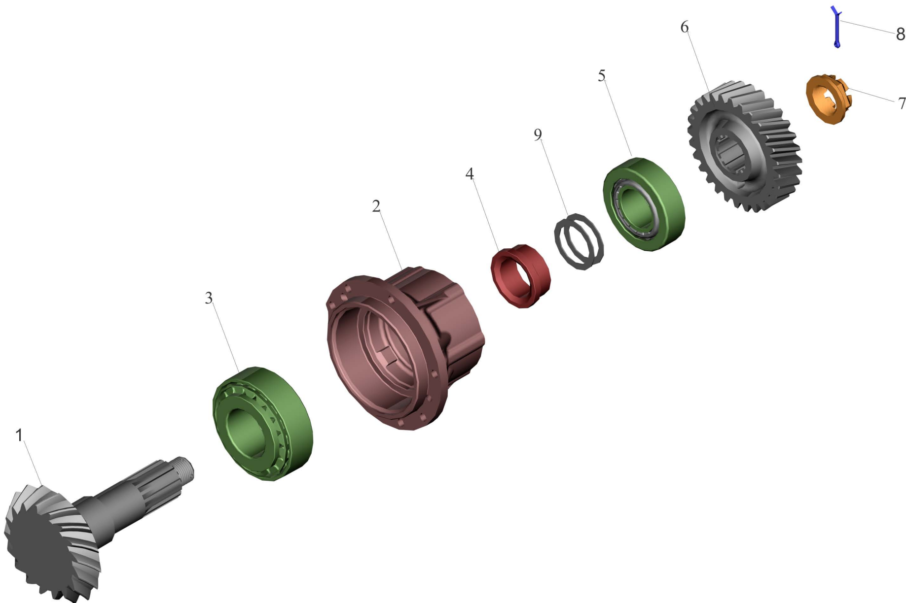
Fig.83 Intermediate axle reduction gear. Drive pinion.
