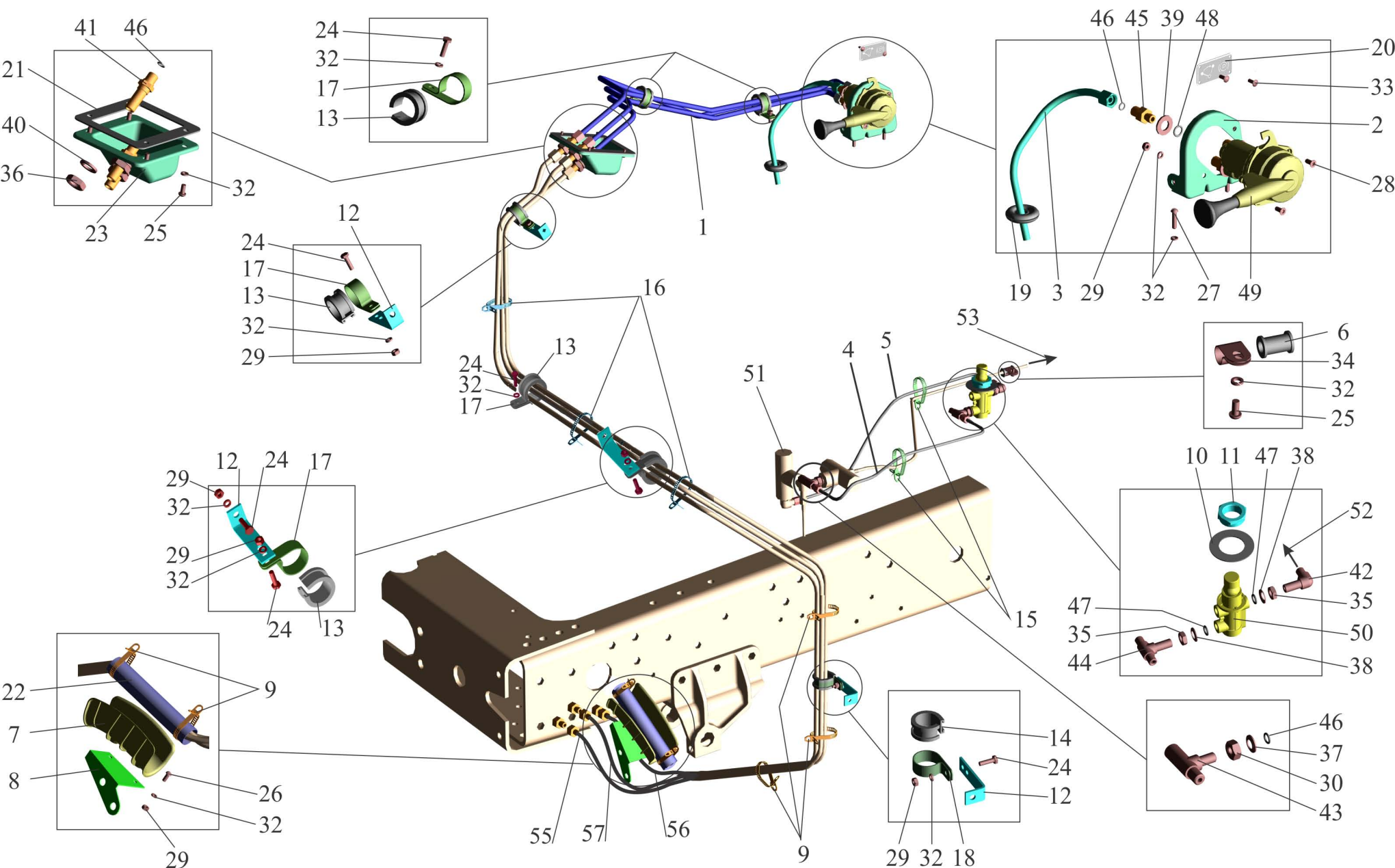
Fig. 187 The parking and secondary braking drive on MAZ-533608, MAZ-533605, MAZ-533603, MAZ-533602, MAZ-630308.
