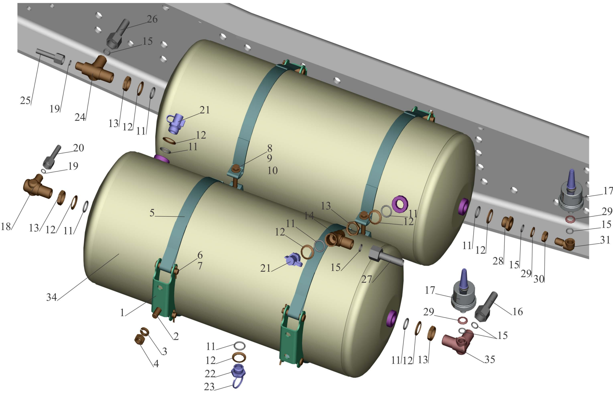
Fig.170 Installation of receivers and attach accessories on MAZ-543208, 543205, 543203, 543202
