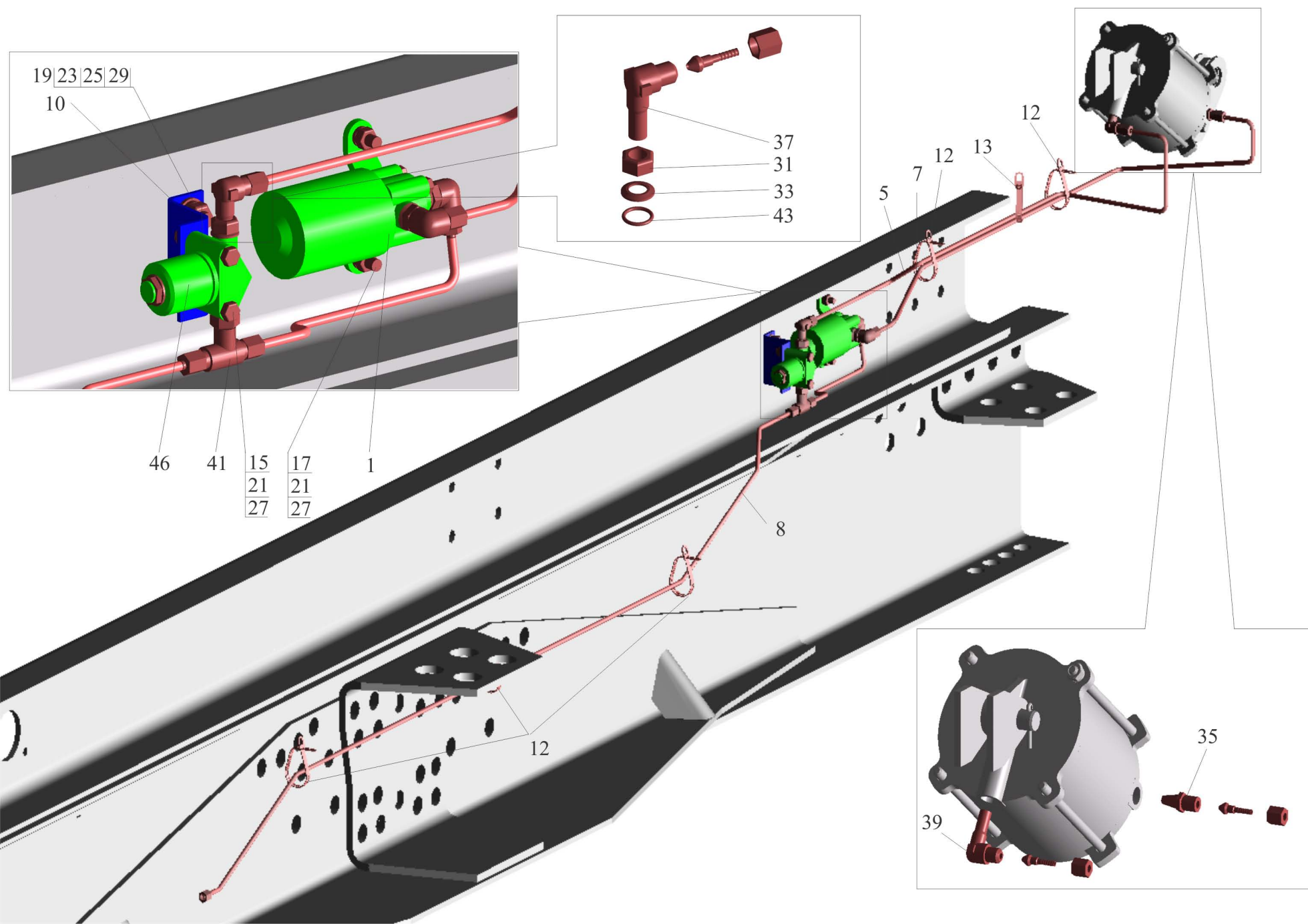
Fig.254 Installation of mechanisms of lock of board MAZ-5516.
