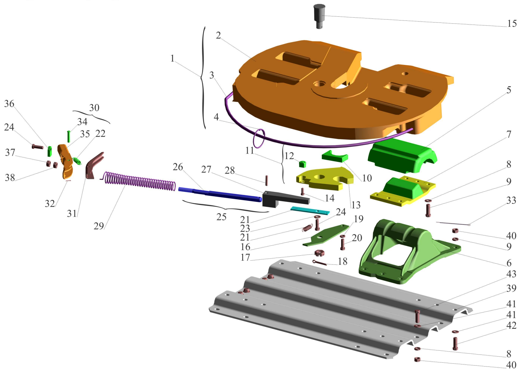
Fig.87 Coupling device.
