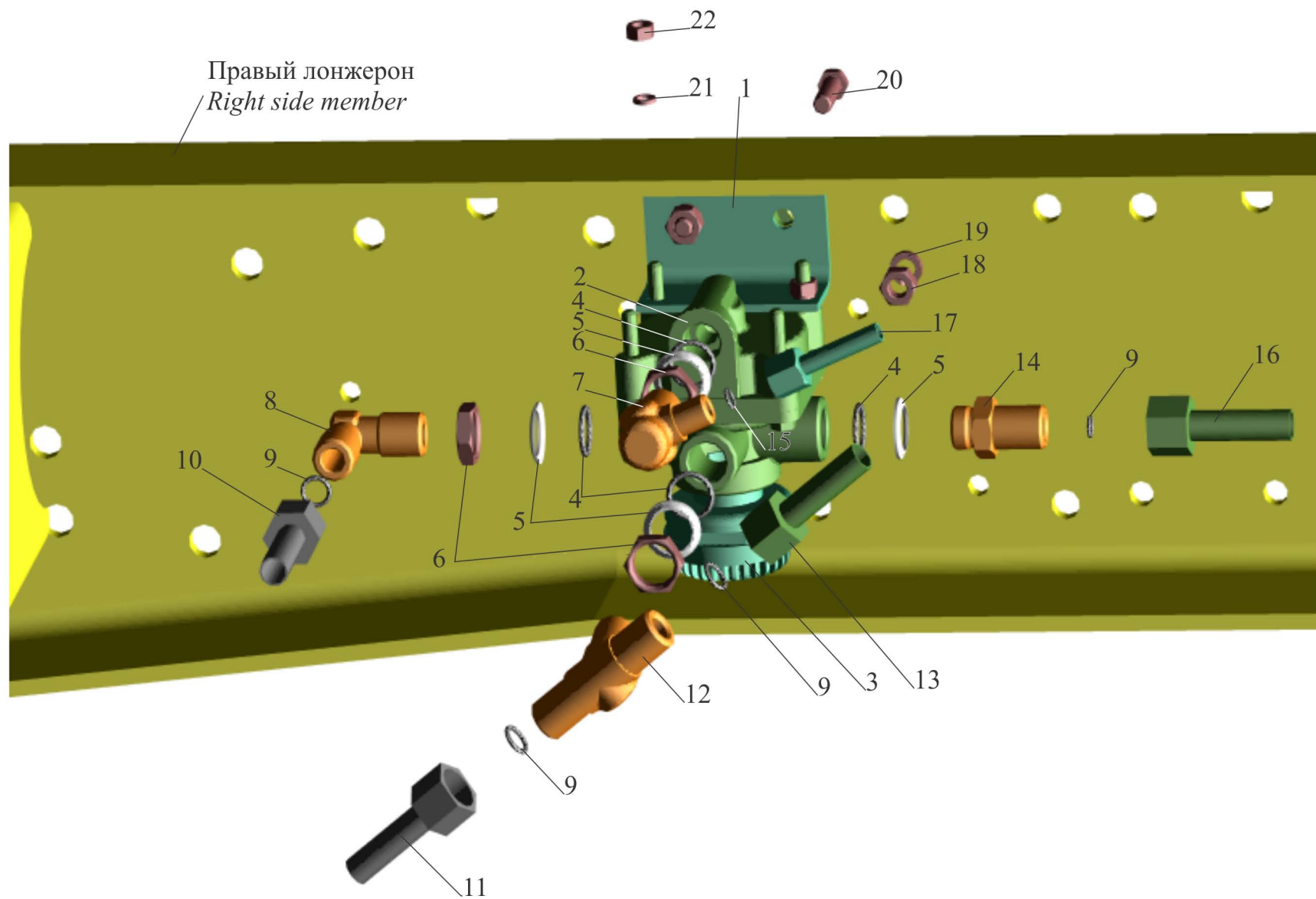
Fig.145 Installation of relay valve and attach accessories MAZ-642208, 642205.
