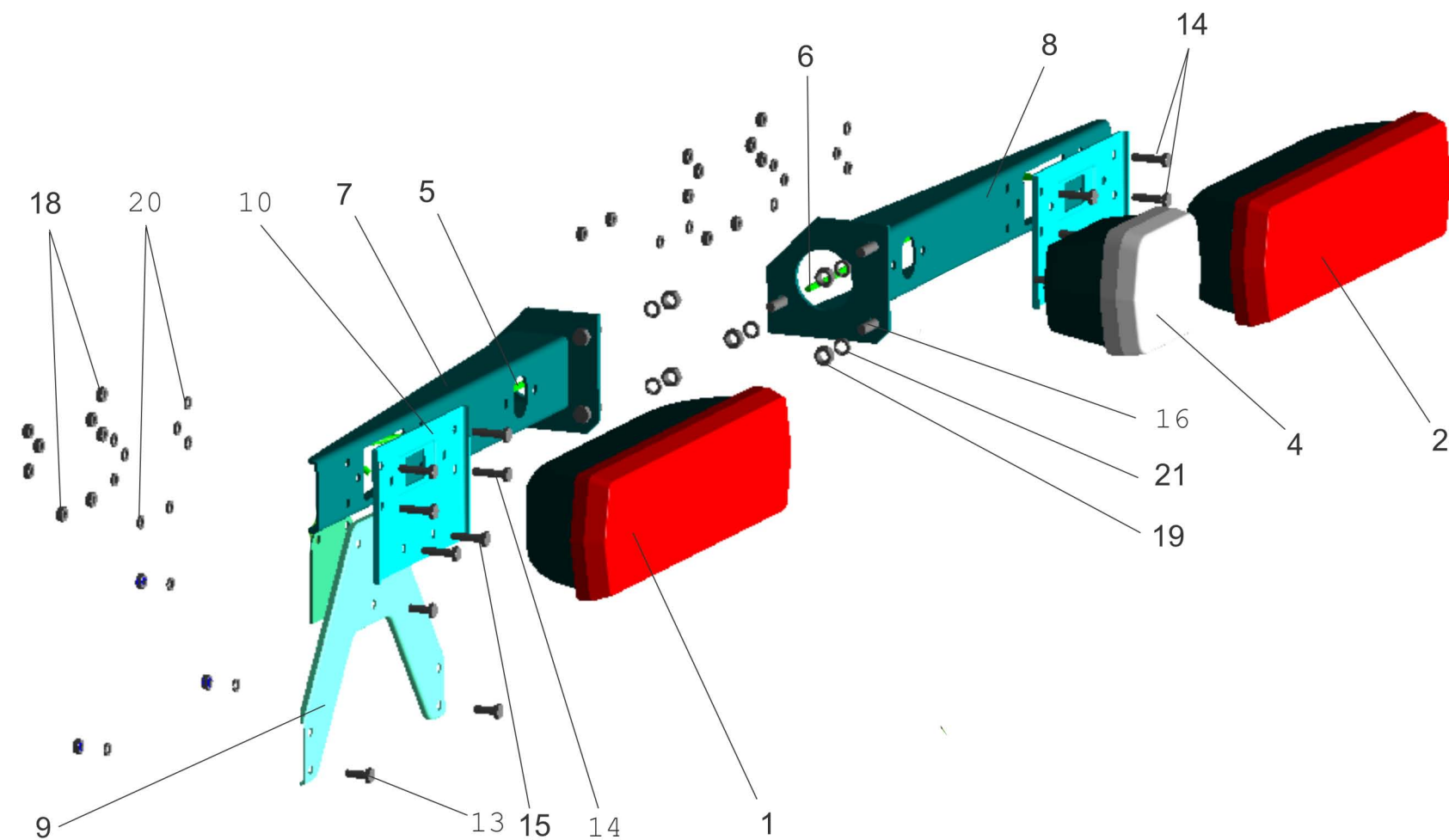
Fig.205 Installation of rear lamps MAZ-555102
