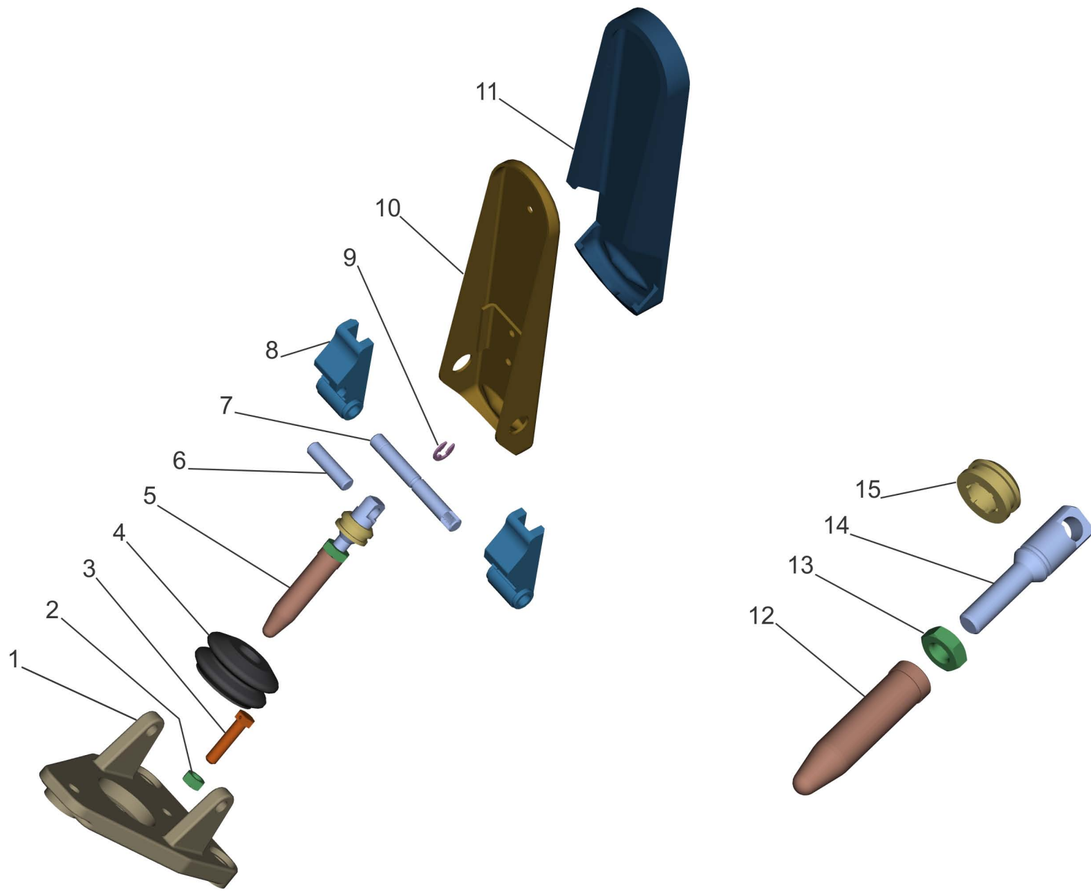
Fig.134 Pedal Brake Valve.
