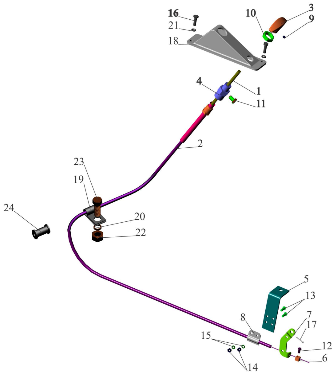
Fig.31 Engine shut-off device
