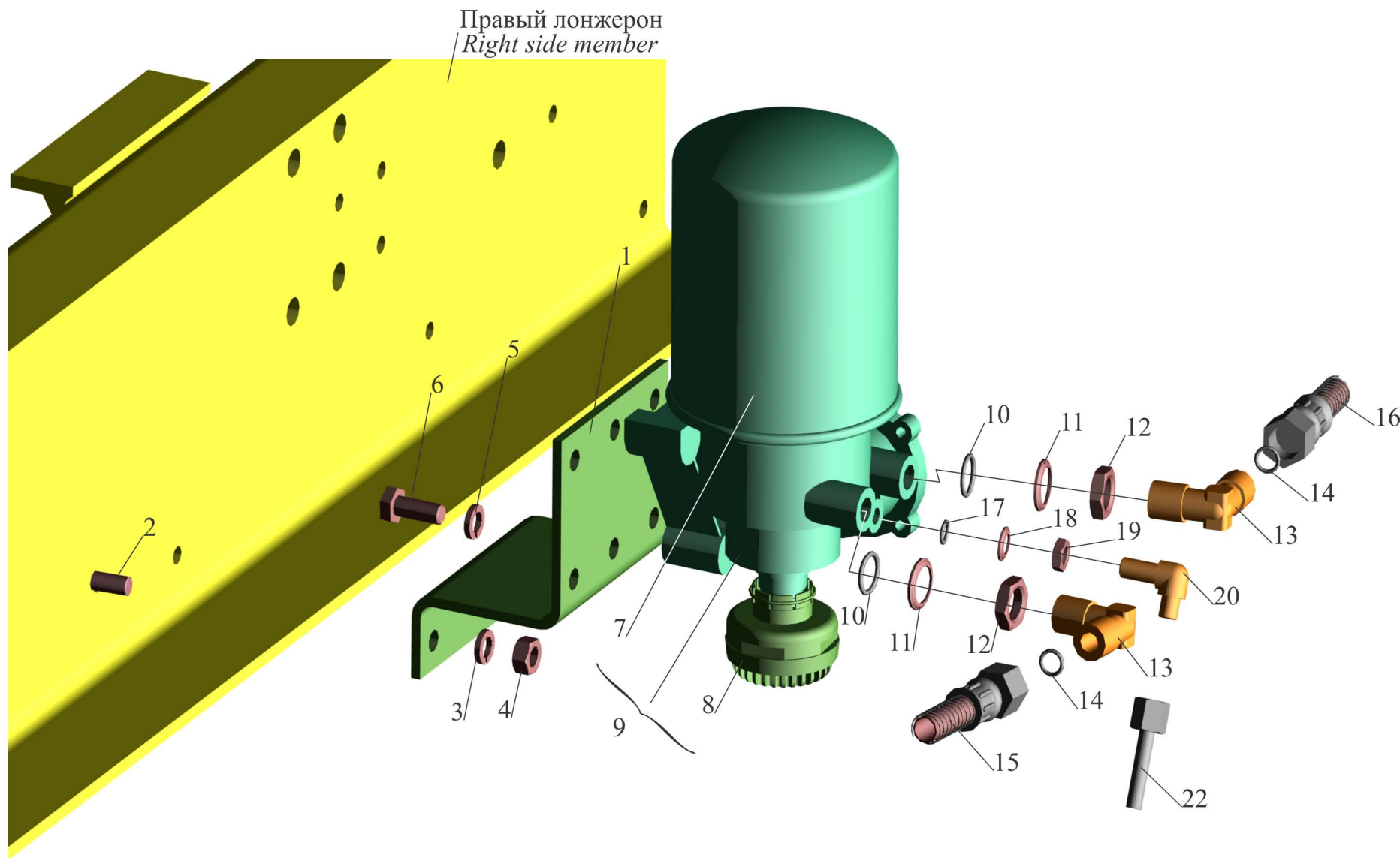
Fig.158 Installation of air dehumidifier and attach accessories MAZ-551605, 551603
