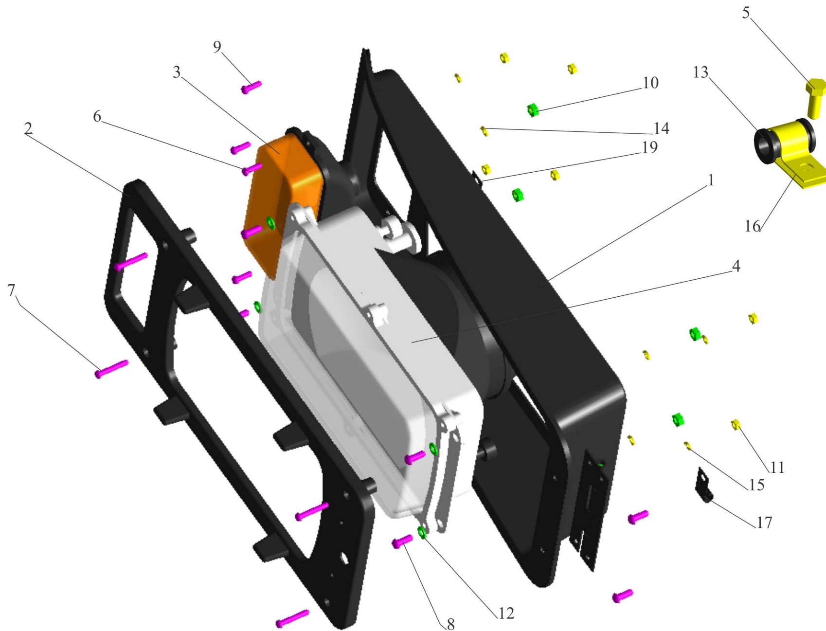
Fig.198 Installing of head lights
