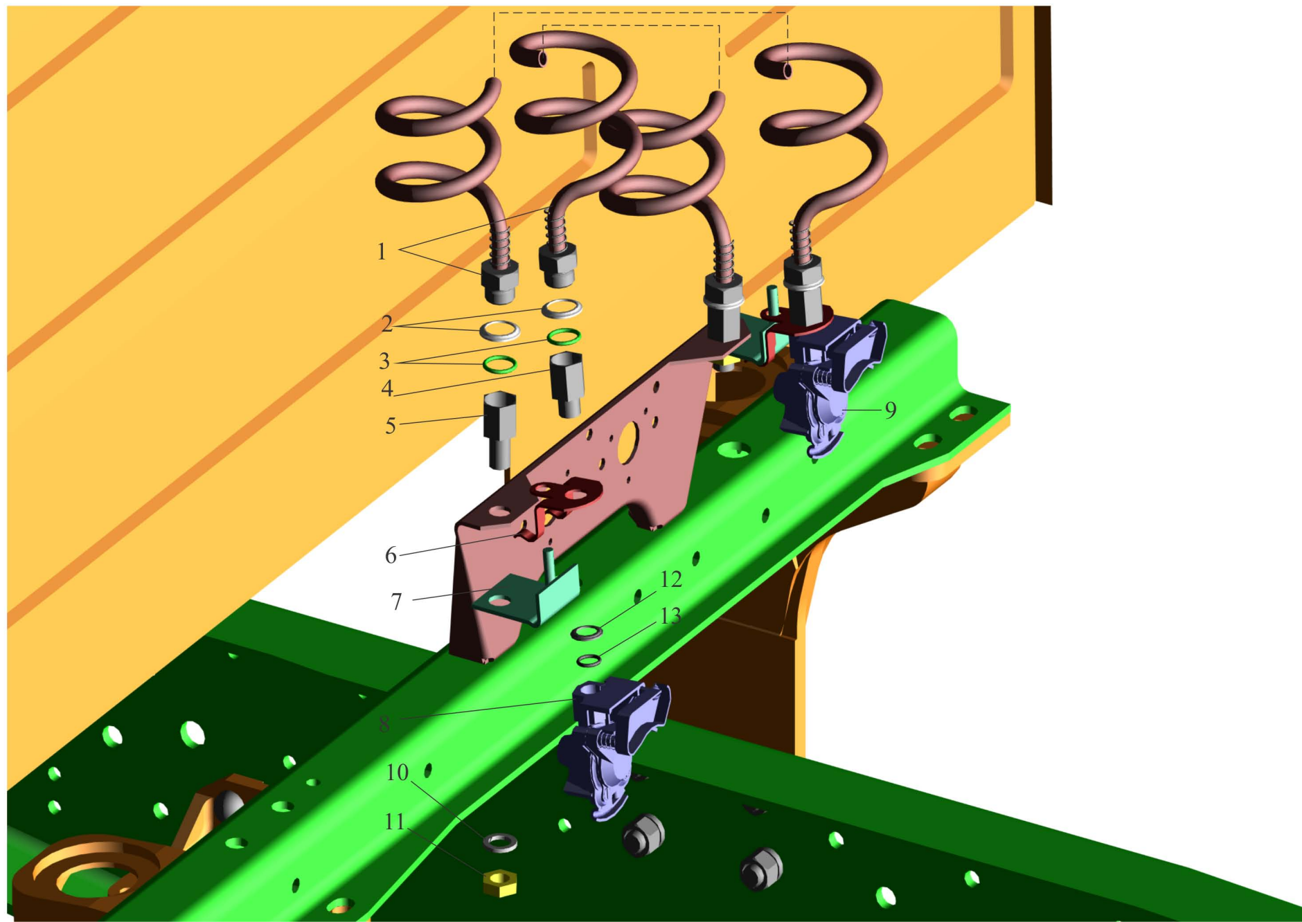
Fig.185 Pneumatic leads on semi-trailer and attach accessories
