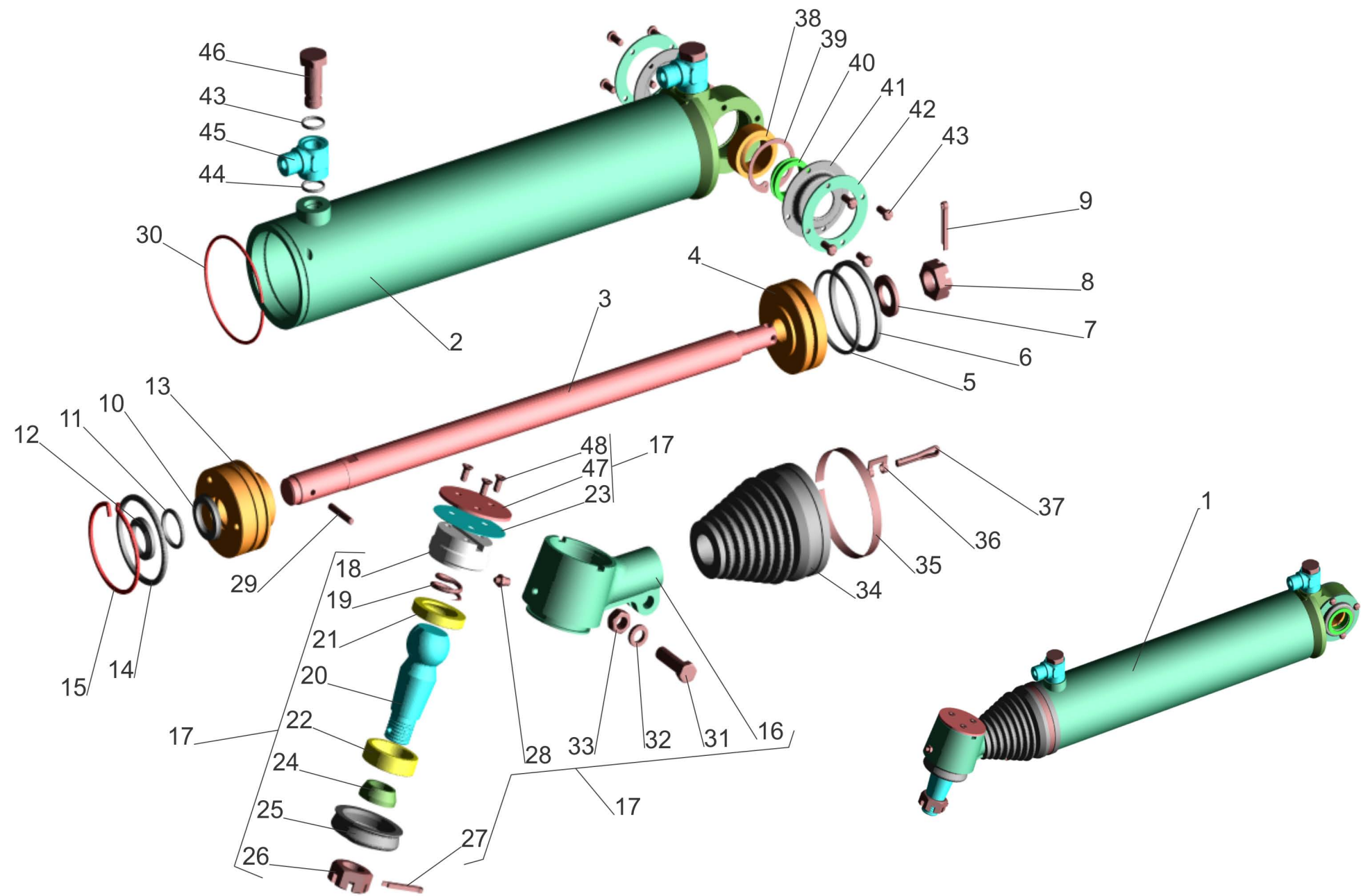
Fig.126 Steering hydraulic booster power cylinder
