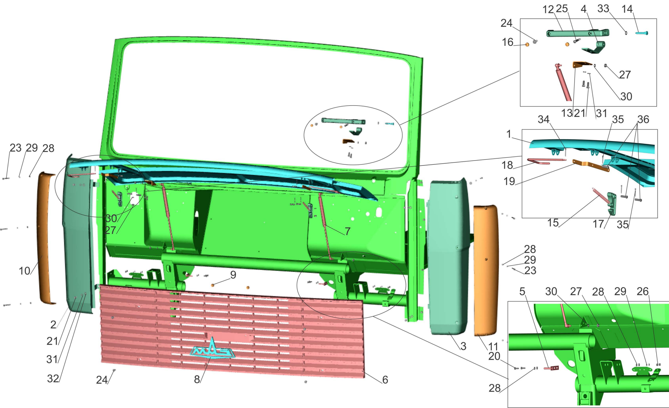
Fig.232 Installation of facing and side flaps
